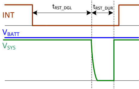
Figure 6: System Reset Function Operation Profile
