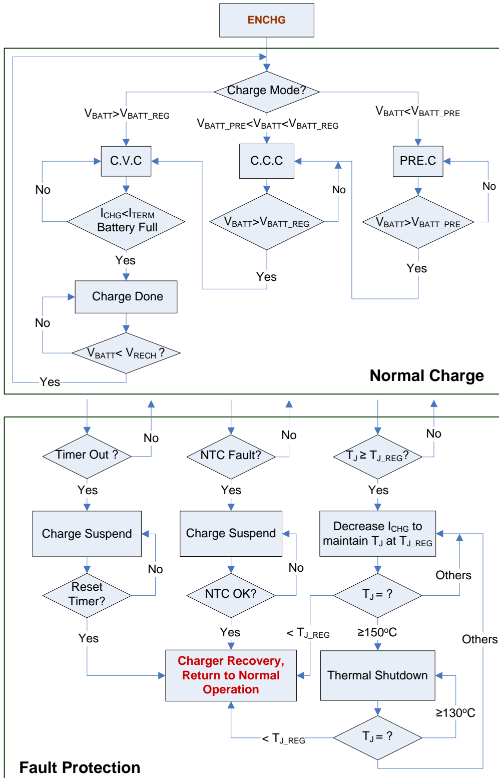
Figure 16: Charging Process
