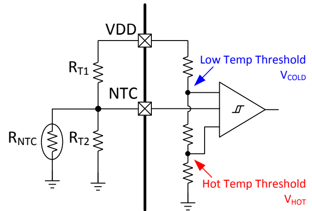
Figure 18: NTC Function Block
