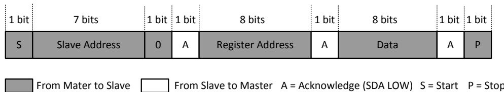
Figure 11: Single Write
