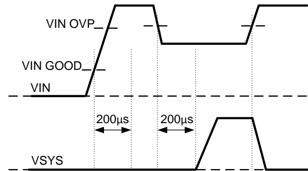
Figure 3: Input Power Detection Operation Profile
