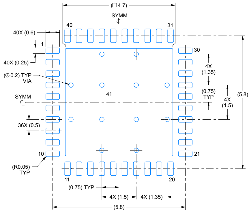
LAND PATTERN EXAMPLE SCALE:12X
