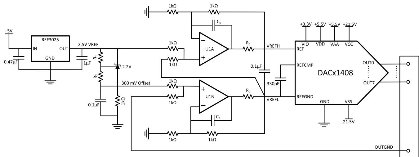
Figure 67. Schematic for Remote Ground Tracking
