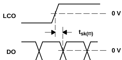
Figure 11. LCO to DO Multiple-Frequency Skew Waveforms
