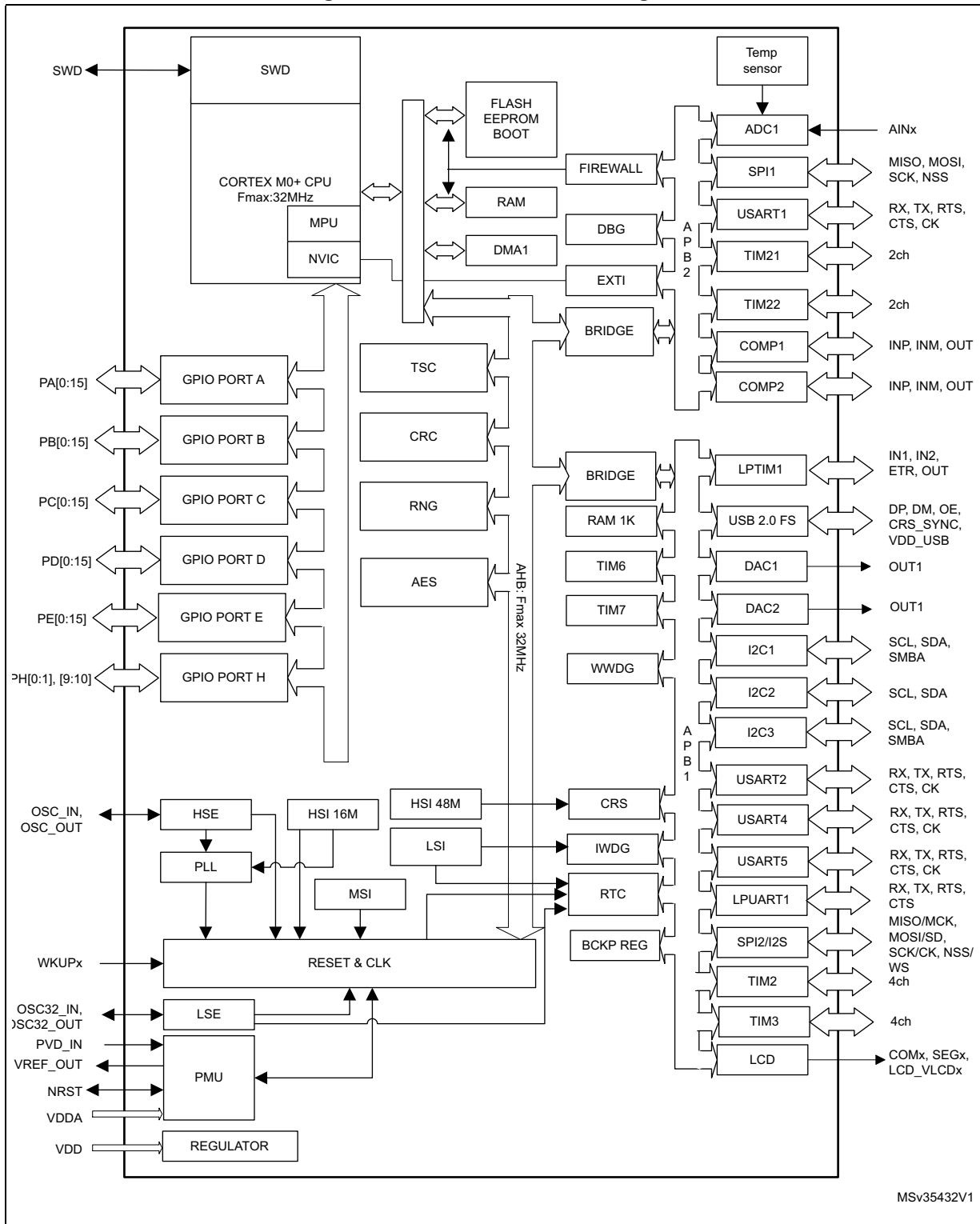
Figure 1. STM32L083xx block diagram
