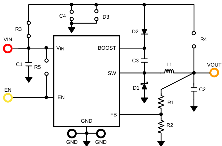
Figure 3. LMR12010Y Demo Board Schematic
