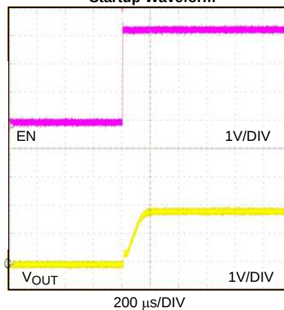
Startup Waveform
