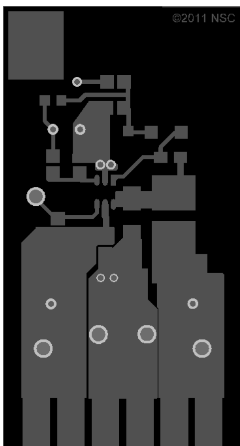
Figure 4. Top Layer
