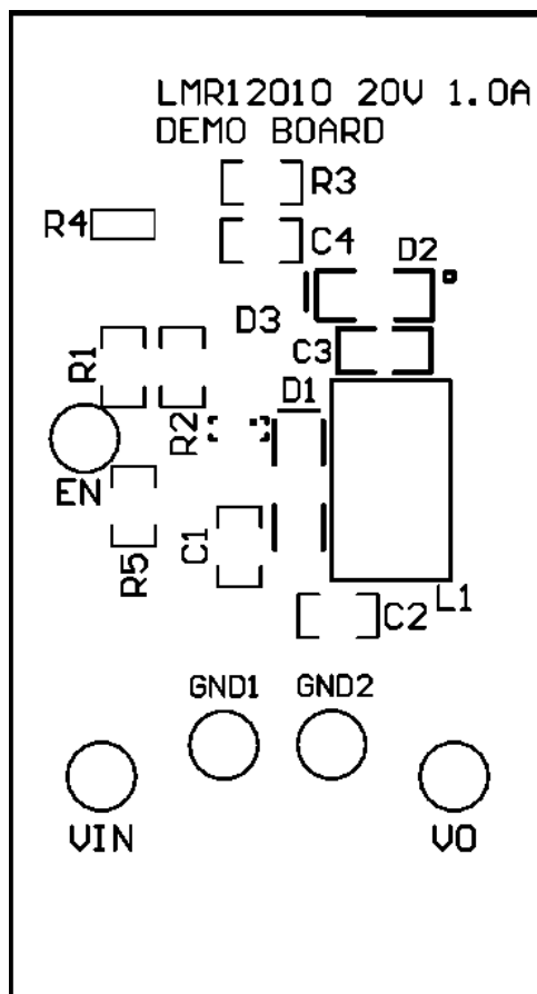
Figure 5. Top Overlay
