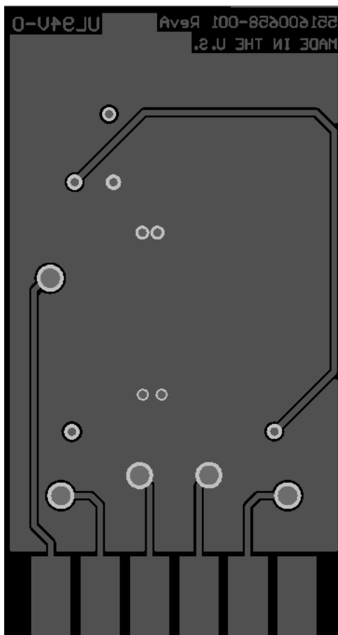
Figure 8. Bottom Layer
