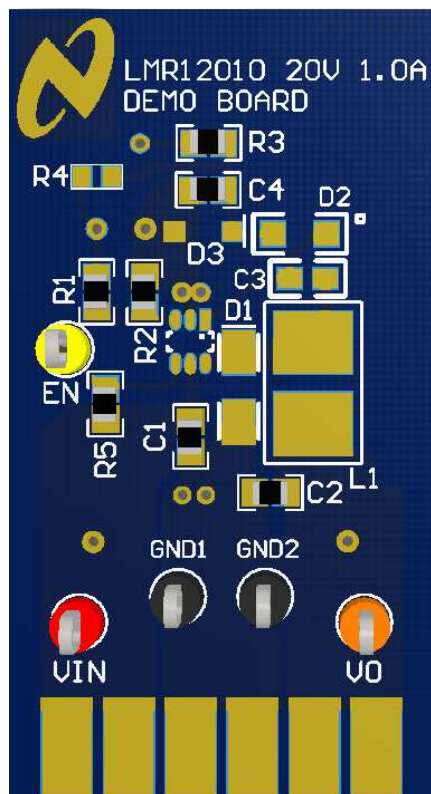
Figure 1. LMR12010 Demo Board Top View
