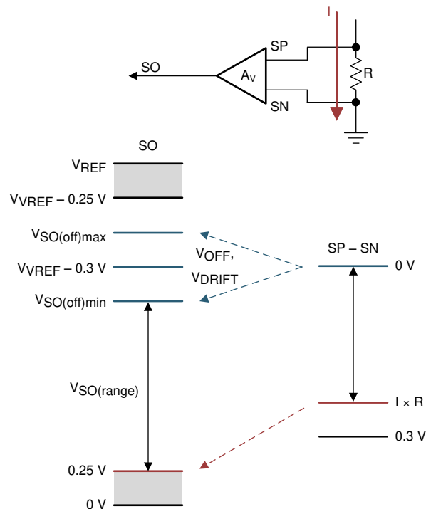
Figure 35. Unidirectional Current-Sense Regions
