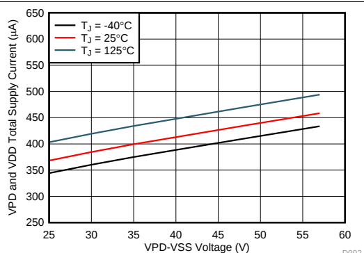
Figure 6. VPD and VDD Supply Current vs Voltage
