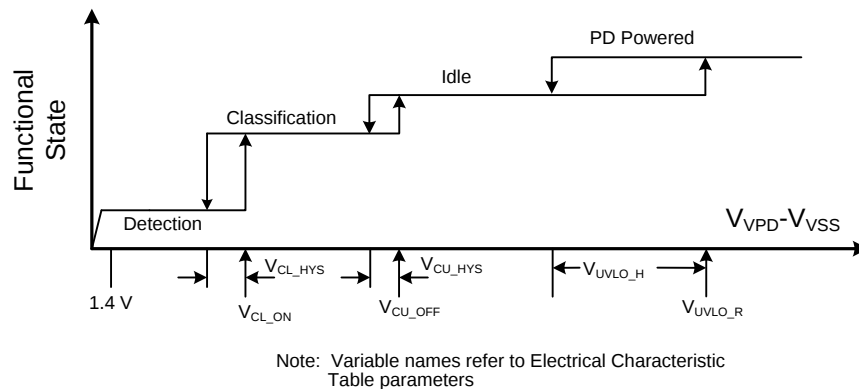
Figure 28. Threshold Voltages
