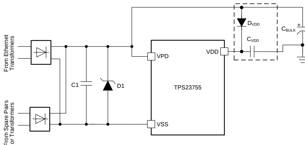
Figure 35. DVDD and CVDD Configuration for Low Temperature Conditions
