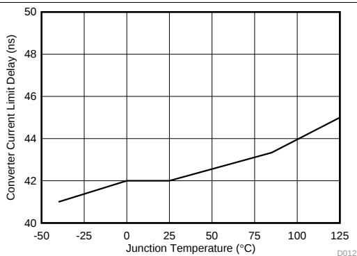
Figure 18. Converter Current Limit Delay vs Temperature
