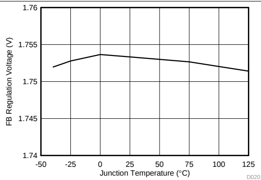
Figure 14. Feedback Regulation Voltage vs Temperature
