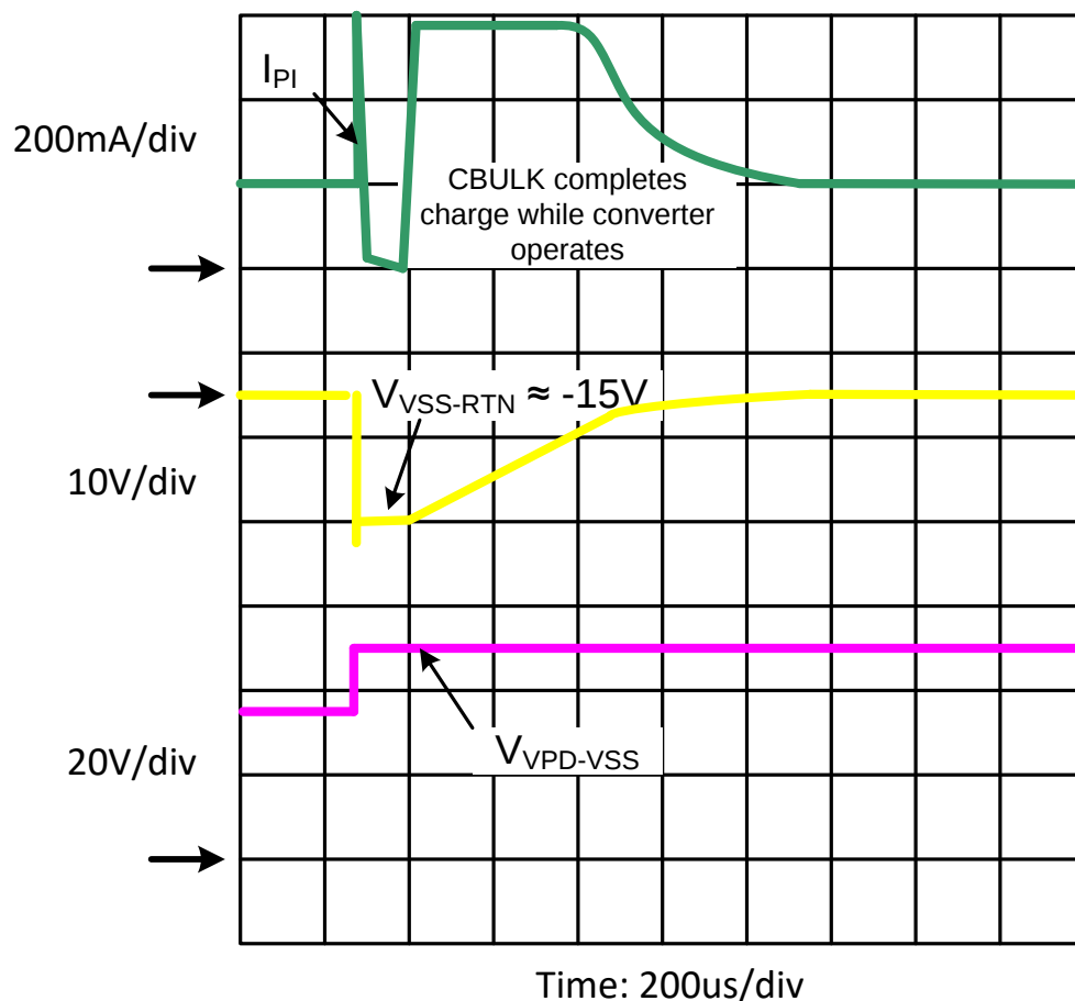
Figure 32. Response to PSE Step Voltage
