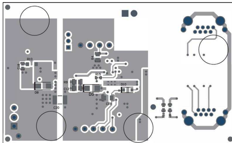
Figure 45. Bottom Side Placement and Routing
