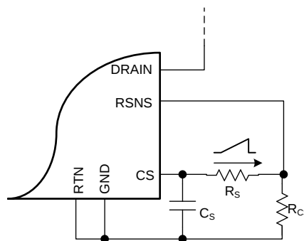
Figure 25. Additional Slope Compensation
