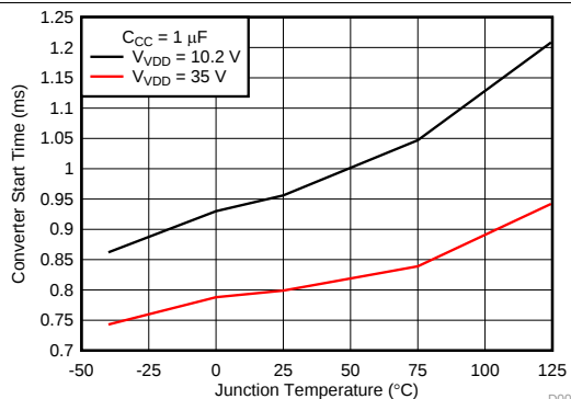
Figure 7. Converter Startup Time vs Temperature
