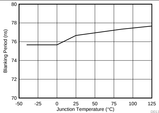
Figure 16. Blanking Period vs Temperature
