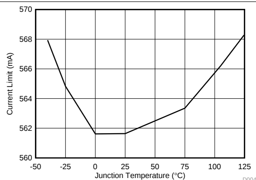
Figure 3. PoE Current Limit vs Temperature
