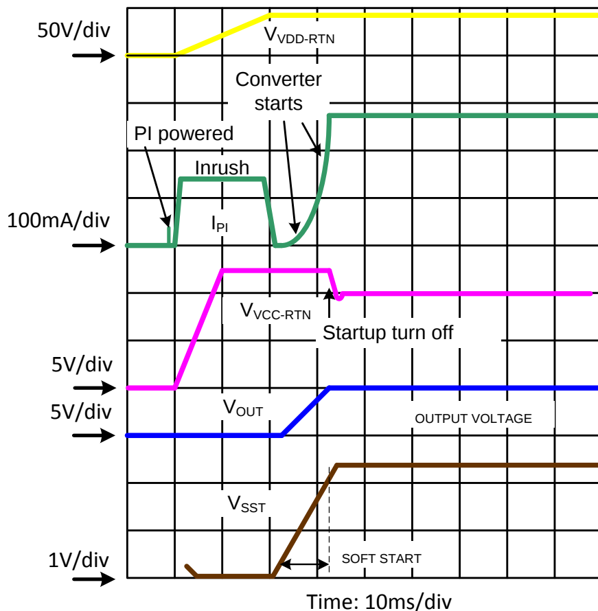
Figure 30. Power Up and Start
