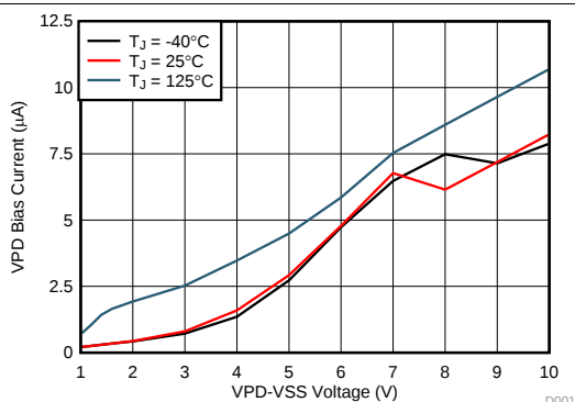
Figure 2. Detection Bias Current vs Voltage
