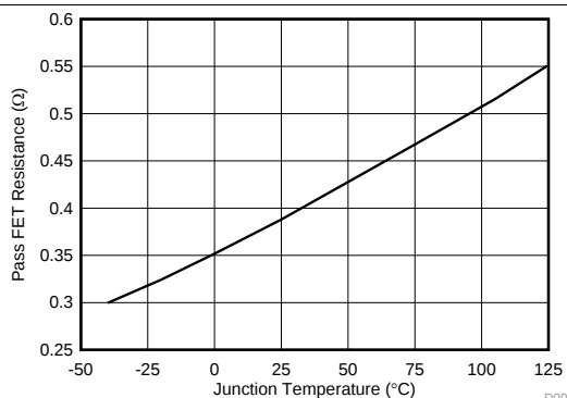
Figure 5. Pass FET Resistance vs Temperature
