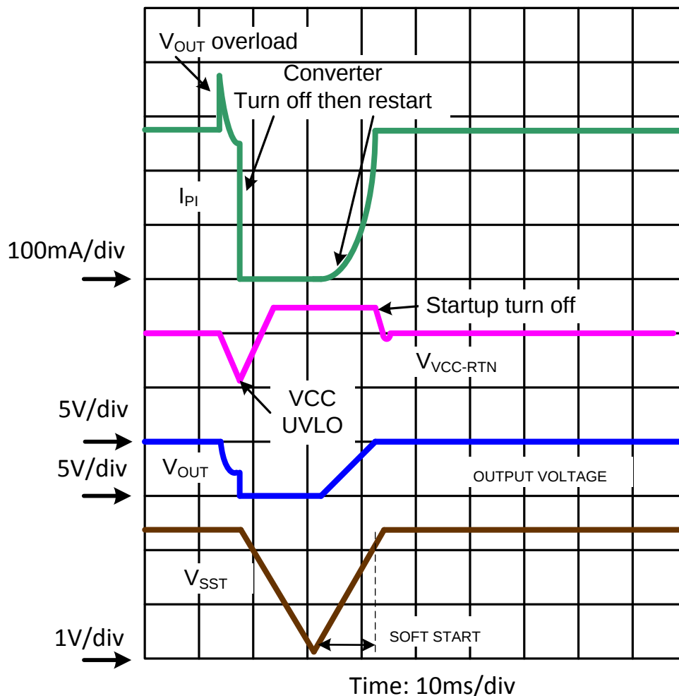
Figure 31. Restart Following Severe Overload at Main Output of Flyback DC-DC Converter
