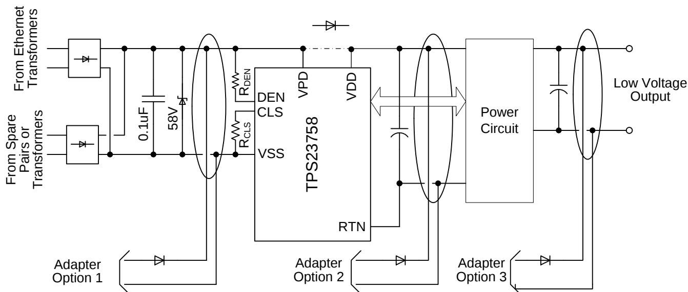
Figure 33. ORing Configurations
