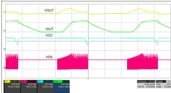
Figure 38. TPS23758 Output Short and Recovery
