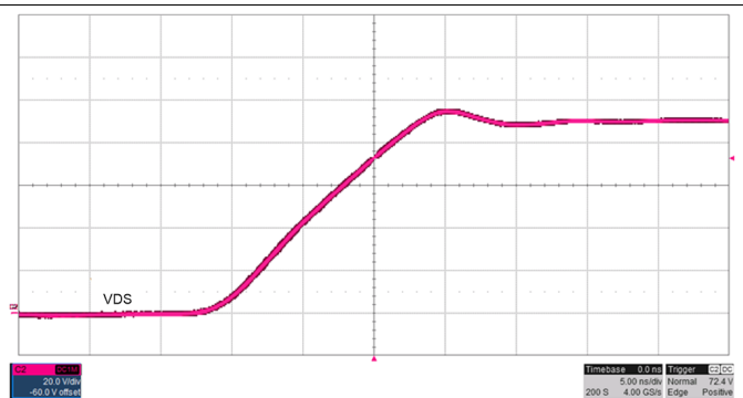
Figure 39. Slew Rate Adjust SRR = 10 \Omega
