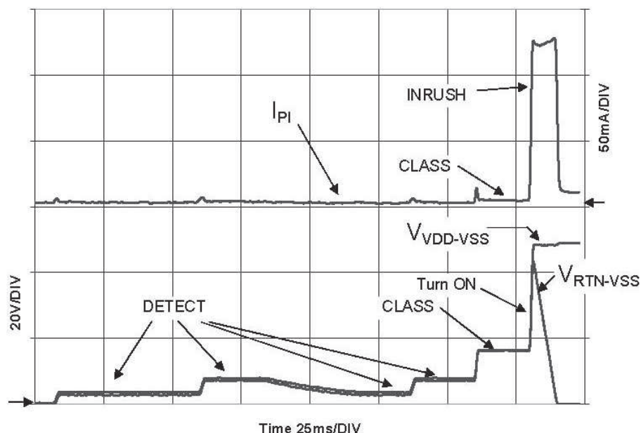
Figure 29. PoE Start-Up Sequence
