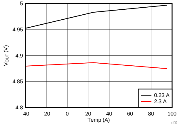
Figure 42. Output Regulation vs. Ambient Temperature
