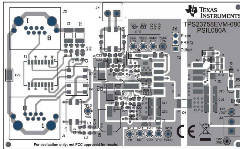
Figure 44. Top Side and Routing
