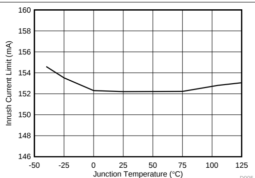
Figure 4. PoE Inrush Current Limit vs Temperature
