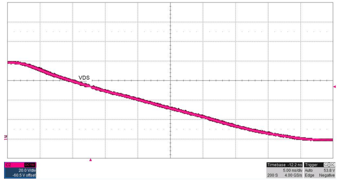
Figure 43. Slew Rate Adjust SRF = 100 Ω
