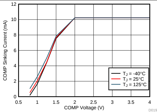
Figure 20. Error Amplifier Sink Current
