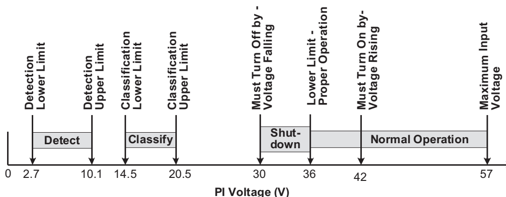
Figure 27. Operational States
