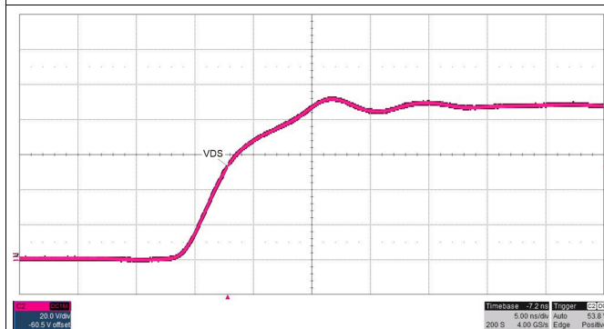
Figure 40. Slew Rate Adjust SRR = 0 \Omega
