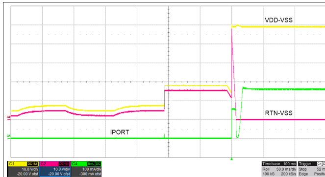
Figure 36. TPS23758 Startup to TPS23880 PSE
