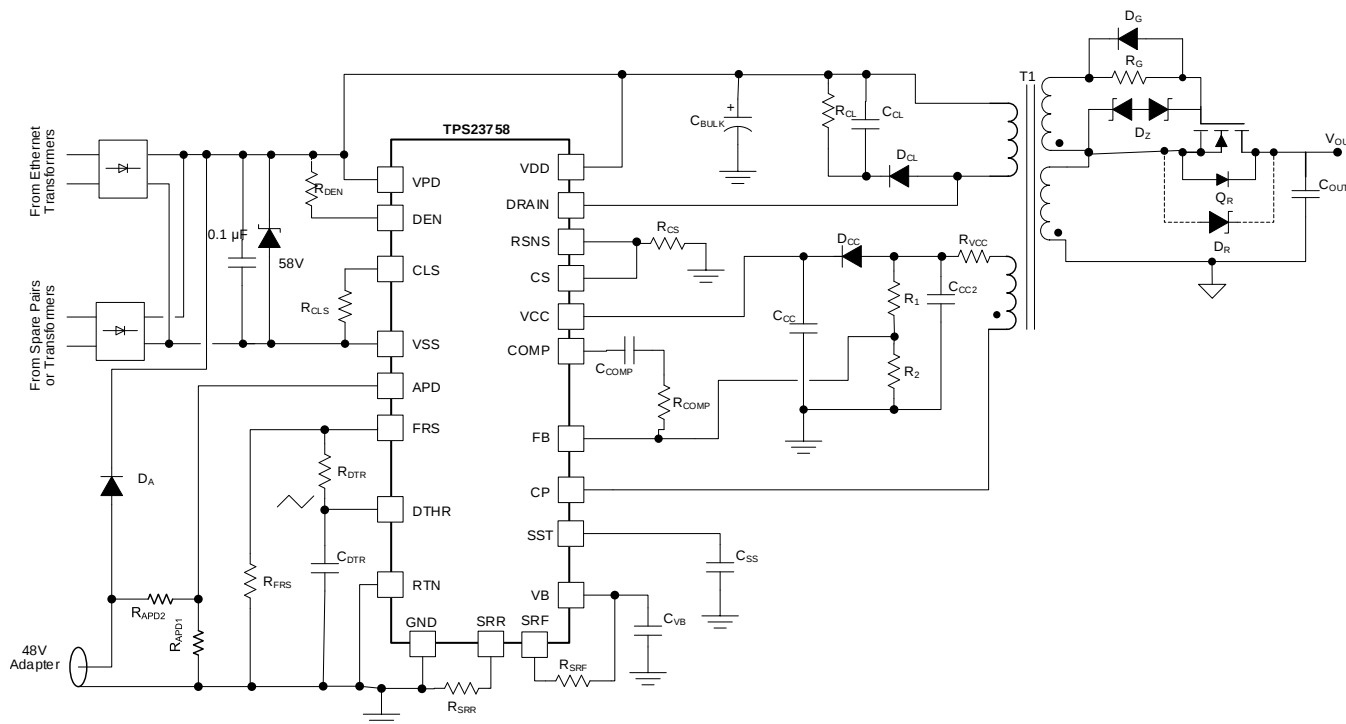
Figure 34. Basic TPS23758 Implementation
