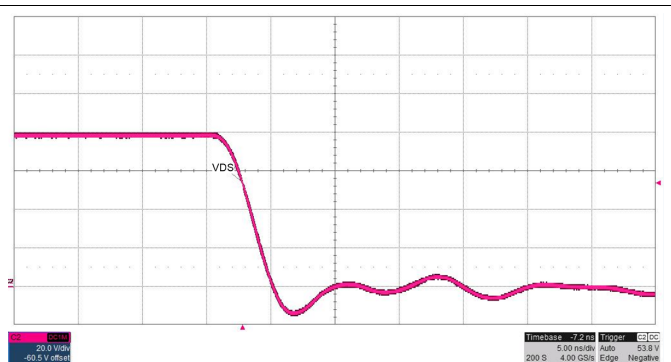
Figure 41. Slew Rate Adjust SRF = 0 \Omega
