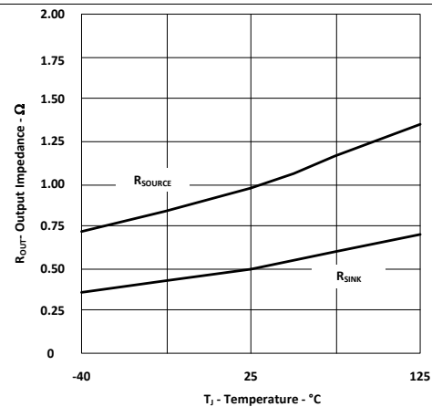
Figure 7. LGATE DC Output Impedance vs Temperature
