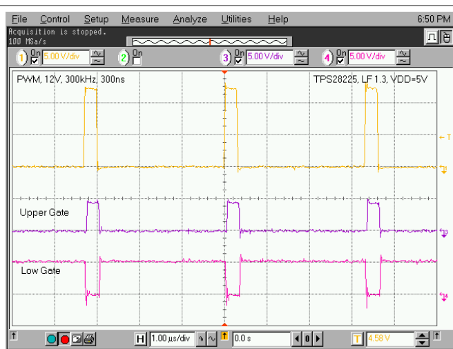
Figure 24. 12-V PWM Pulse at V_{DD} = 5 V
