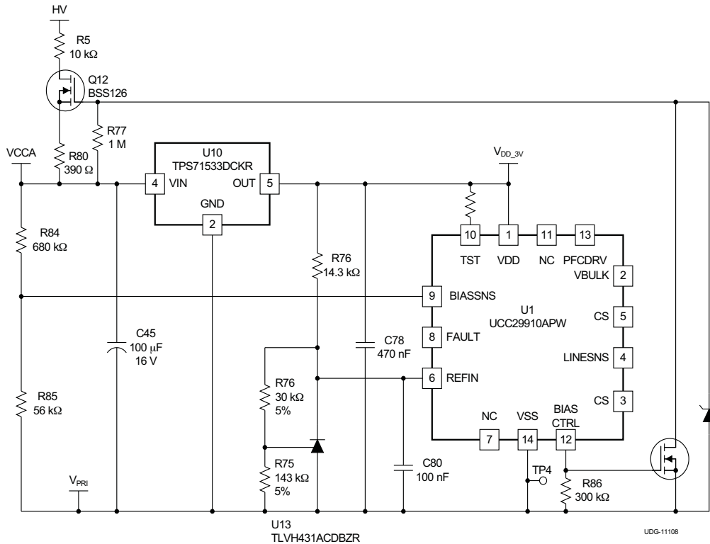
Figure 5. Simplified Schematic
