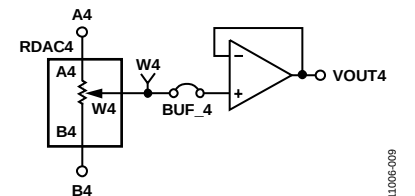
Figure 9. RDAC4
