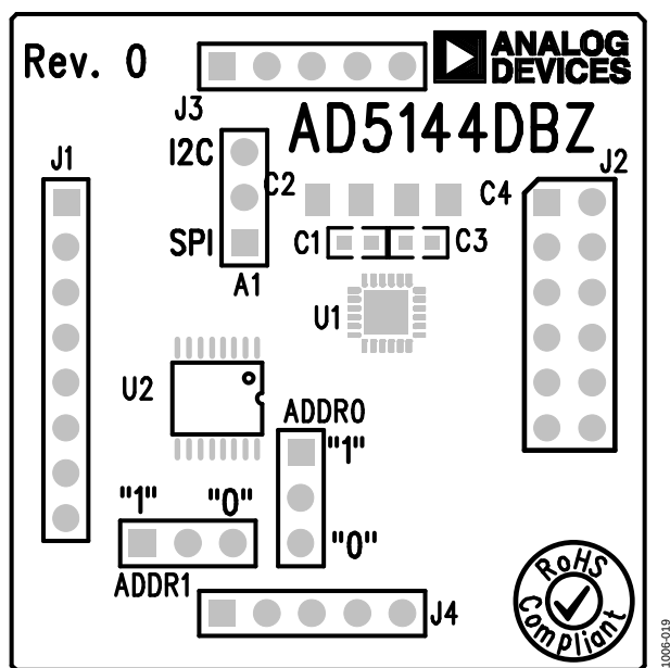
Figure 20. Component Side View of Daughter Board
