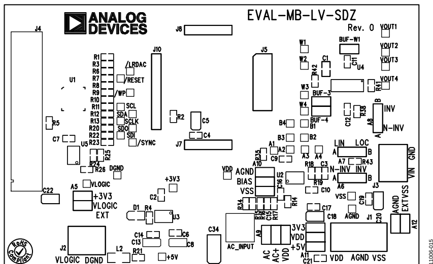
Figure 16. Component Side View of Motherboard
