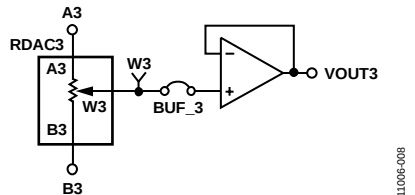
Figure 8. RDAC3
