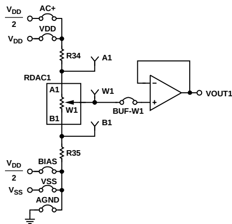
Figure 2. DAC
