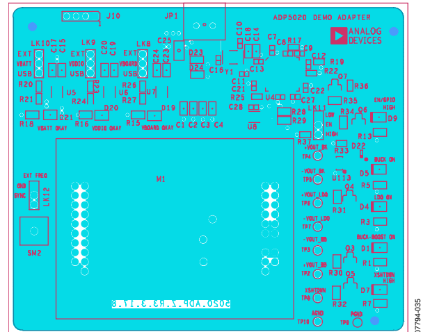
Figure 35. Bottom Layer
