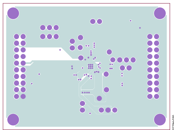
Figure 30. Inner Layer 2
