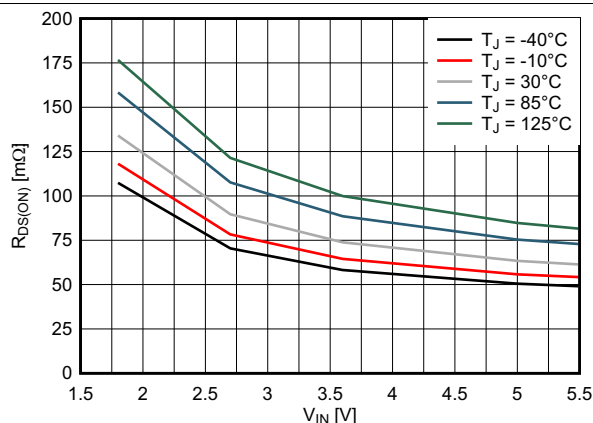
Figure 6. Low Side Switch Drain Source Resistance R_{DS(ON)}
