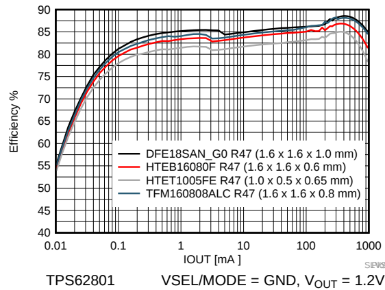
Figure 18. Inductor Comparison
