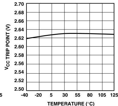
V CC Trip Point vs. Temperature (°C)
