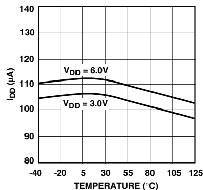
I DD vs. Temperature (SELECT = NC)
