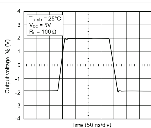
Figure 8. Large signal follower response
