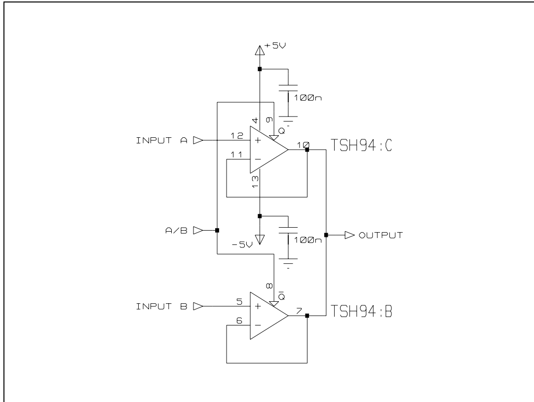
Figure 18. Signal multiplexing
