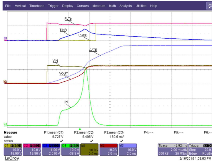
Figure 2. Start Up (COUT (on EVM + External) = 5500 \mu F)
