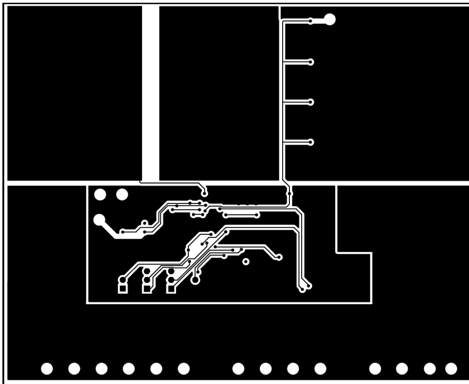
Figure 13. Midlayer 1 Routing
