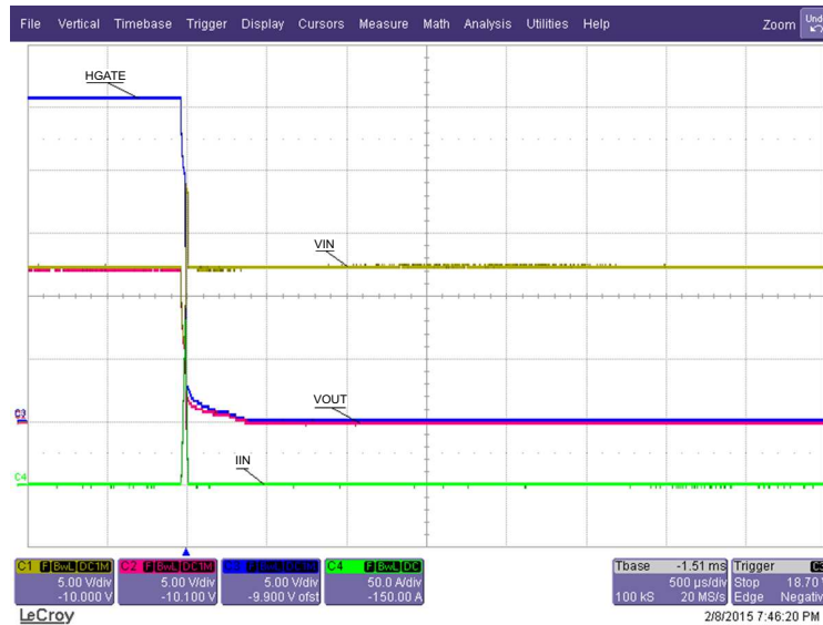
Figure 3. Hot Short With No Load on VOUT (Zoomed Out)
