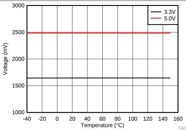
Figure 1. Quiescent Voltage vs Temperature
