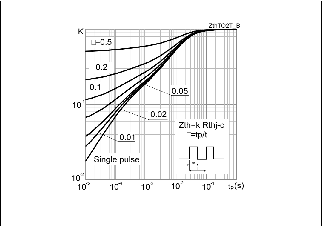
Figure 21. Thermal impedance
