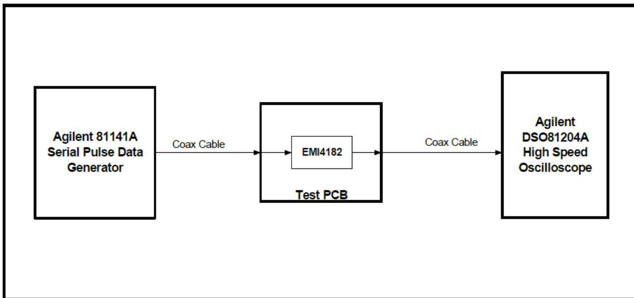
Figure 9. EMI4182MU Eye Diagram Test Setup
