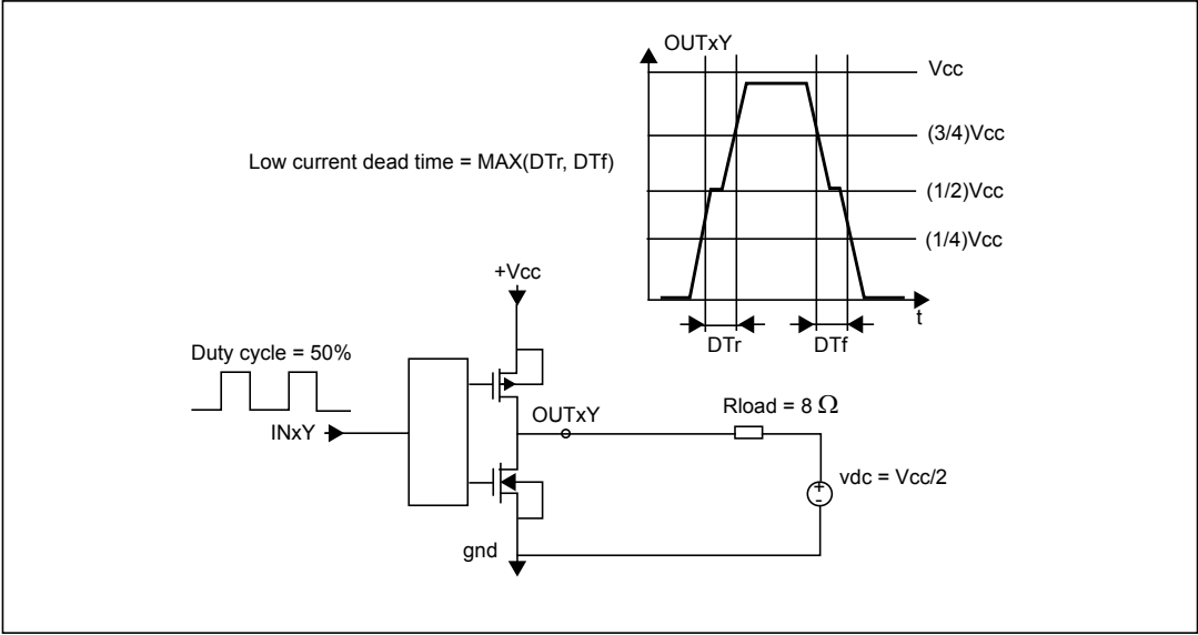
Figure 3. Test circuit
