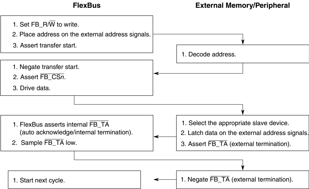
Figure 30-27. Write-Cycle Flowchart
