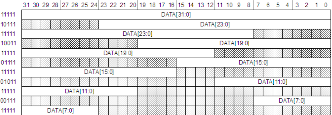
Figure 51-60. SAI first bit shifted, MSB first
