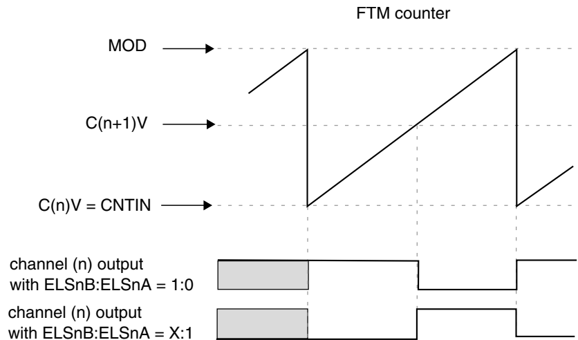
Figure 38-190. Channel (n) output if (C(n)V = CNTIN) and (CNTIN < C(n+1)V < MOD)
