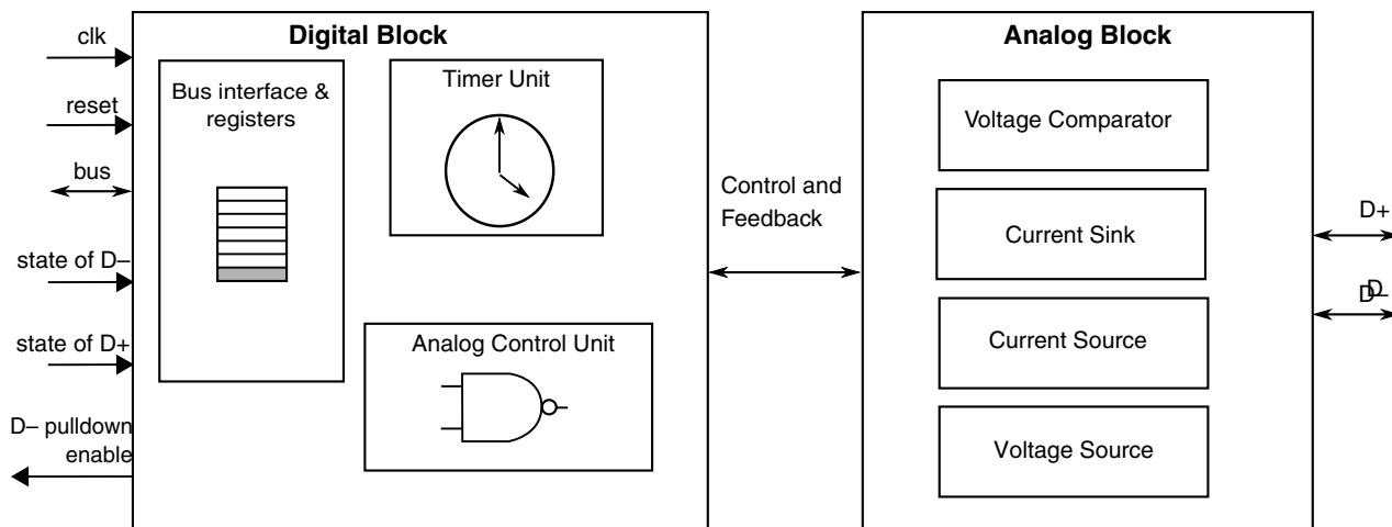
Figure 44-1. Block diagram
