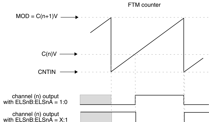
Figure 38-189. Channel (n) output if (CNTIN < C(n)V < MOD) and (C(n+1)V = MOD)
