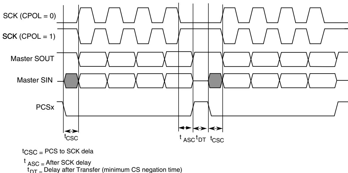
Figure 47-73. Example of non-continuous format (CPHA=1, CONT=0)
