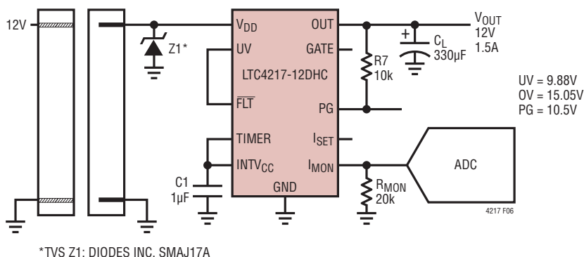
Figure 6. 1.5A, 12V Card Resident Application
