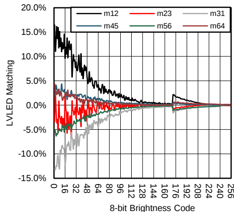
Exponential Mapping
