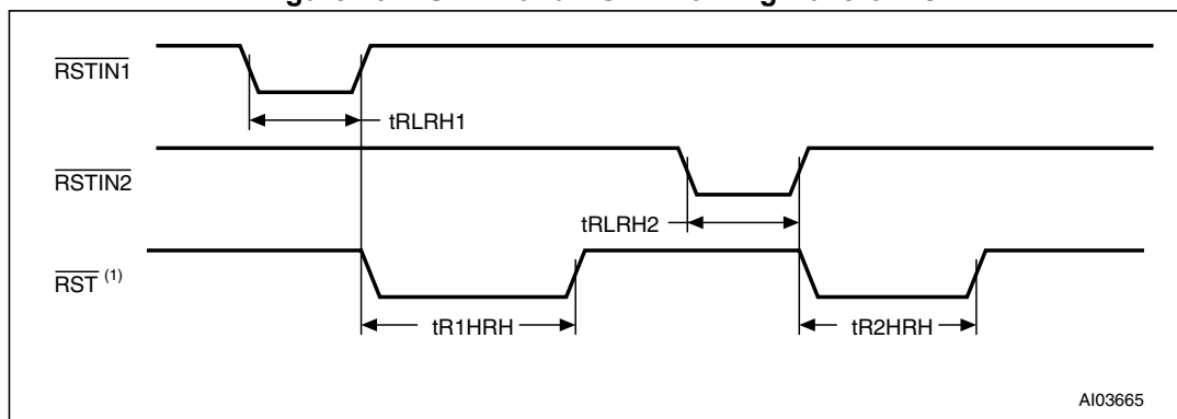
Figure 13. \overline{\text{RSTIN1}} and \overline{\text{RSTIN2}} timing waveforms
