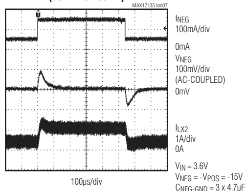
NEG LOAD-TRANSIENT RESPONSE (50mA TO 150mA)
