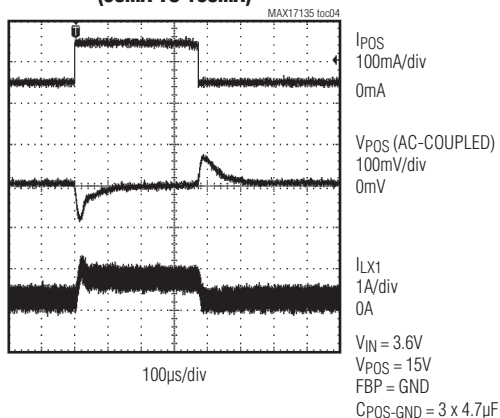
POS LOAD-TRANSIENT RESPONSE (50mA TO 150mA)
