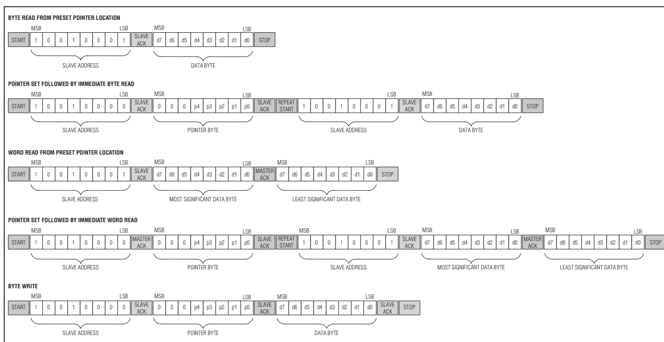
Figure 4. Read/Write Protocols
