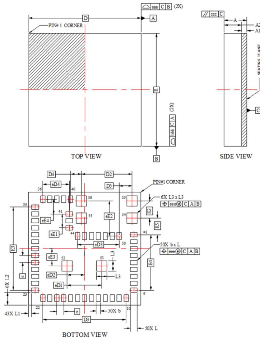
Figure 8.1. BGM121/BGM123 Package Dimensions
