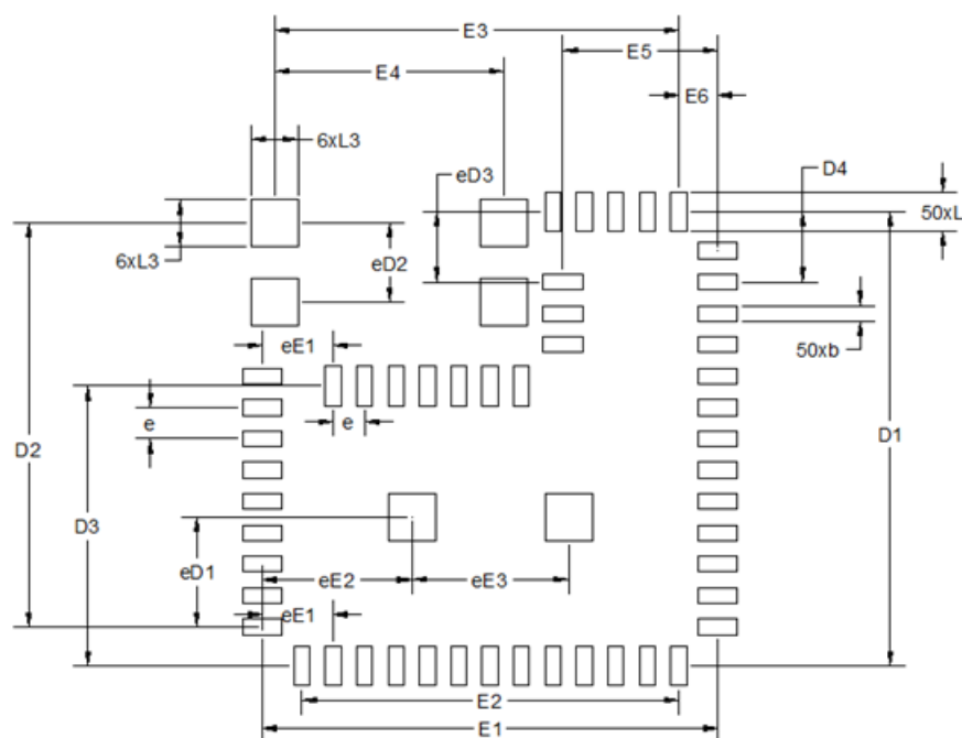
Figure 8.3. Module Footprint
