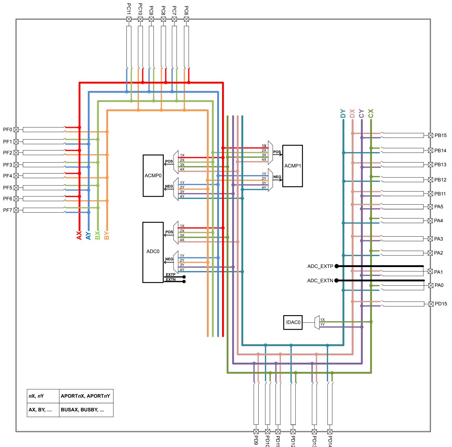
Figure 7.2. BGM121/BGM123 APORT
