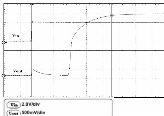
Figure 13. Enable transient
