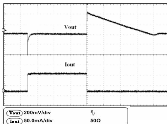
Figure 11. Load transient
