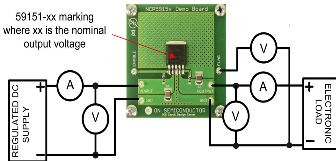
Figure 1: Test Setup
