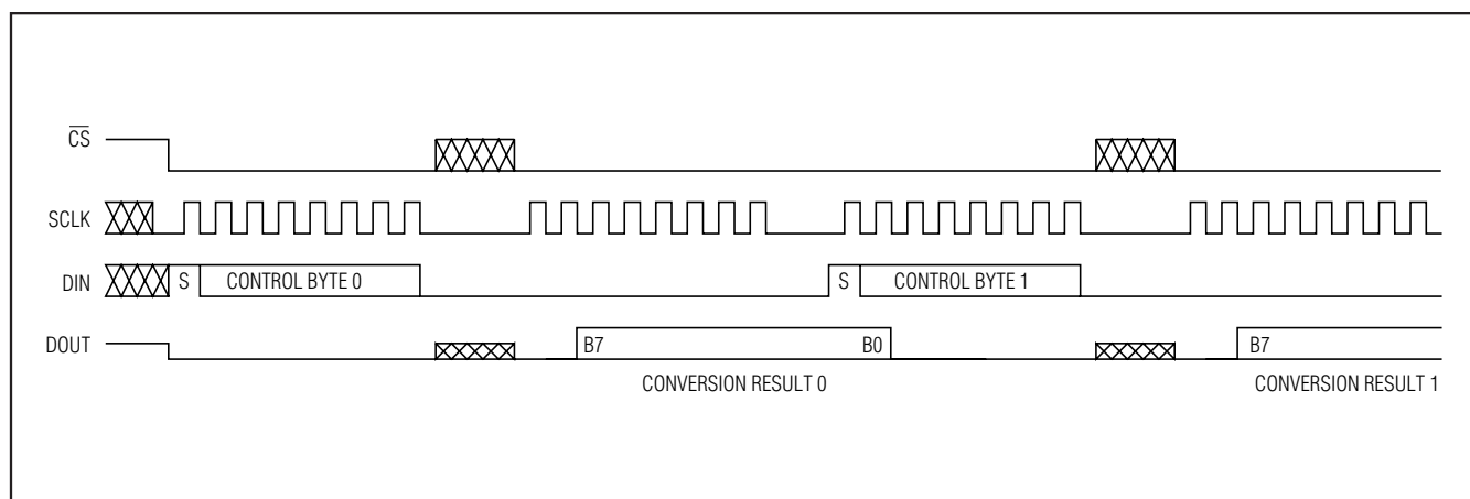
Figure 12b. Continuous Conversions, External Clock Mode, 16 Cycles/Conversion Timing
