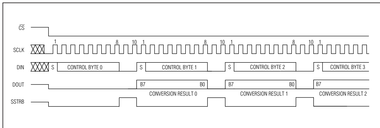
Figure 12a. Continuous Conversions, External Clock Mode, 10 Cycles/Conversion Timing
