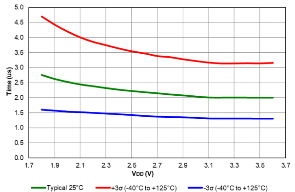
Figure 41-66. ADC RC Oscillator Period, PIC16LF18426/46 only
