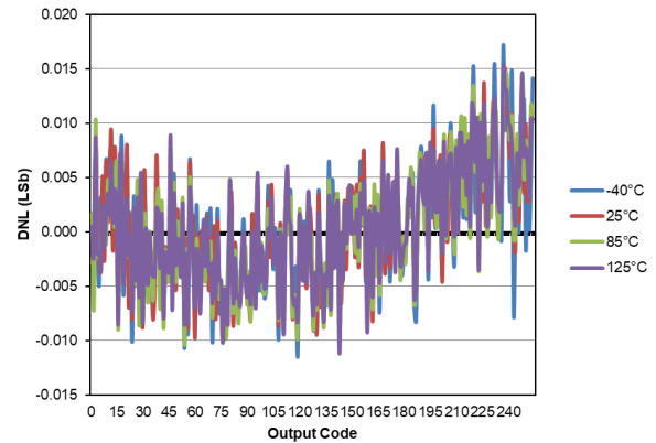
Figure 41-72. DAC DNL Error, V_{DD} = 3.0V , PIC16LF18426/46 only
