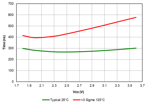
Figure 41-89. Band Gap Ready Time, PIC16LF18426/46 only
