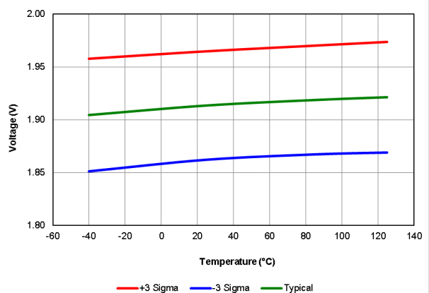
Figure 41-42. Brown-Out Reset Voltage, Trip Point BORV = 01, PIC16F18426/46 only
