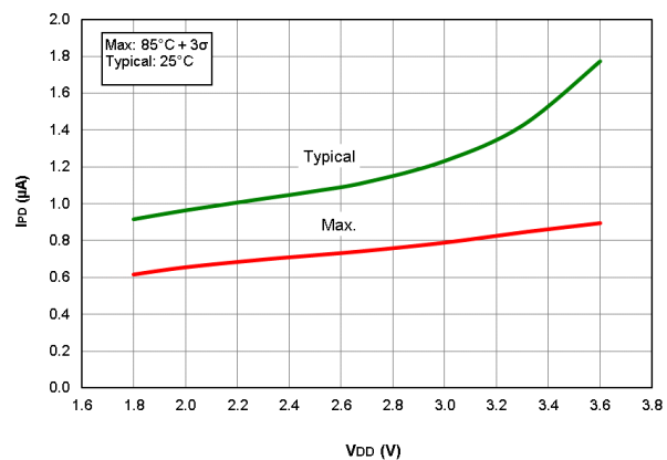
Figure 41-2. I_{PD} Watchdog Timer (WDT), PIC16LF18426/46 only
