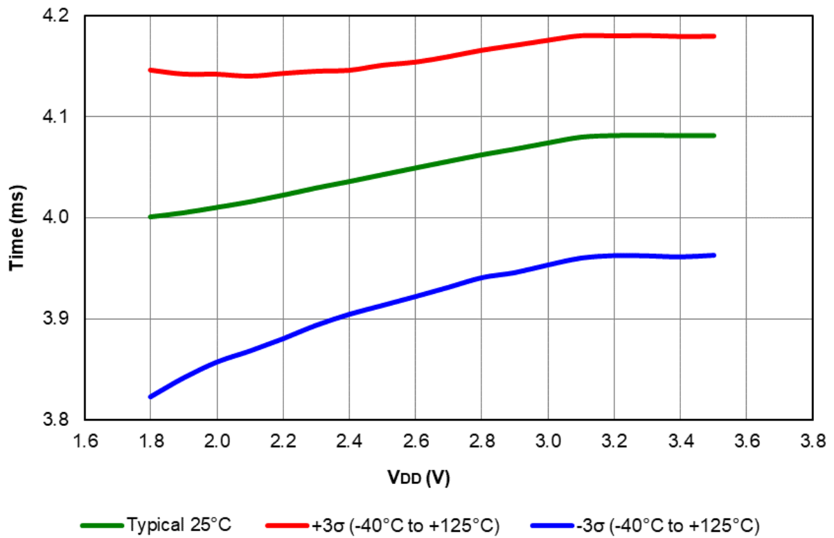
Figure 41-115. WDT Time-Out Period, PIC16LF18426/46 only
