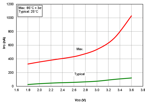
Figure 41-1. I_{PD} Base, Low-Power Sleep Mode, PIC16LF18426/46 only
