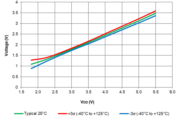
Figure 41-96. Schmitt Trigger High Values, All devices
