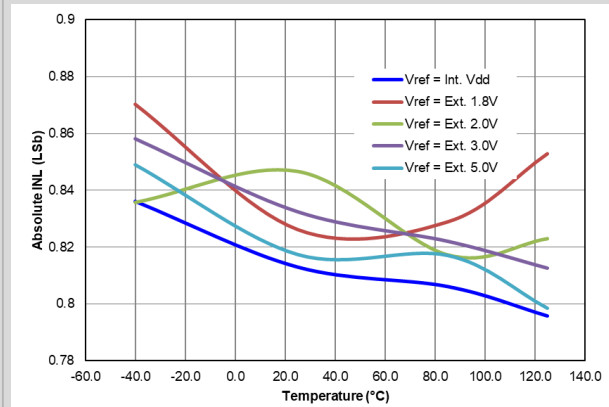
Figure 41-76. Absolute Value of DAC INL Error, V_{DD} = 5.0V , V_{REF} = V_{DD} , PIC16F18426/46 only
