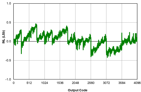
Figure 41-53. ADC 12-Bit Mode, Single-Ended INL, V_{DD} = 3.0V , V_{REF} = 3.0V , T_{AD} = 4 \mu s , 25^{\circ}C , All devices
