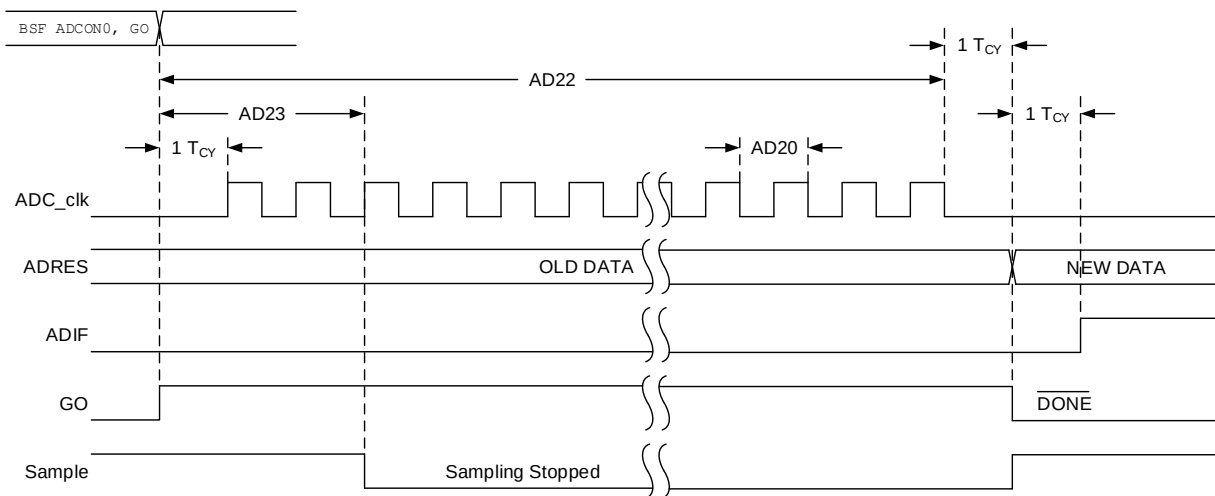
Figure 40-10. ADC Conversion Timing (ADC Clock F OSC -Based)
