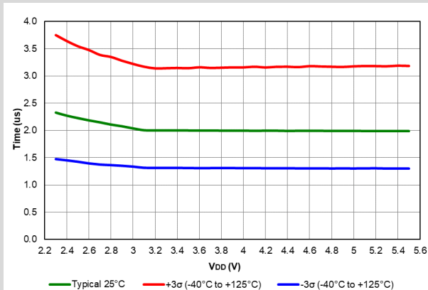
Figure 41-67. ADC RC Oscillator Period, PIC16F18426/46 only
