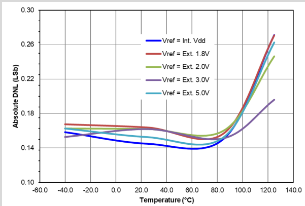
Figure 41-75. Absolute Value of DAC DNL Error, V_{DD} = 5.0V , V_{REF} = V_{DD} , PIC16F18426/46 only
