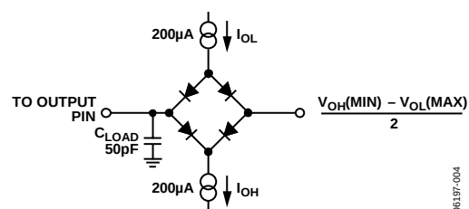
Figure 4. Load Circuit for \text{SDO} , \overline{\text{BUSY}} Timing Diagram
