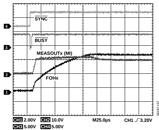
Figure 45. FV Settling, 0 \text{ V} to 5 \text{ V} , \pm 20 \mu\text{A} Range, C_{\text{LOAD}} = 220 \text{ pF} , C_{\text{COMP}x} = 100 \text{ pF} , R_{\text{LOAD}} = 270 \text{ k}\Omega
