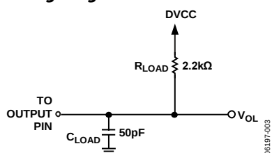
Figure 3. Load Circuit for \overline{\text{CGALM}} , \overline{\text{TMPALM}}
