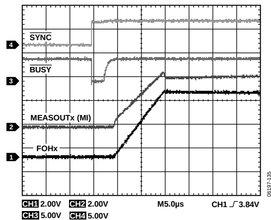
Figure 43. FV Settling, 0 \text{ V} to 5 \text{ V} , \pm 2 \text{ mA} Range, C_{\text{LOAD}} = 220 \text{ pF} , C_{\text{COMP}x} = 100 \text{ pF} , R_{\text{LOAD}} = 5.6 \text{ k}\Omega
