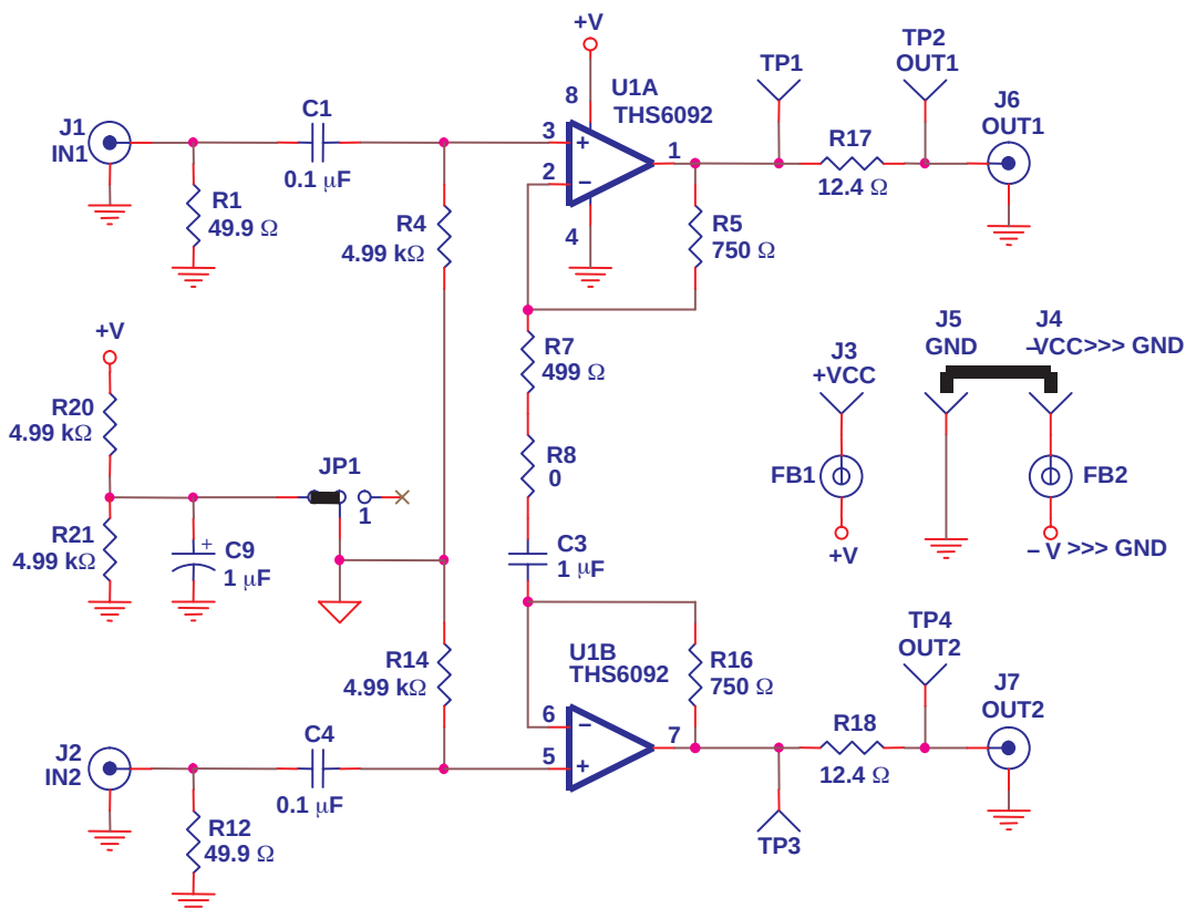
Figure 3–2. Single-Supply Operation
