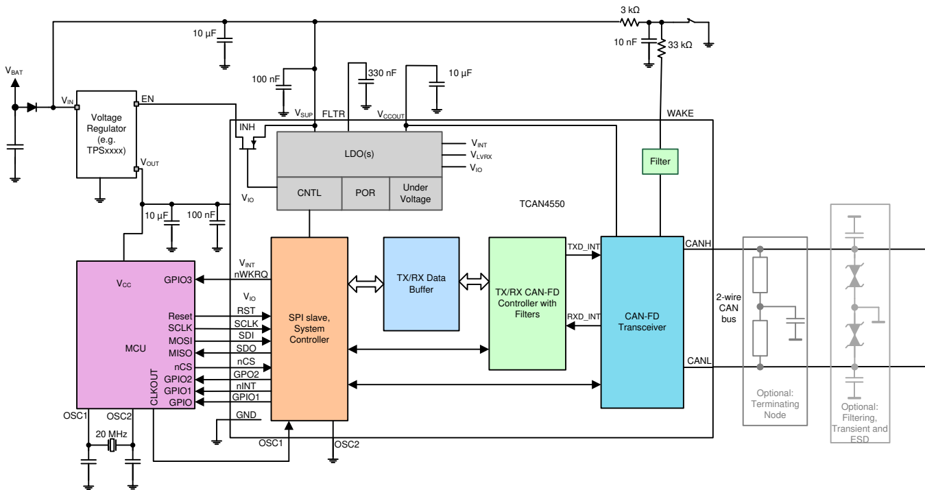
Figure 108. Typical CAN Applications for TCAN4550-Q1 for 3.3 V \mu C; Clock from MCU
