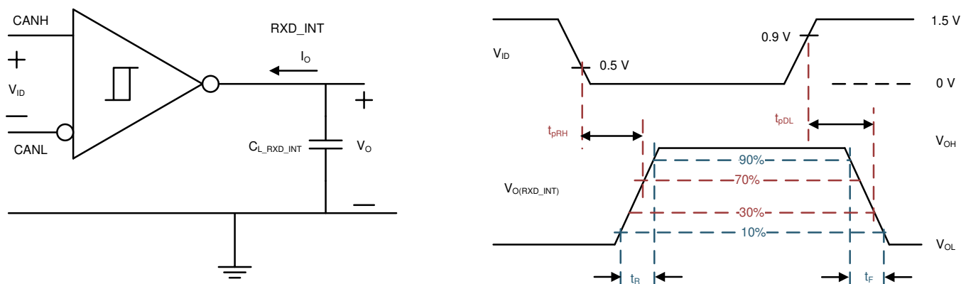
Figure 7. Receiver Test Circuit and Measurement
