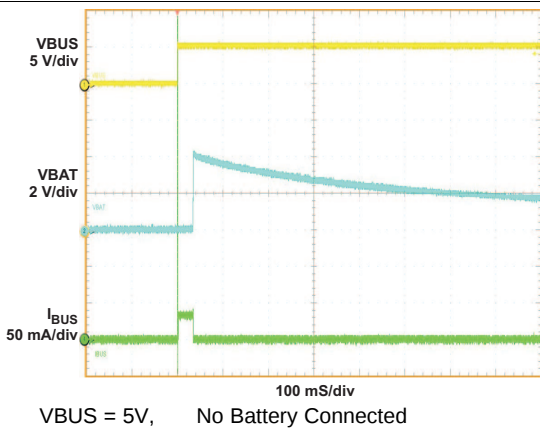
Figure 28. Adapter Insertion
