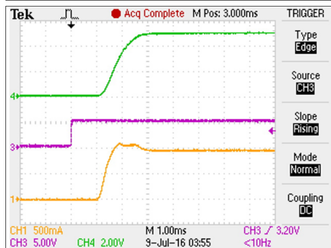
Figure 11. Turnon Delay
