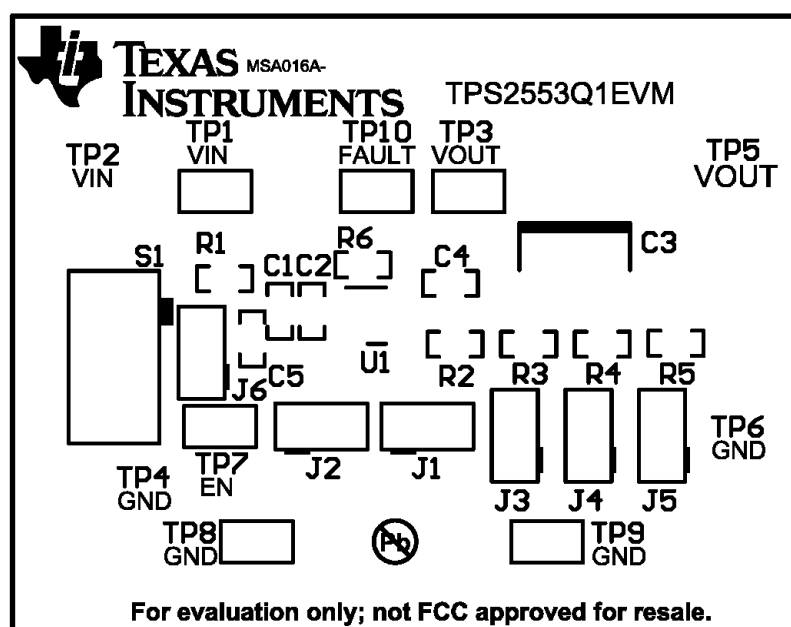
Figure 6. Top Overlay
