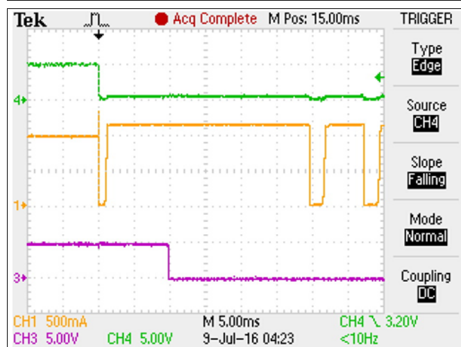
Figure 14. 5-Ohm Load to Short-Circuit Transient
