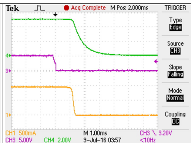
Figure 12. Turnoff Delay
