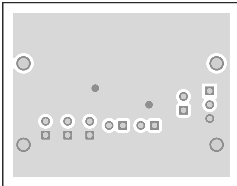
Figure 7. Layout—Bottom Composite
