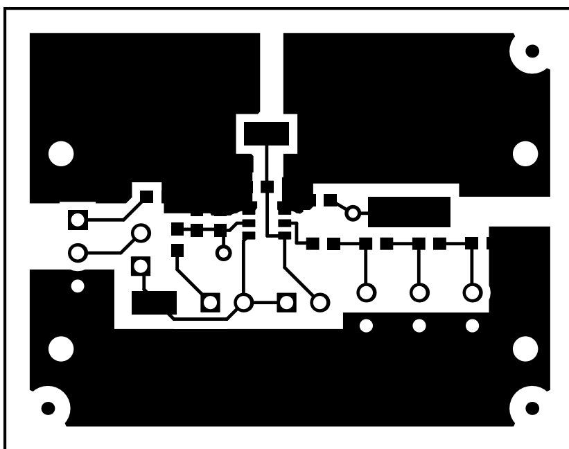
Figure 8. Top Layer
