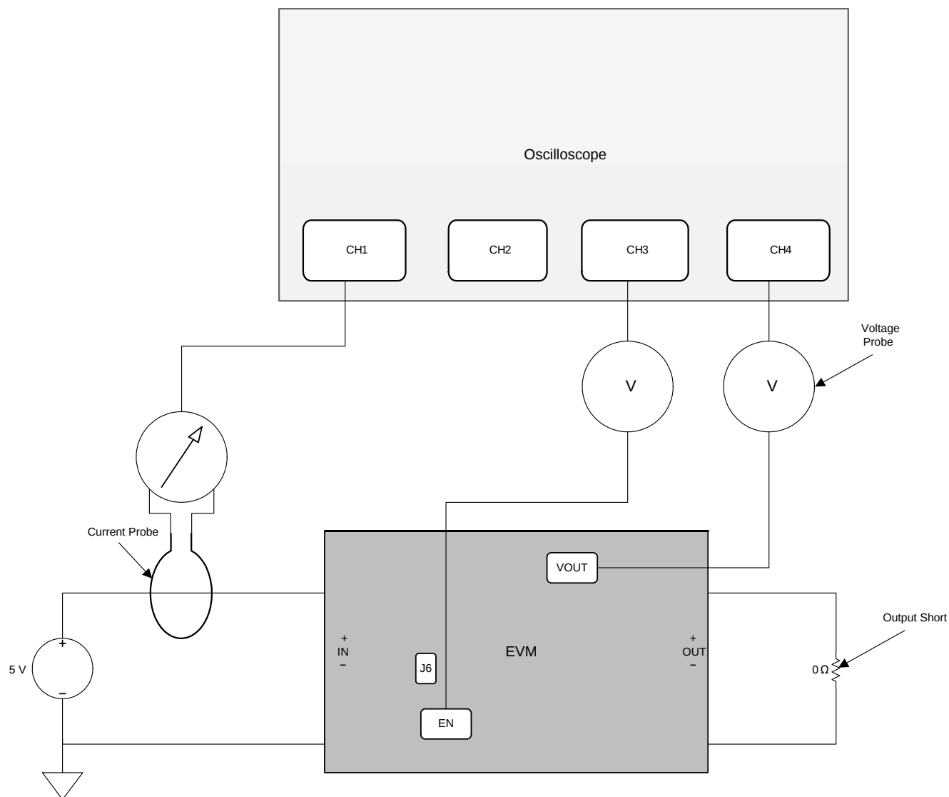
Figure 10. Test Setup for Turnon and Turnoff Delay
