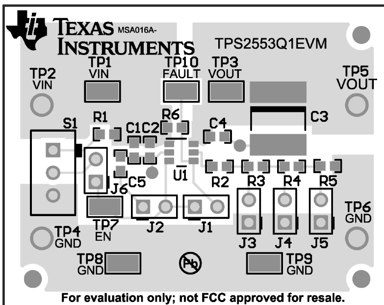
Figure 5. Layout—Top Composite
