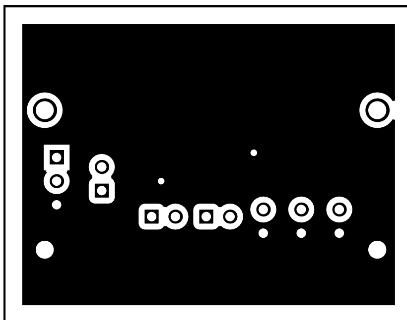
Figure 9. Bottom Layer
