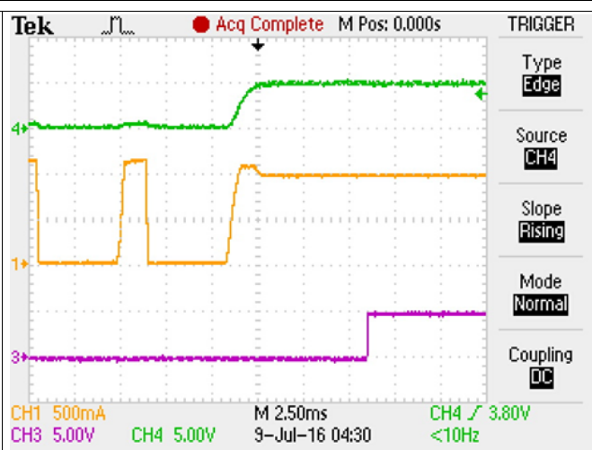
Figure 15. Short-Circuit to 5-Ohm Load Transient
