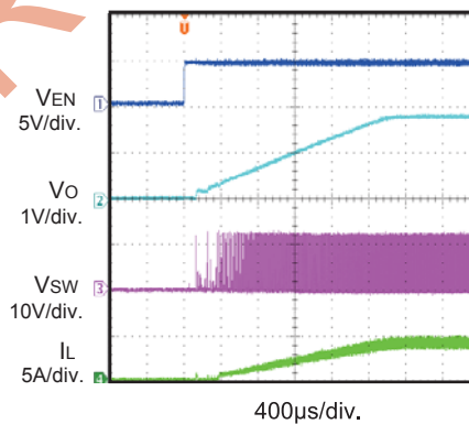
Enable Start-up
