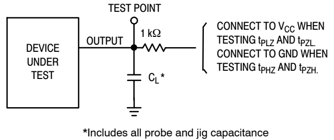
Figure 7. Test Circuit
