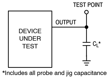
Figure 6. Test Circuit
