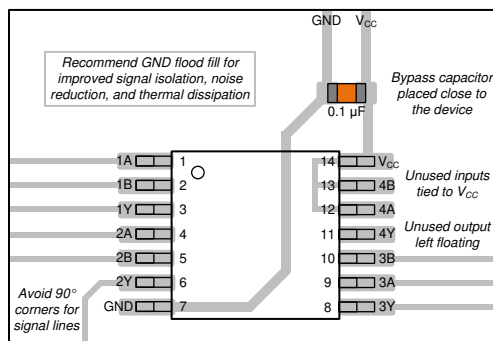
Figure 11. Example layout for the SN74HCS00
