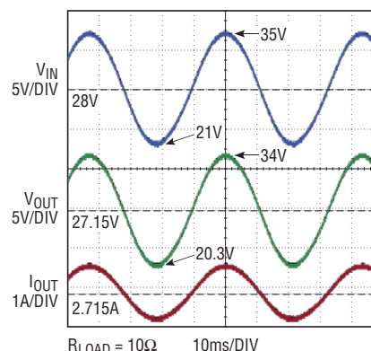
Figure 5. 14V p-p Input Ripple Condition
