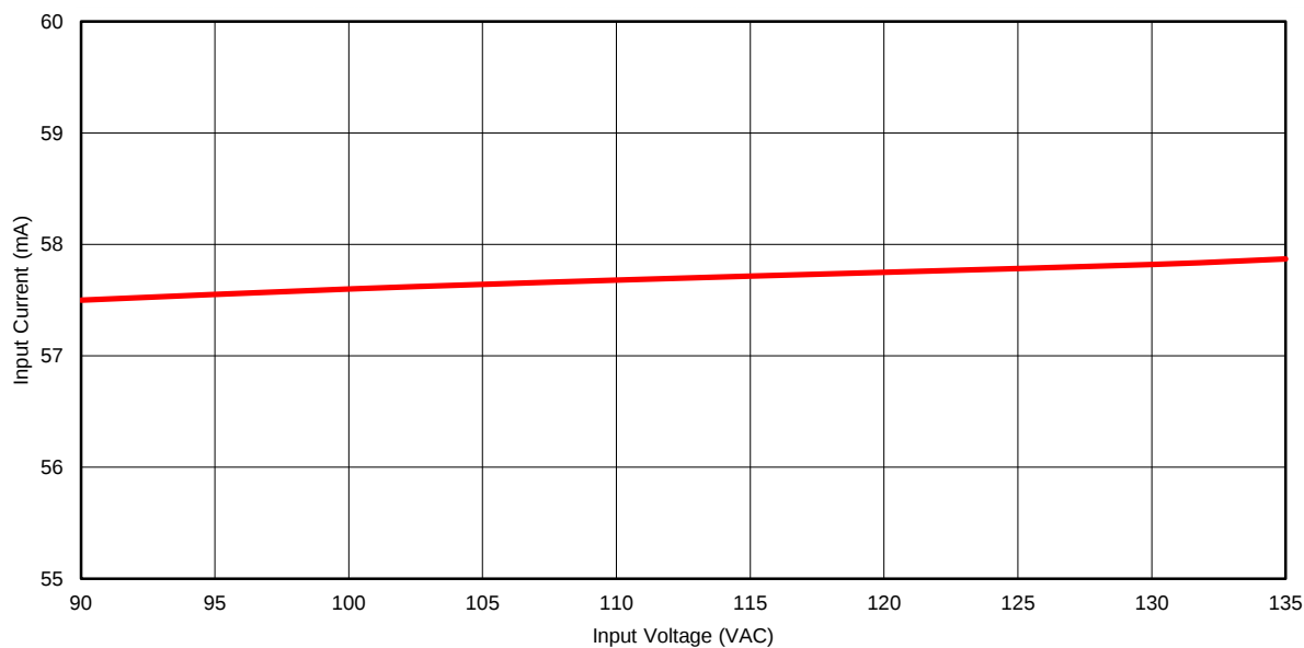
Figure 3. Input (Linear Regulator) Current Versus Input Voltage
