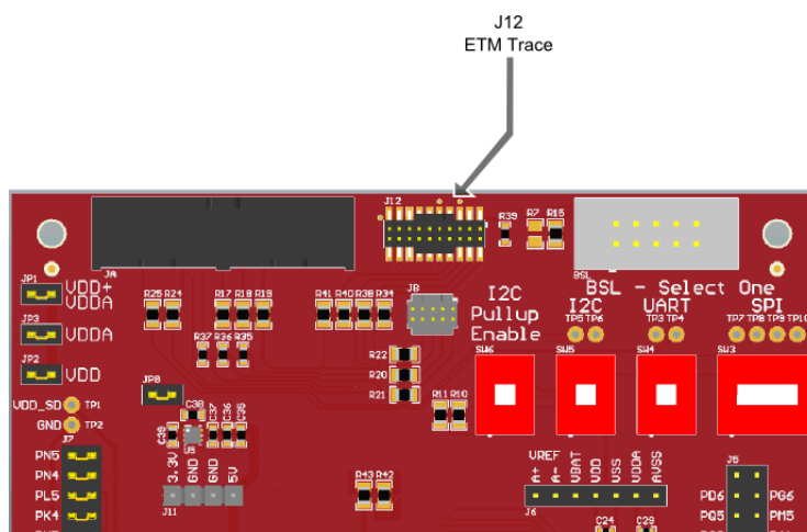
Figure 11. Arm ETM Trace Connector
