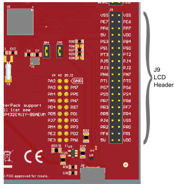
Figure 7. Header J9
