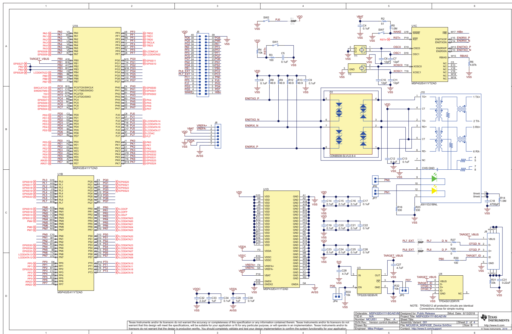
Figure 14. Schematics (2 of 3)
