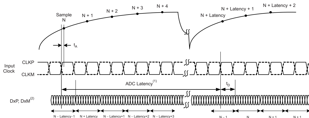
Figure 143. ADC Latency
