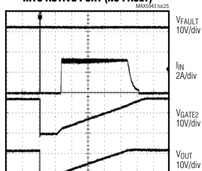
MAX5943A HOT PLUG-IN LOAD CAPACITANCE INTO ACTIVE PORT (NO FAULT)
