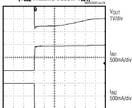
ORing SWITCHOVER WAVEFORM ( V_{IN2} FALLING BELOW V_{IN1} )
