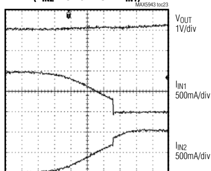
ORing SWITCHOVER WAVEFORM ( V_{IN2} RISING ABOVE V_{IN1} )
