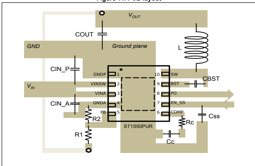
Figure 11. PCB layout
