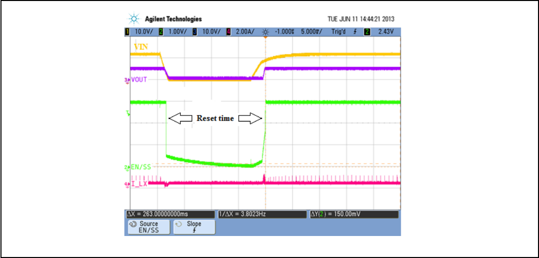
Figure 19. Reset time
