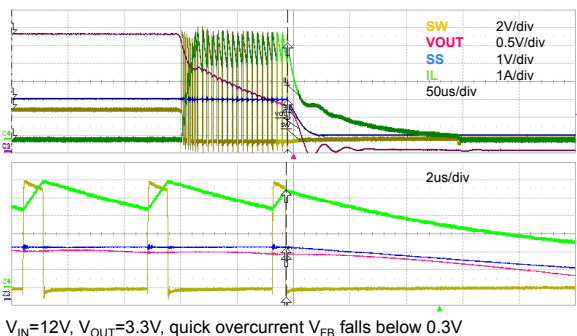
Figure 17. Quick overload
