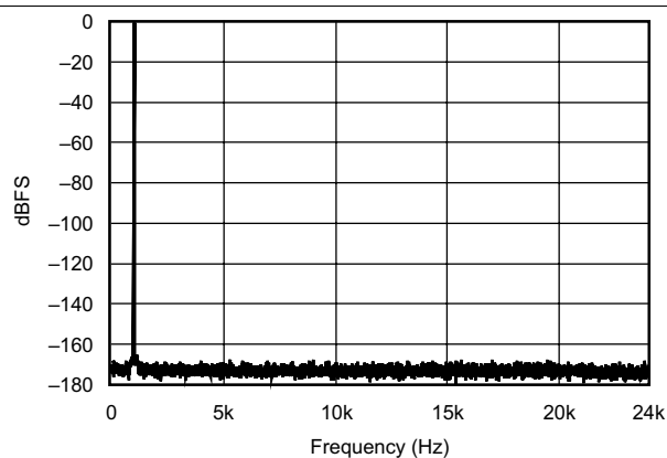
Figure 3. FFT With 1-kHz Input Tone at 0 dBFS
