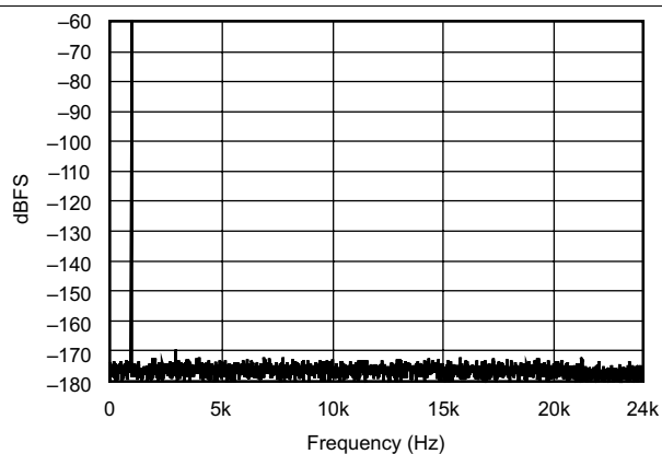
Figure 4. FFT With 1-kHz Input Tone at -60 dBFS
