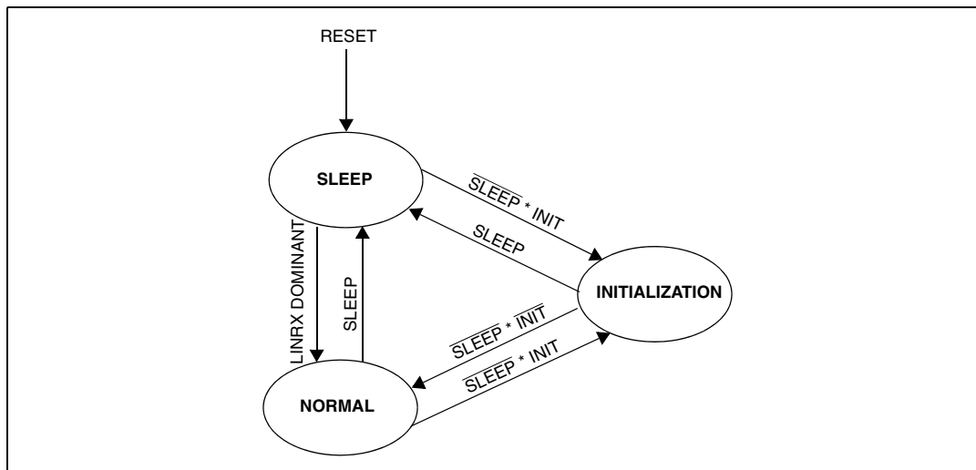
Figure 205. LINFlexD controller operating modes
