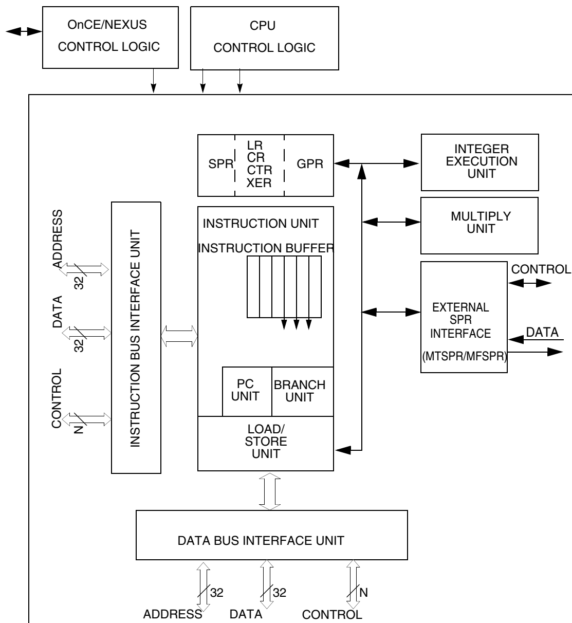
Figure 106. e200z0h block diagram
