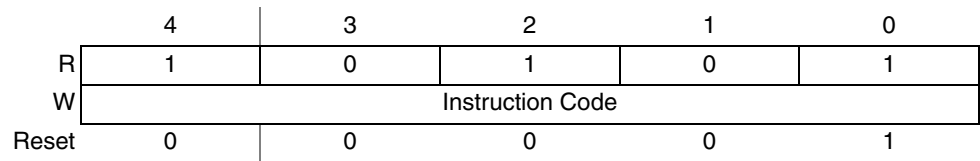
Figure 503. 5-bit Instruction Register
