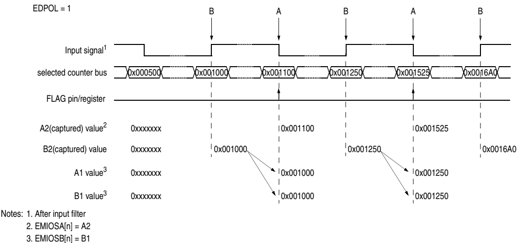
Figure 337. Input pulse width measurement example
