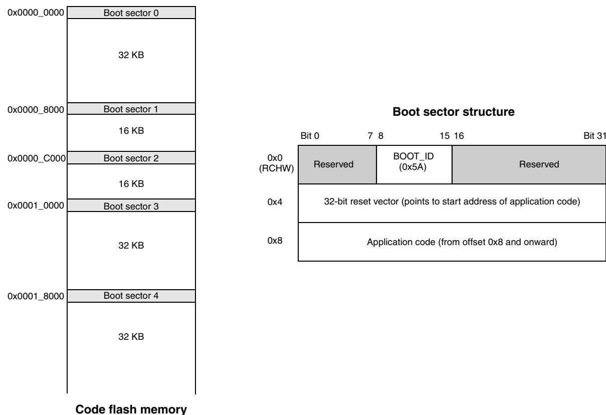
Figure 6. Boot sector structure
