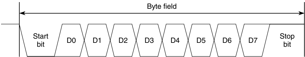
Figure 14. LINFlex bit timing in UART mode
