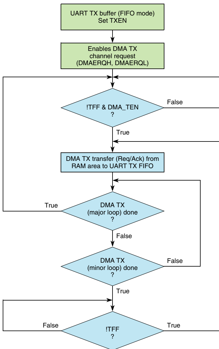
Figure 249. FSM to control the DMA TX interface (UART node)
