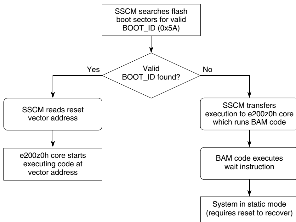
Figure 7. Flash memory boot mode sequence
