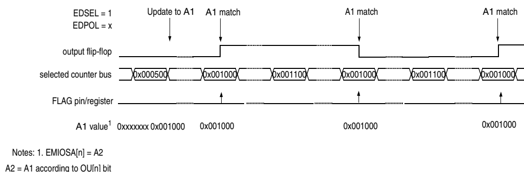
Figure 335. SAOC example toggling the output flip-flop
