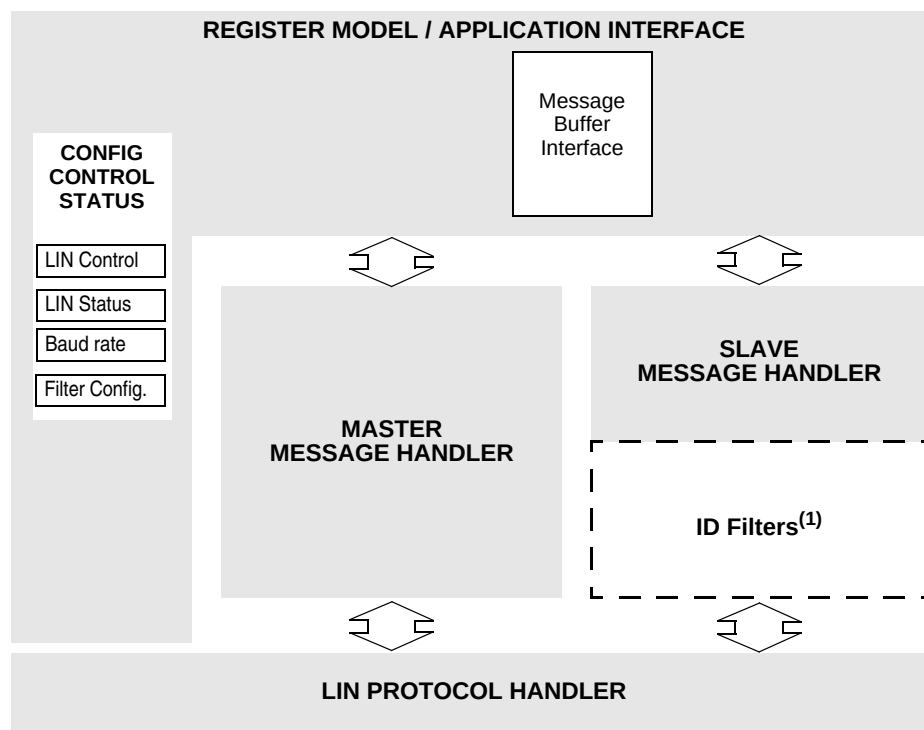
Figure 198. LINFlexD block diagram
