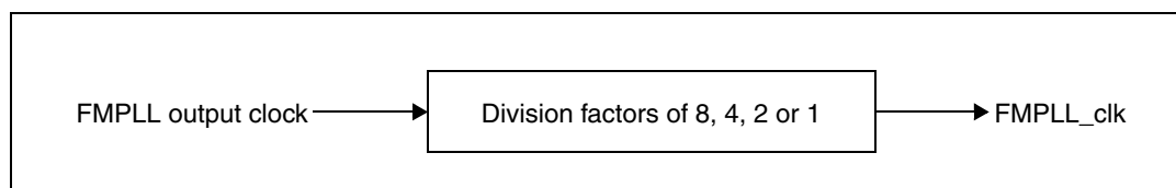
Figure 30. FMPLL output clock division flow during progressive switching
