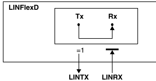
Figure 210. LINFlexD in Self Test mode
