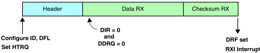
Figure 255. Programming consideration: master node, receiver
