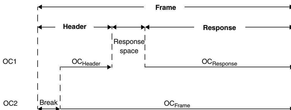
Figure 252. Header and response timeout
