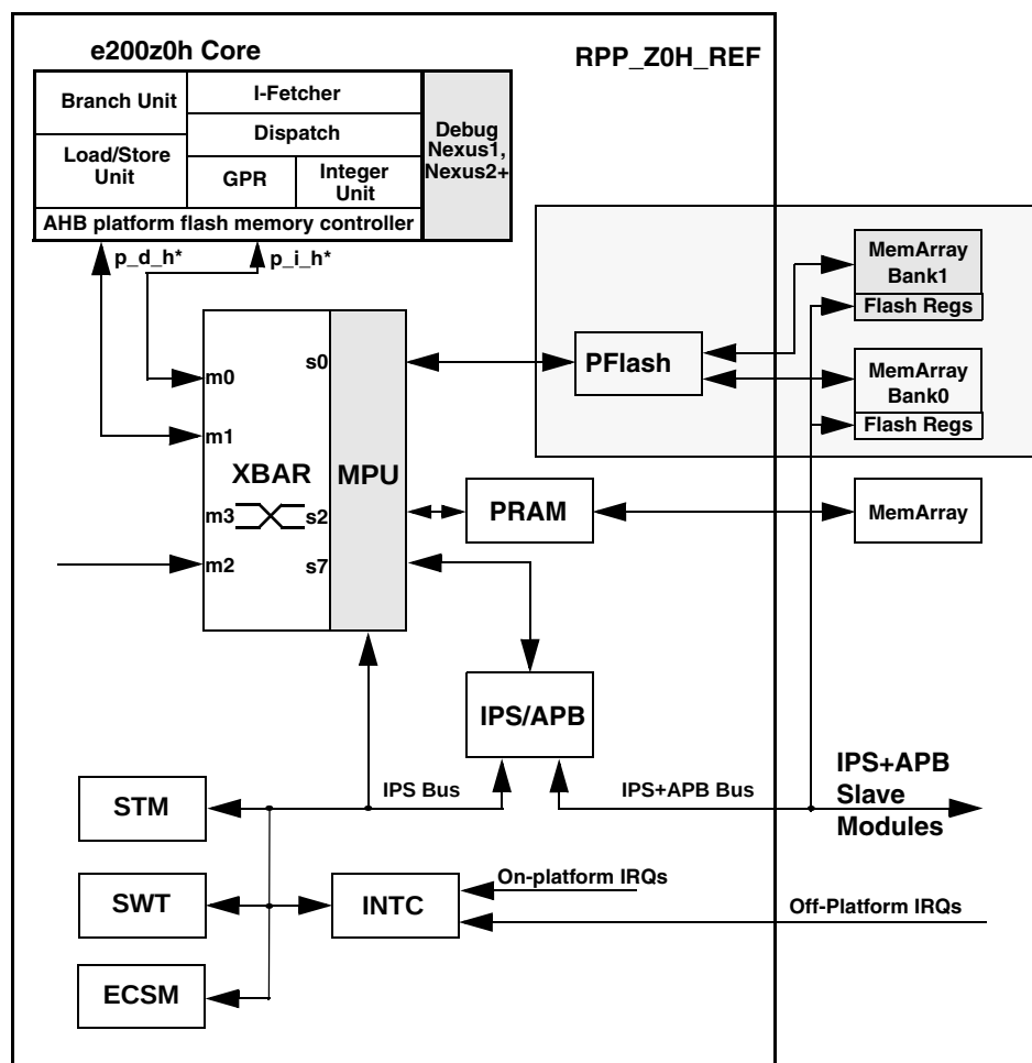
Figure 463. Power Architecture e200z0h RPP reference platform block diagram
