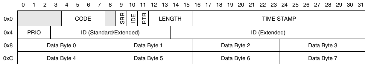
Figure 274. Message Buffer Structure
