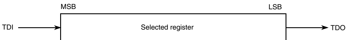
Figure 505. Shifting data through a register
