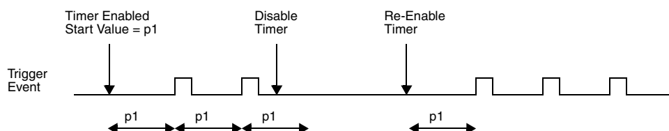
Figure 376. Stopping and starting a timer
