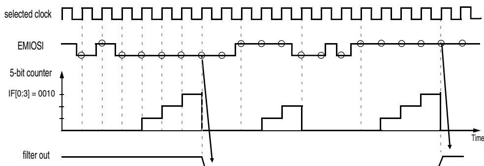
Figure 365. Input programmable filter example
