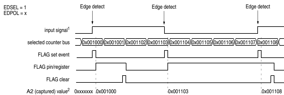
Figure 333. Single action input capture with both edges triggering example
