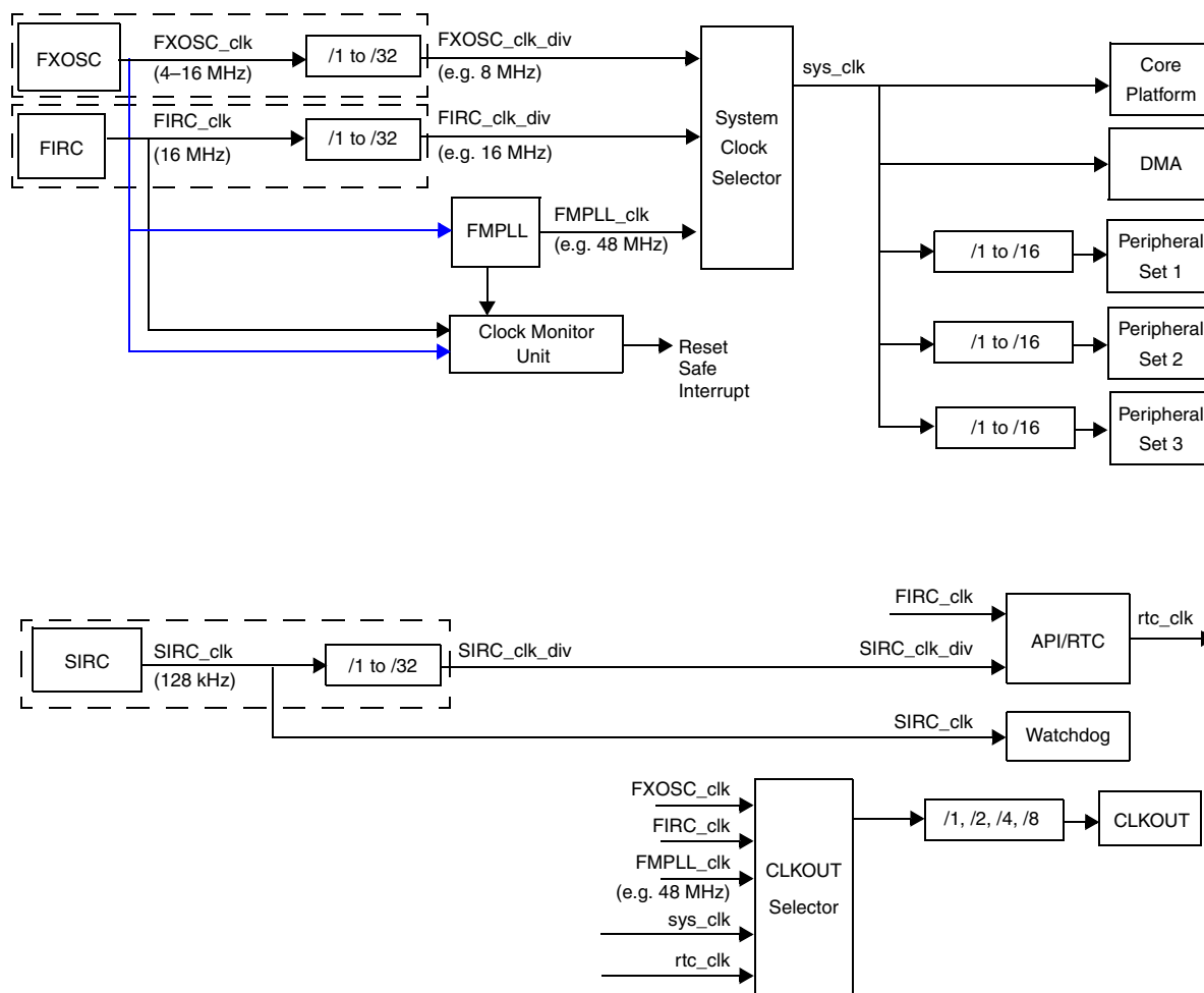
Figure 23. SPC560D30/40 system clock generation
