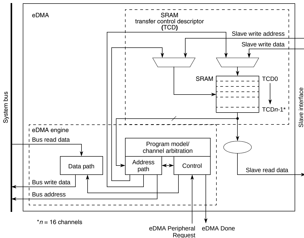
Figure 108. eDMA block diagram
