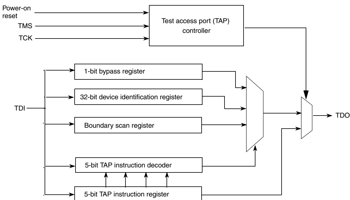
Figure 502. JTAG Controller Block Diagram
