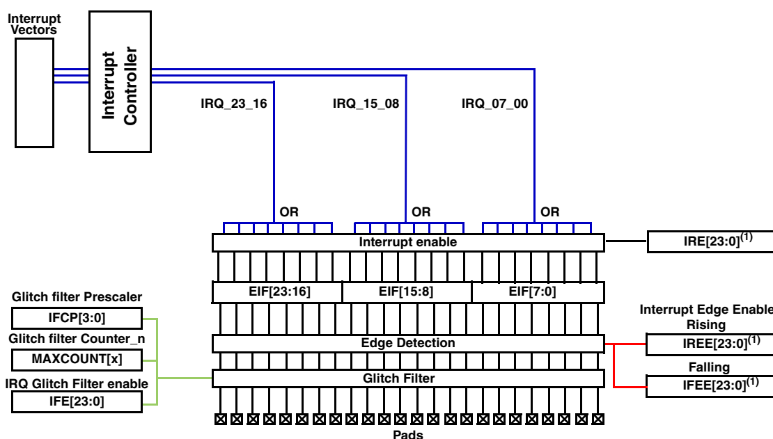
Figure 165. External interrupt pad diagram
