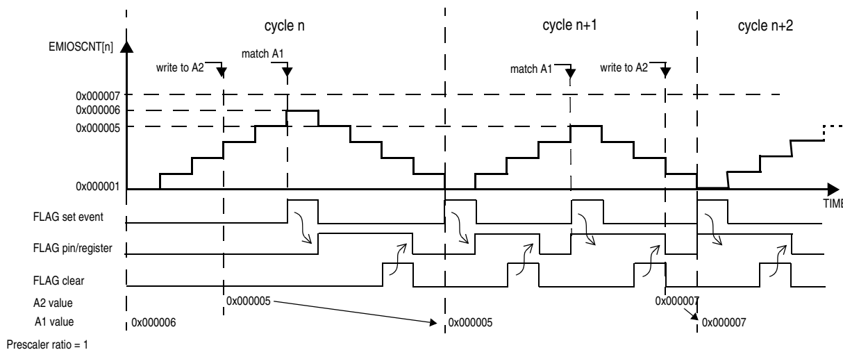
Figure 347. Modulus Counter Buffered (MCB) Up/Down mode
