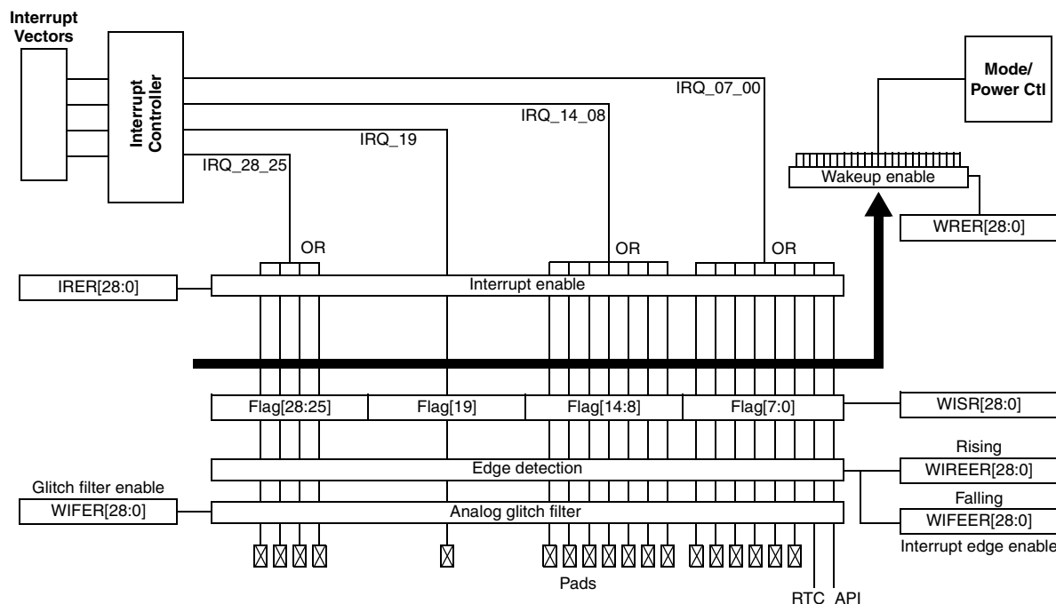
Figure 99. External interrupt pad diagram
