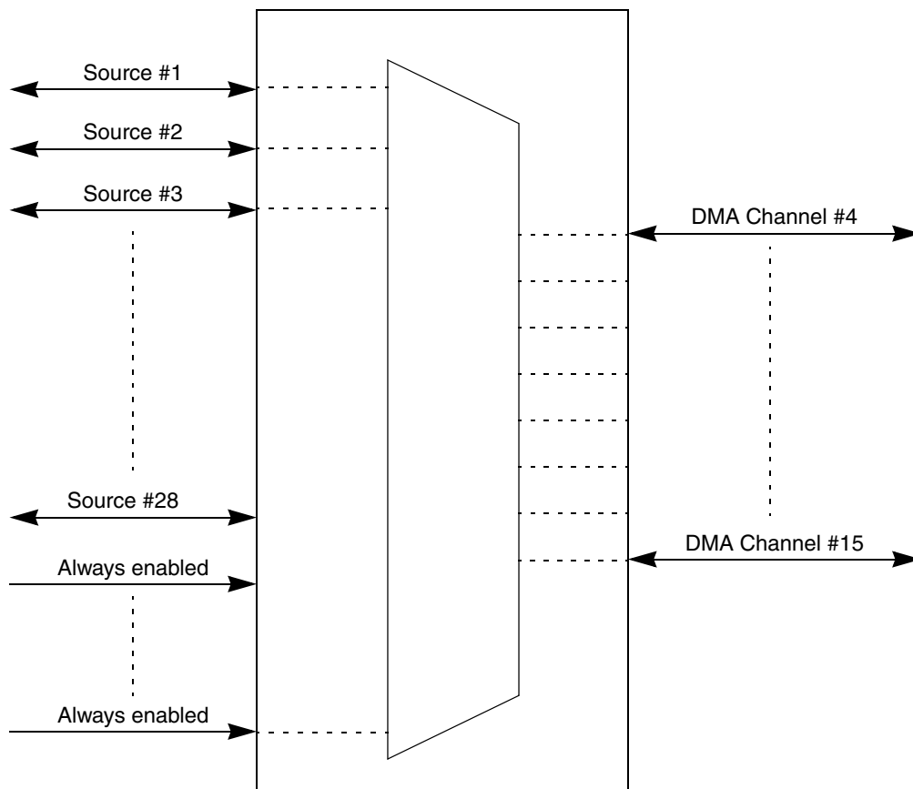
Figure 136. DMA_MUX channel 4–15 block diagram
