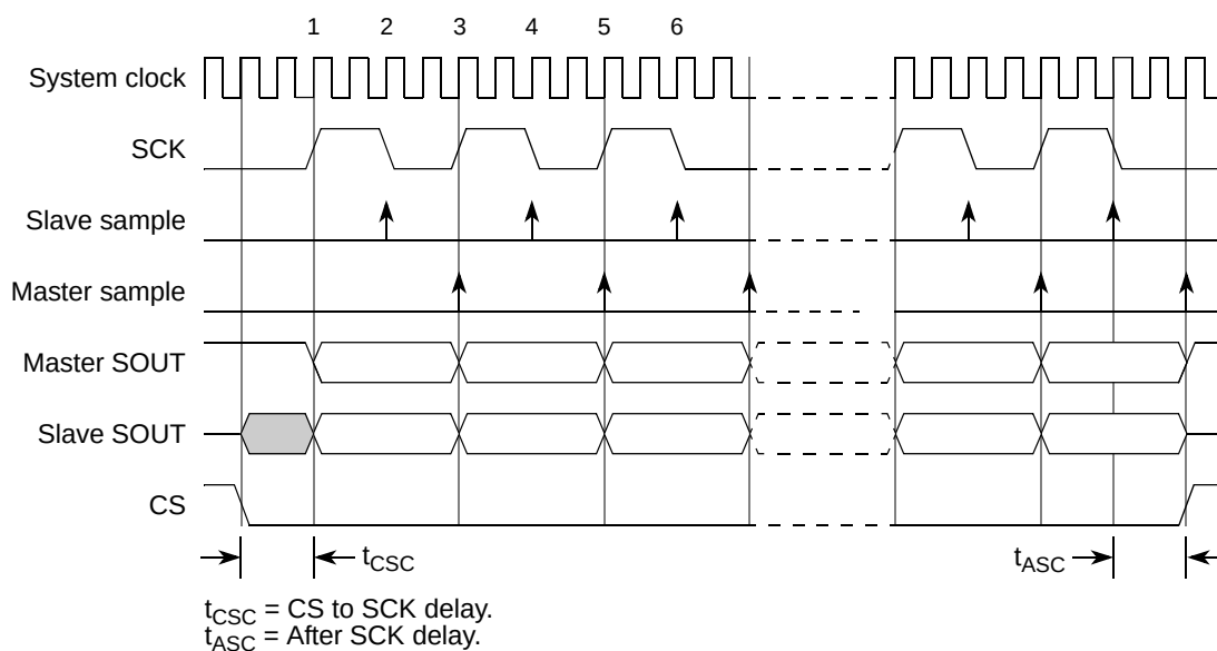
Figure 308. DSPI modified transfer format ( MTFE = 1 , CPHA = 1 , f_{SCK} = f_{sys} / 4 )
