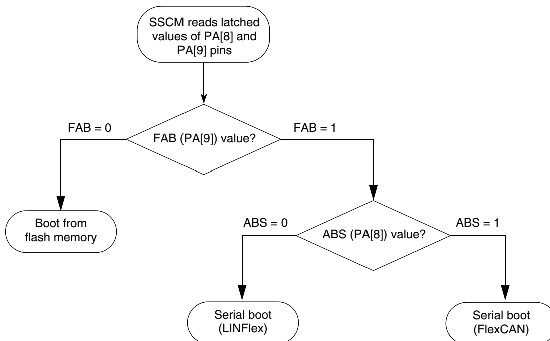
Figure 5. Boot mode selection
