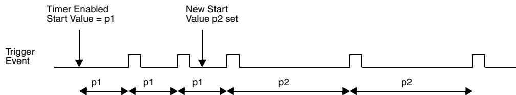
Figure 378. Dynamically setting a new load value
