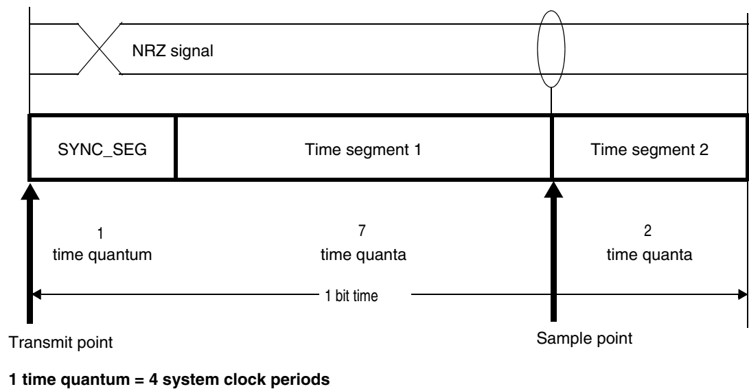
Figure 15. FlexCAN bit timing
