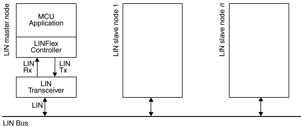
Figure 166. LIN topology network
