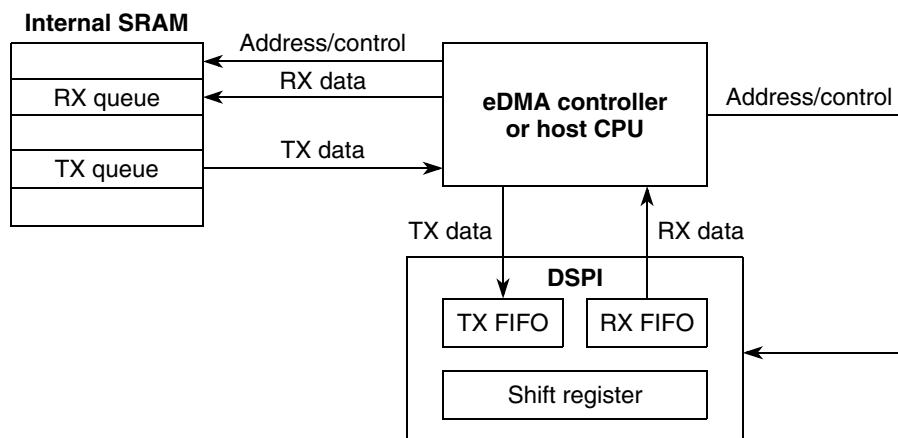
Figure 291. DSPI with queues and eDMA
