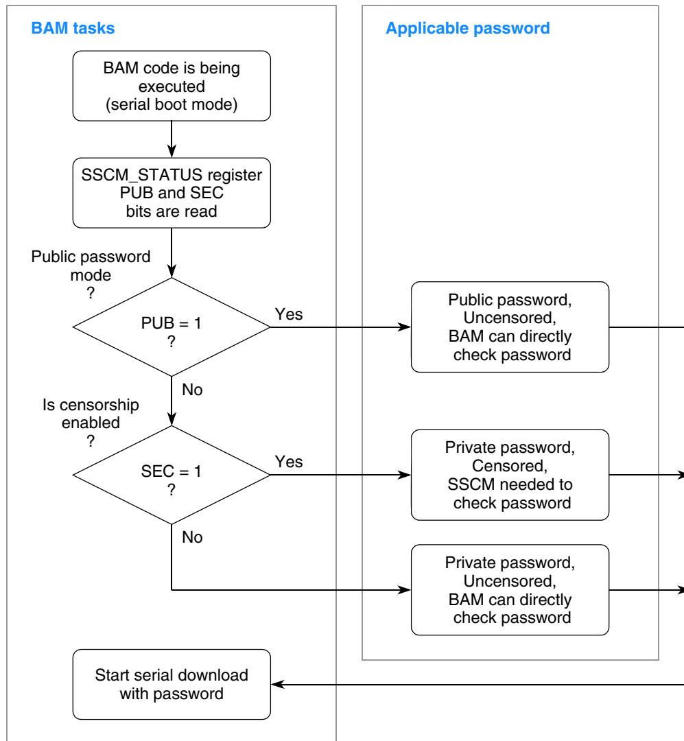
Figure 11. BAM censorship mode detection
