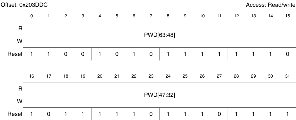
Figure 444. CFlash Nonvolatile Private Censorship Password 1 Register (NVPWD1)
