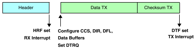
Figure 258. Programming consideration: slave node, transmitter, no filters
