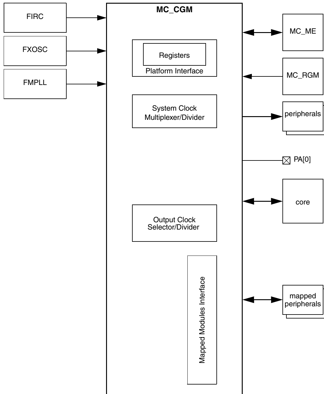
Figure 39. MC_CGM block diagram
