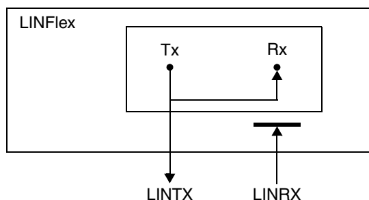
Figure 169. LINFlex in loop back mode
