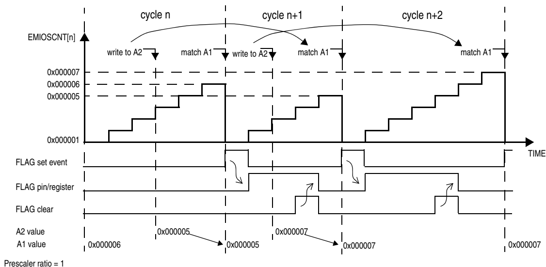
Figure 346. Modulus Counter Buffered (MCB) Up Count mode
