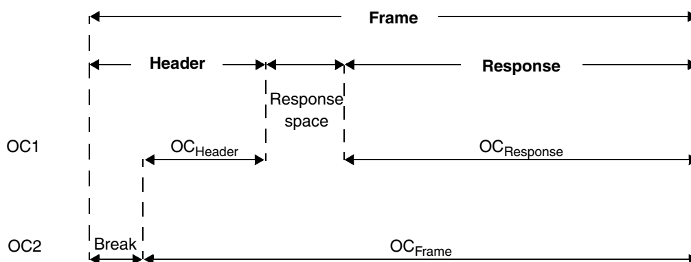
Figure 197. Header and response timeout
