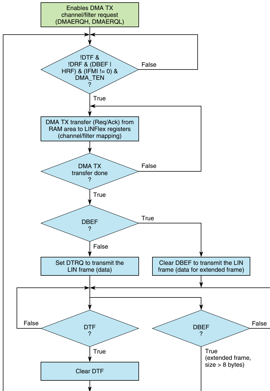
Figure 245. FSM to control the DMA TX interface (slave node)
