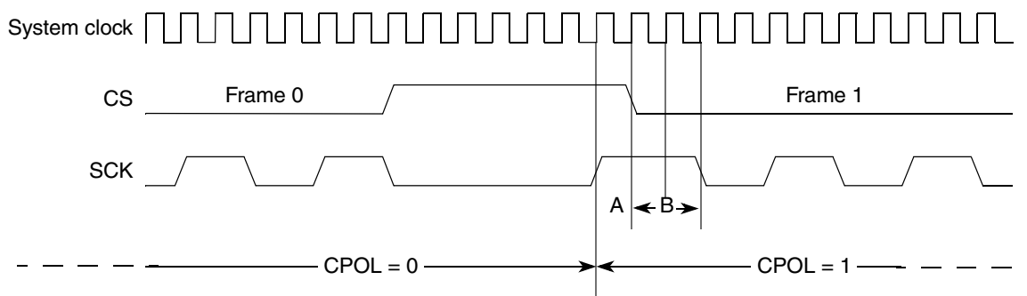
Figure 311. Polarity switching between frames
