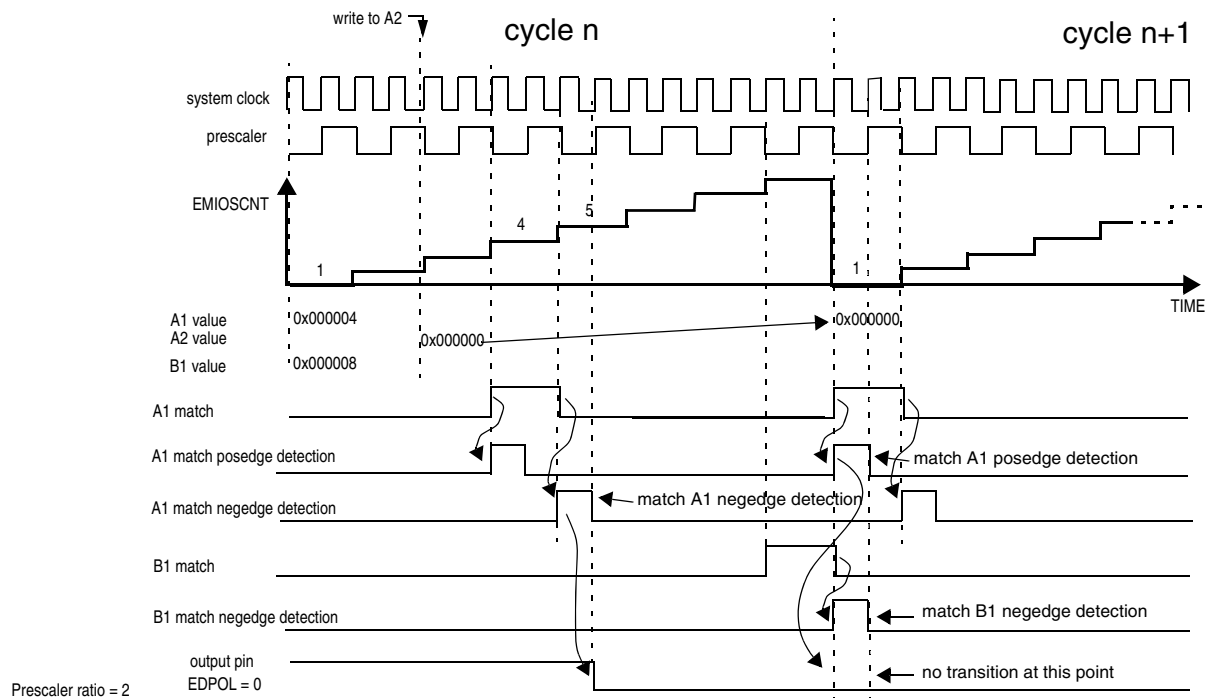
Figure 351. OPWFMB Mode with A1 = 0 (0% duty cycle)
