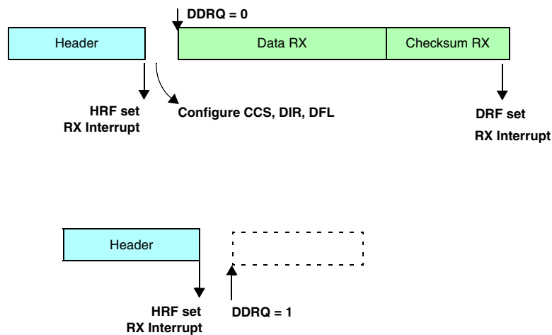
Figure 259. Programming consideration: slave node, receiver, no filters
