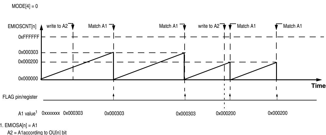
Figure 344. Modulus Counter Up mode example
