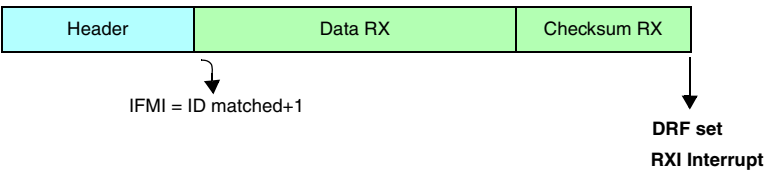
Figure 263. Programming consideration: slave node, at least one RX filter, BF is reset, ID matches filter
