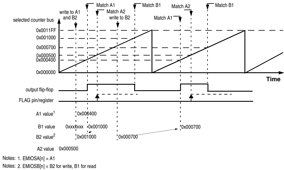
Figure 361. OPWMT example
