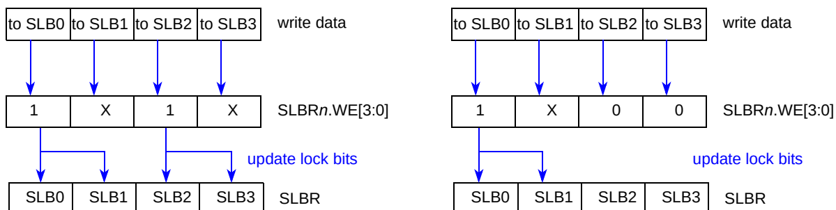
Figure 473. Change Lock Settings for 16-bit Protected Addresses
