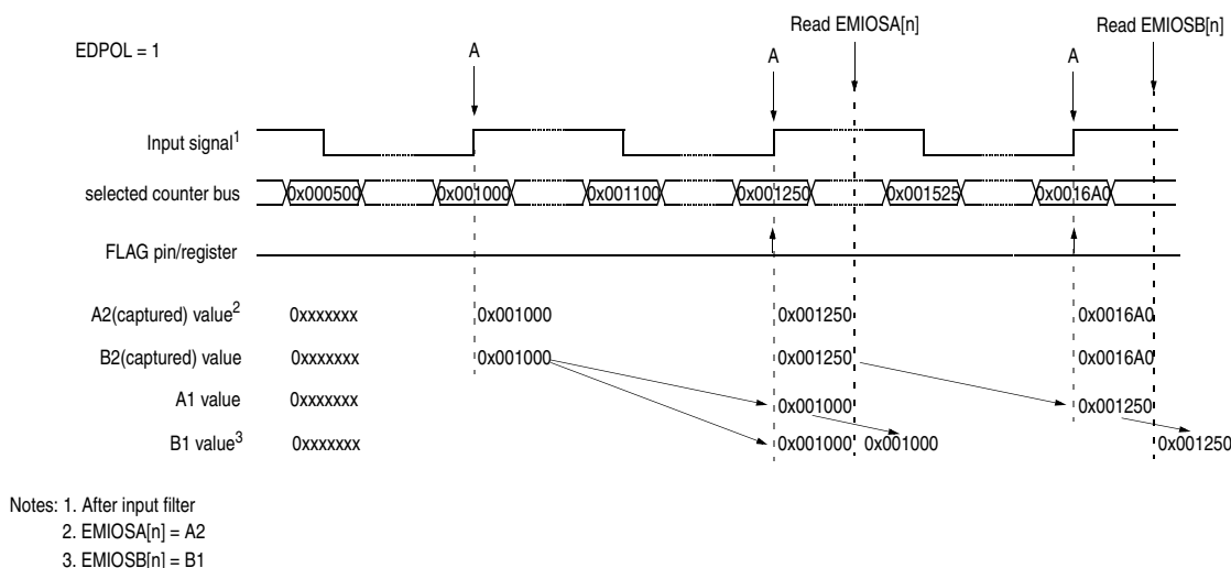
Figure 340. A1 and B1 updates at EMIOSA[n] and EMIOB[n] reads
