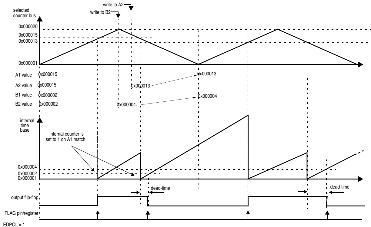
Figure 356. OPWMCB with trail dead time insertion
