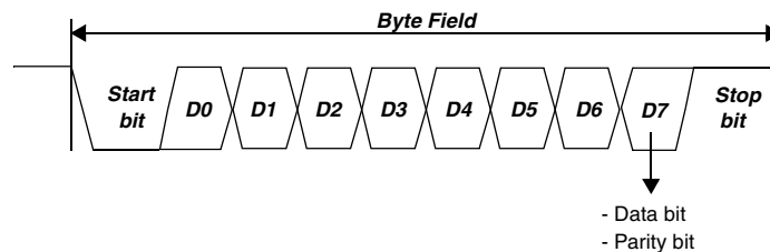
Figure 211. UART mode 8-bit data frame
