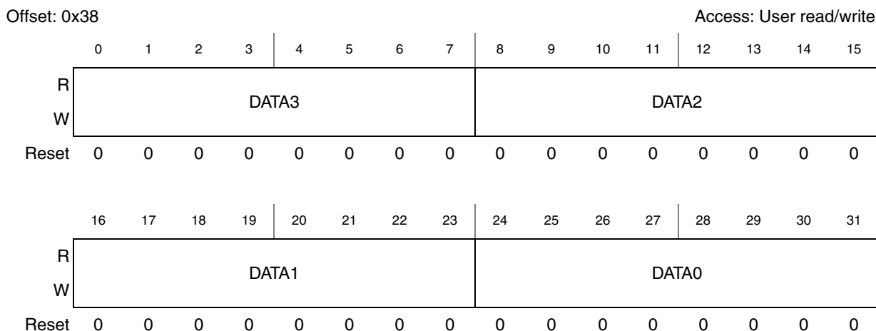
Figure 229. Buffer data register least significant (BDRL)
