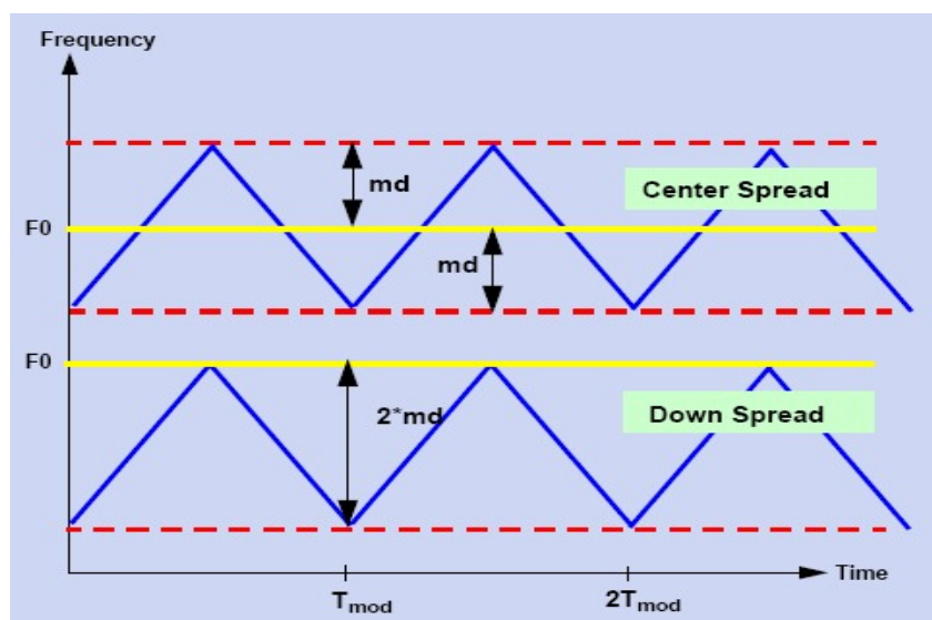
Figure 31. Frequency modulation
