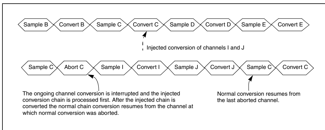
Figure 381. Injected sample/conversion sequence
