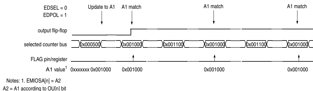
Figure 334. SAOC example with EDPOL value being transferred to the output flip-flop
