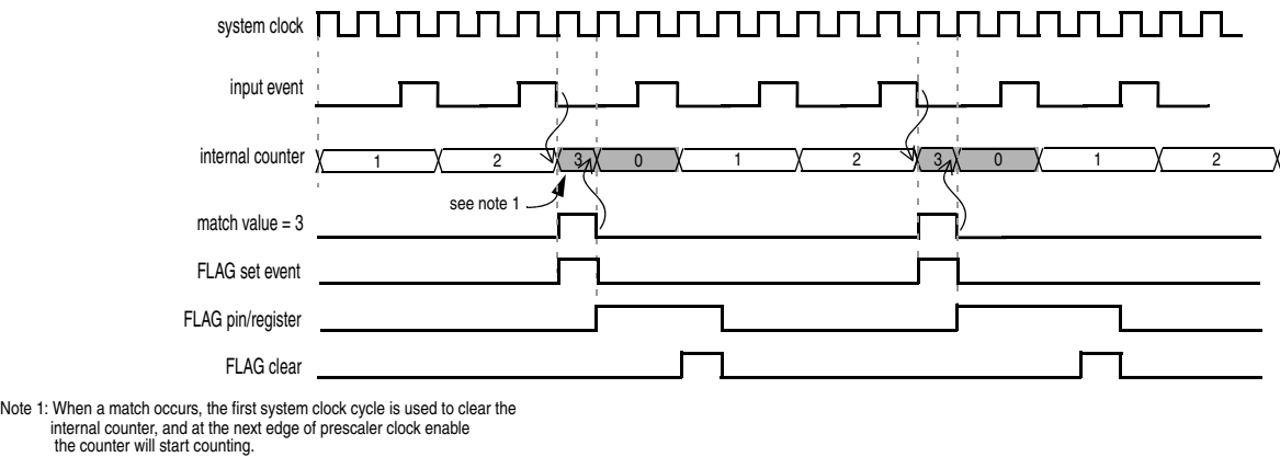
Figure 367. Time base generation with external clock and clear on match start
