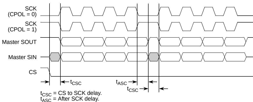
Figure 310. Example of continuous transfer ( CPHA = 1 , CONT = 1 )
