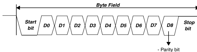
Figure 212. UART mode 9-bit data frame
