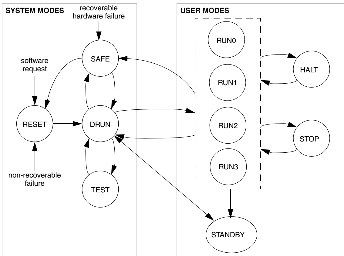
Figure 69. MC_ME Mode Diagram
