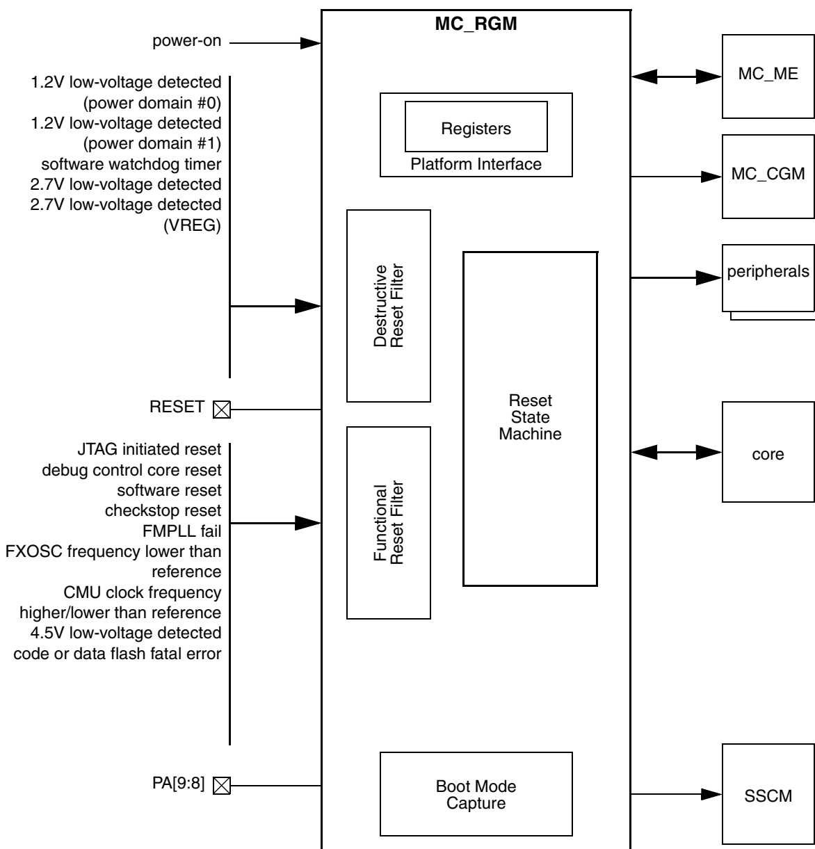
Figure 72. MC_RGM block diagram
