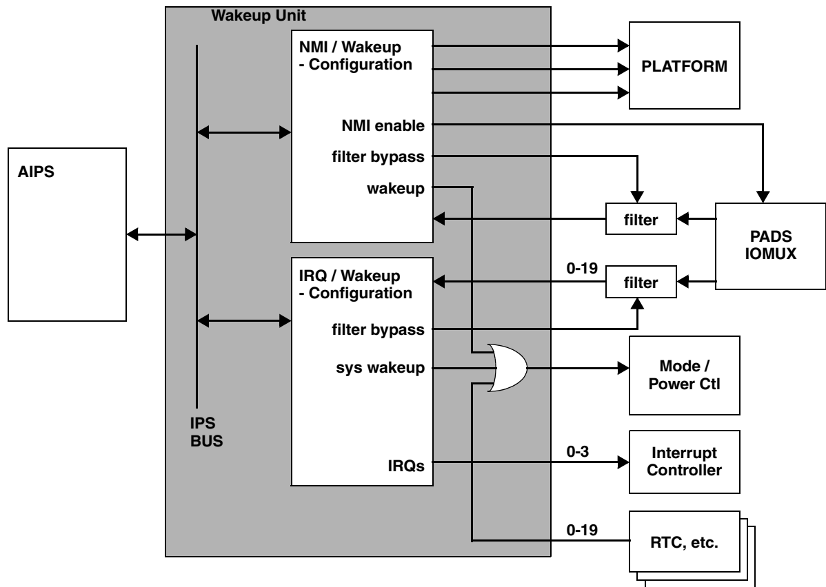
Figure 88. WKPU block diagram
