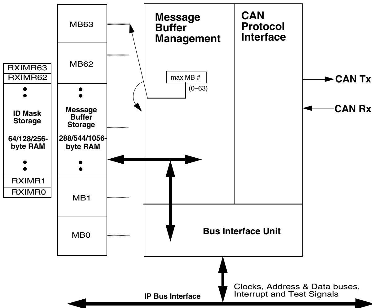
Figure 273. FlexCAN block diagram
