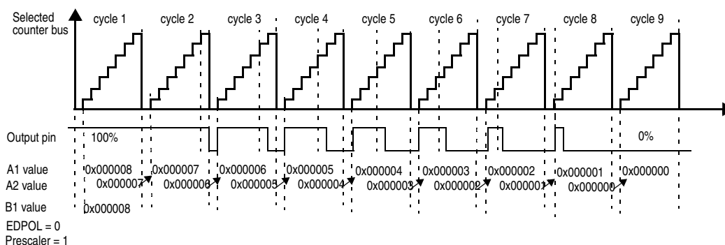
Figure 360. OPWMB mode from 100% to 0% duty cycle
