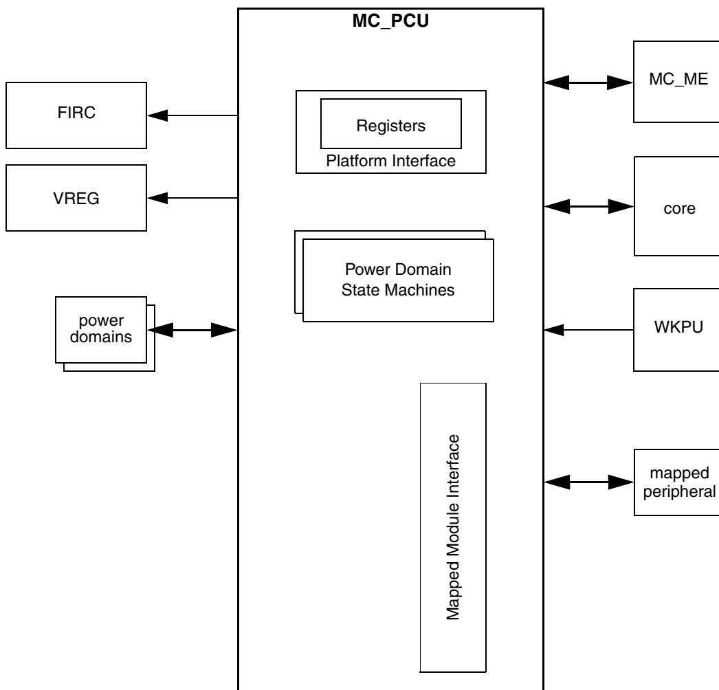
Figure 82. MC_PCU Block Diagram
