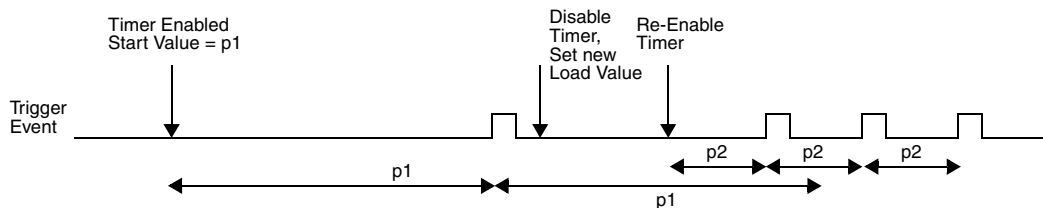
Figure 377. Modifying running timer period
