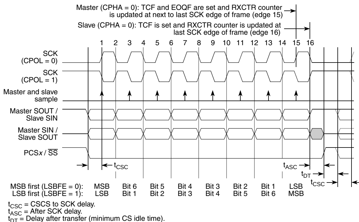
Figure 305. DSPI transfer timing diagram (MTFE = 0, CPHA = 0, FMSZ = 8)
