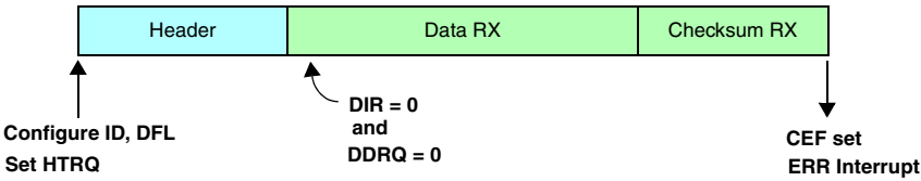
Figure 257. Programming consideration: master node, receiver, checksum error
