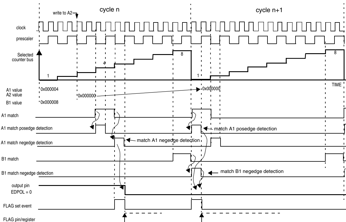
Figure 359. OPWMB mode with 0% duty cycle
