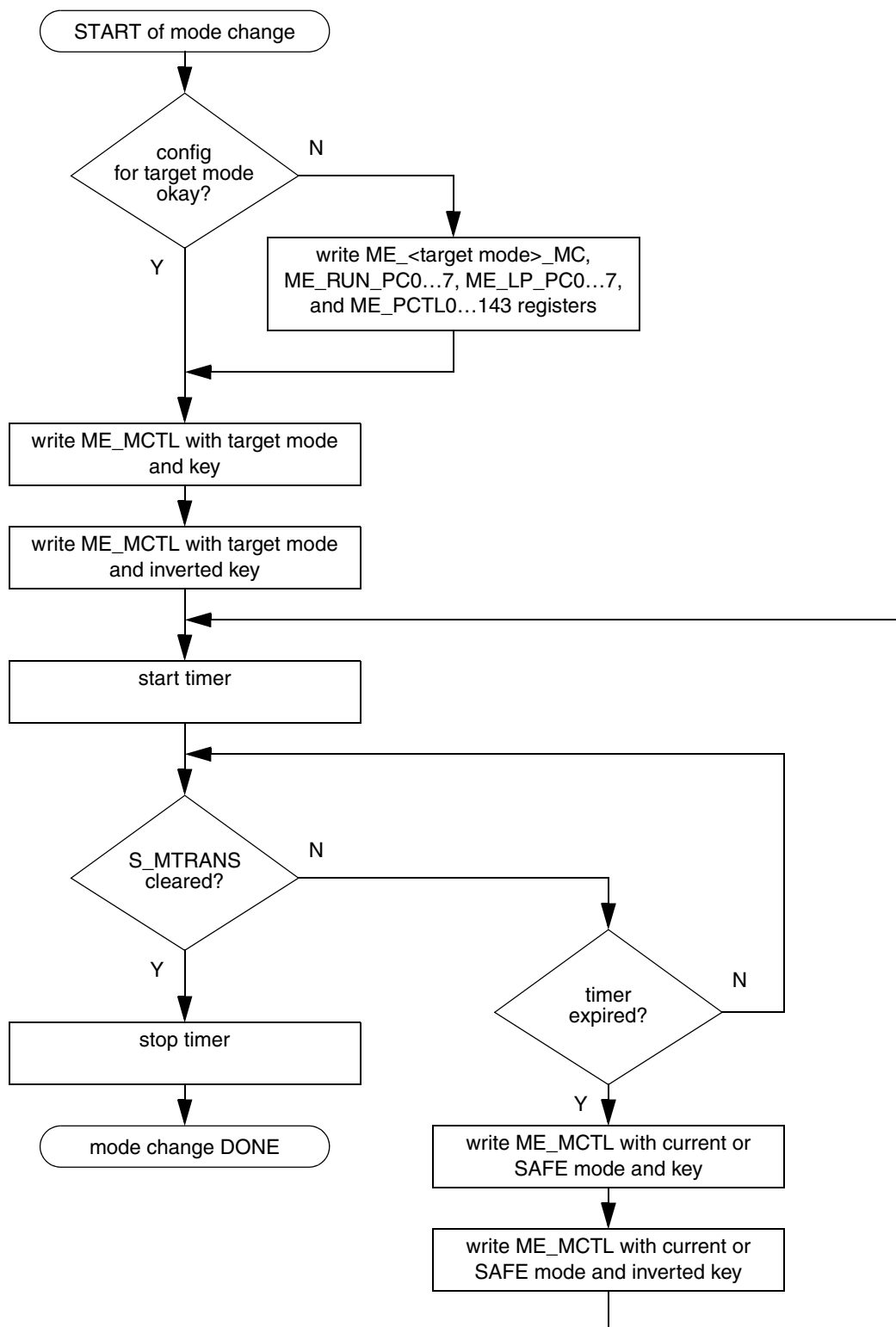
Figure 71. MC_ME Application Example Flow Diagram
