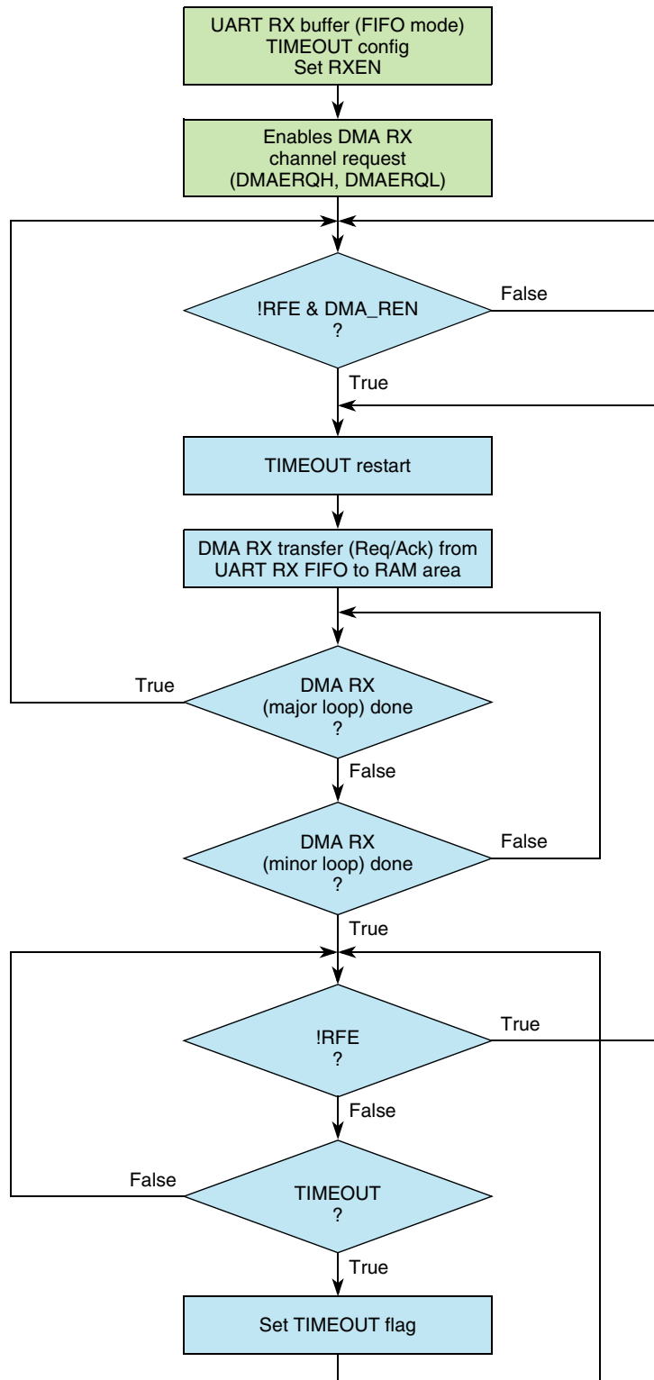
Figure 251. FSM to control the DMA RX interface (UART node)
