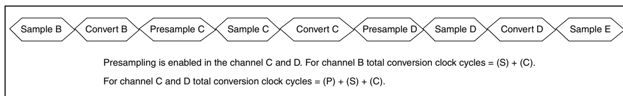
Figure 383. Presampling sequence
