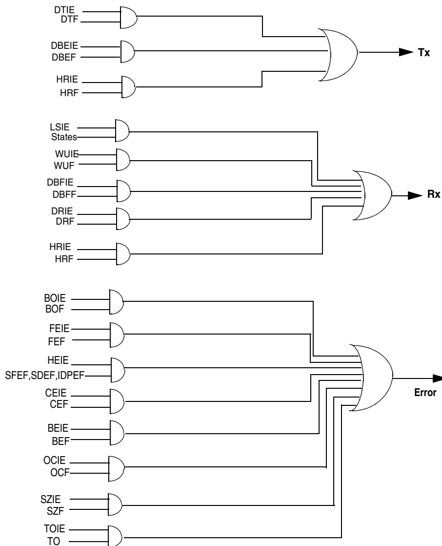
Figure 253. Interrupt diagram
