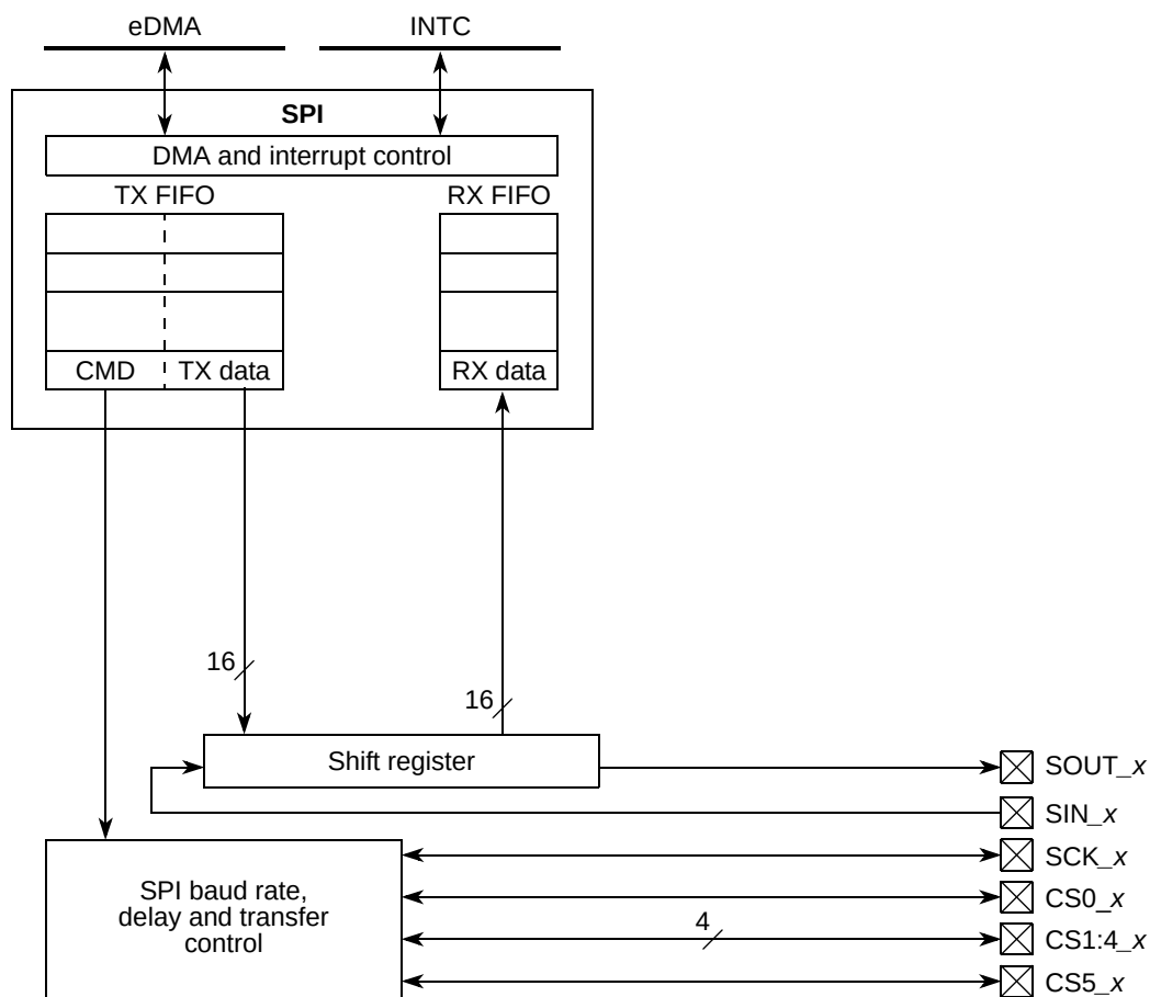
Figure 290. DSPI block diagram
