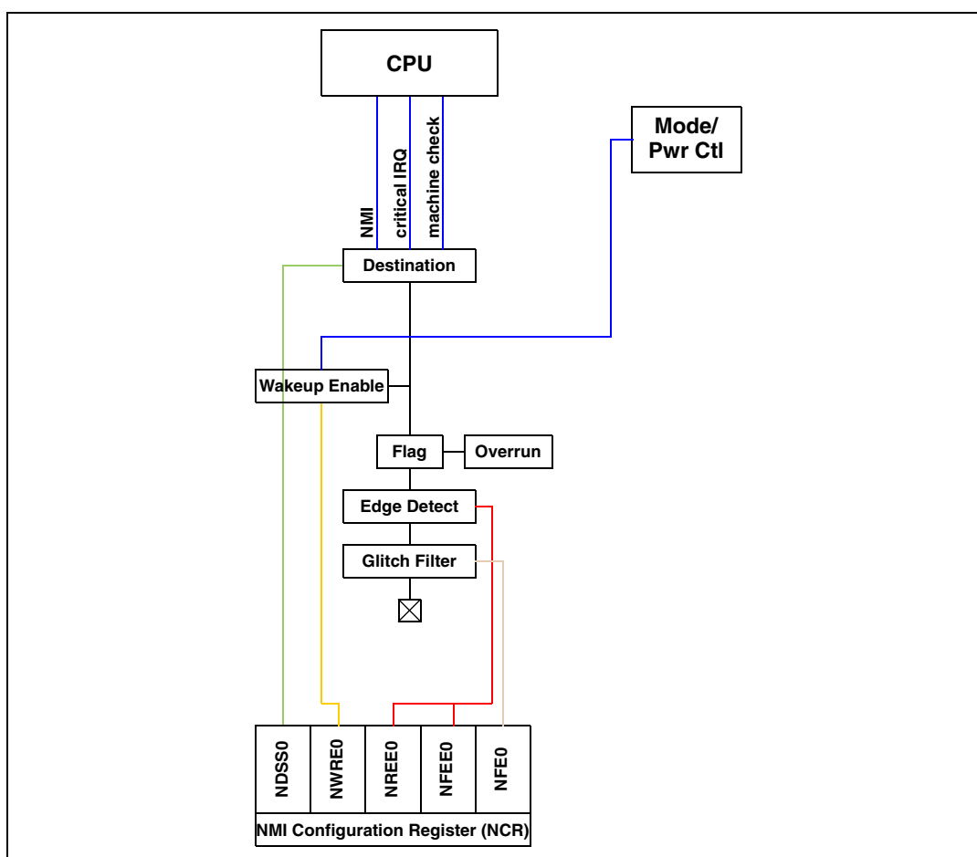
Figure 98. NMI pad diagram
