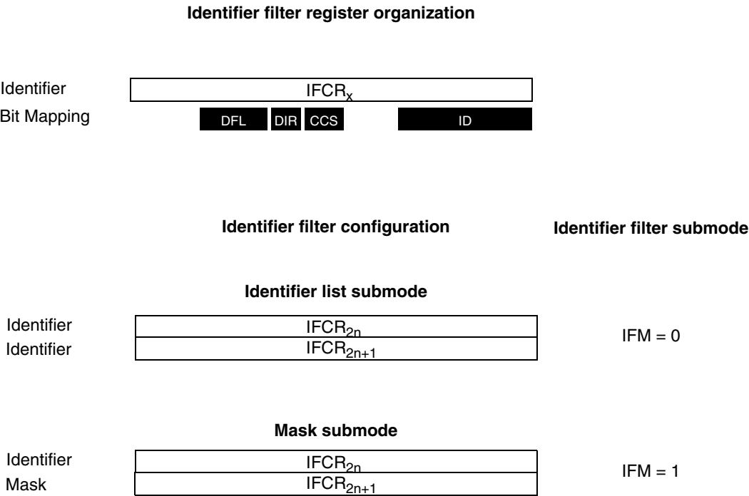
Figure 206. Filter configuration - register organization
