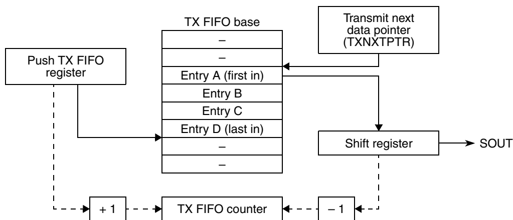
Figure 314. TX FIFO pointers and counter
