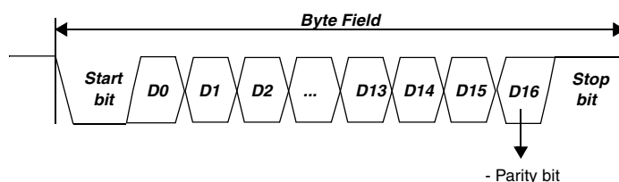
Figure 214. UART mode 17-bit data frame
