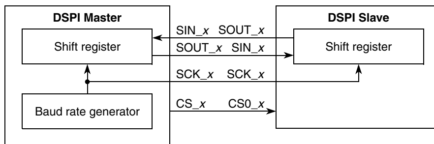
Figure 301. SPI serial protocol overview
