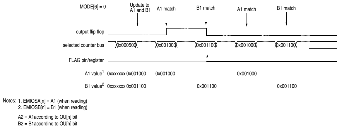
Figure 341. Double action output compare with FLAG set on the second match
