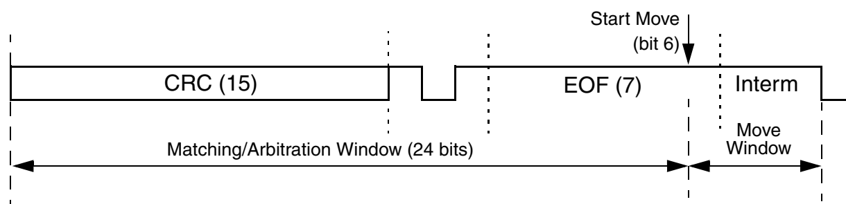
Figure 289. Arbitration, Match and Move Time Windows
