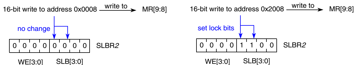
Figure 476. Enable Locking Via Mirror Module Space (Area #3)
