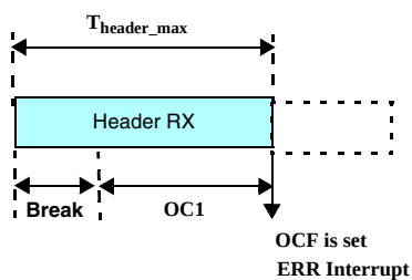
Figure 271. Programming consideration: header timeout
