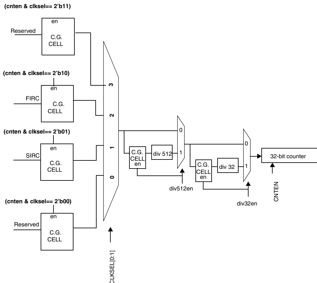
Figure 101. Clock gating for RTC clocks
