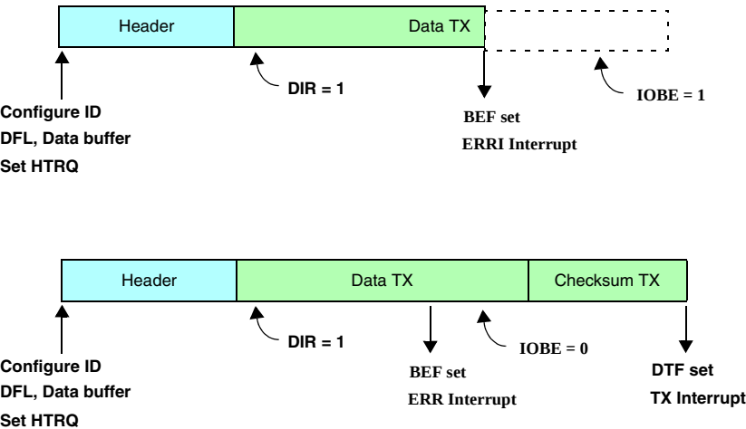
Figure 256. Programming consideration: master node, transmitter, bit error
