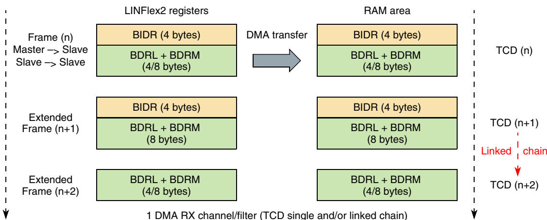
Figure 246. TCD chain memory map (slave node, RX mode)
