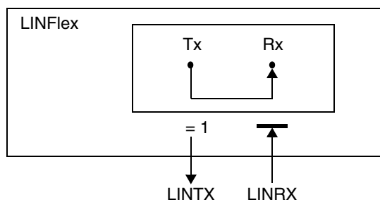
Figure 170. LINFlex in self test mode
