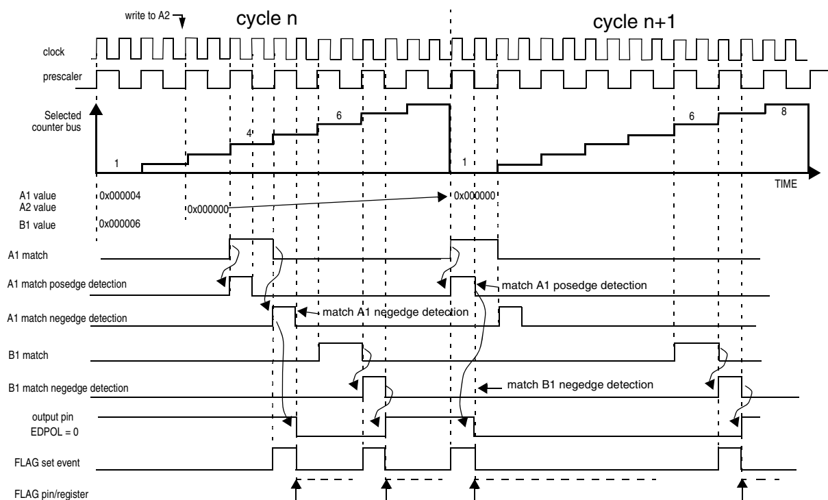
Figure 358. OPWMB mode matches and flags
