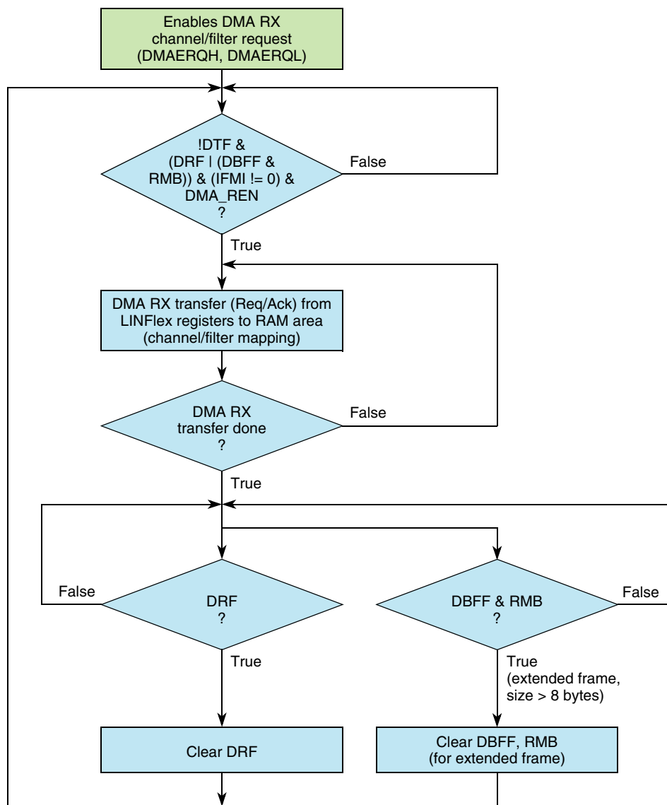
Figure 247. FSM to control the DMA RX interface (slave node)
