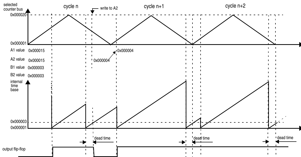
Figure 357. OPWMCB with 100% Duty Cycle (A1 = 4 and B1 = 3)
