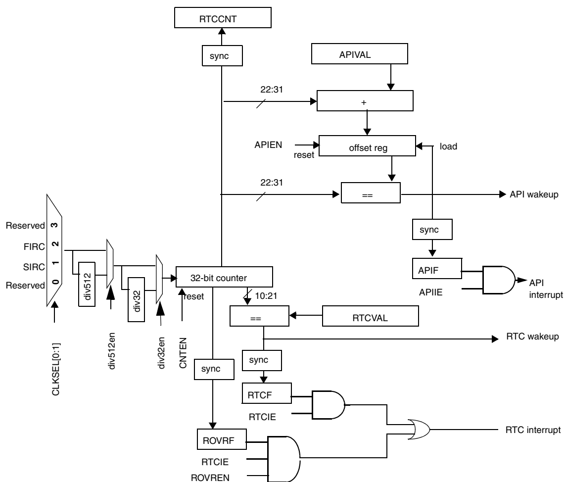
Figure 100. RTC/API block diagram
