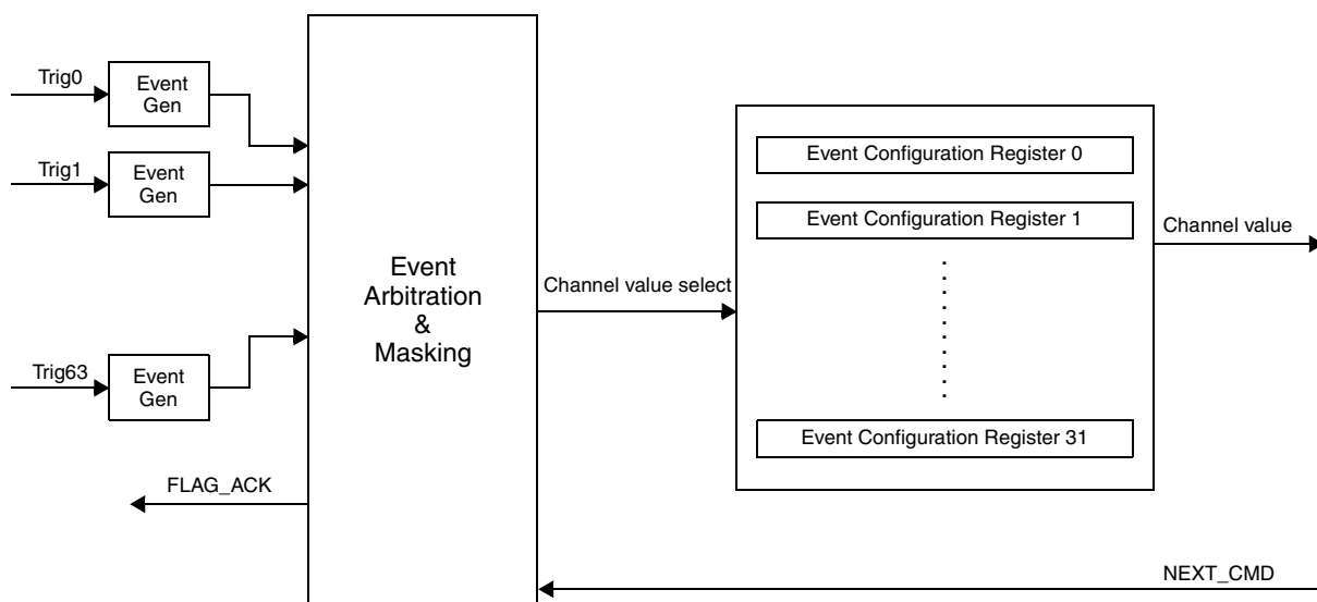
Figure 424. Cross Triggering Unit block diagram
