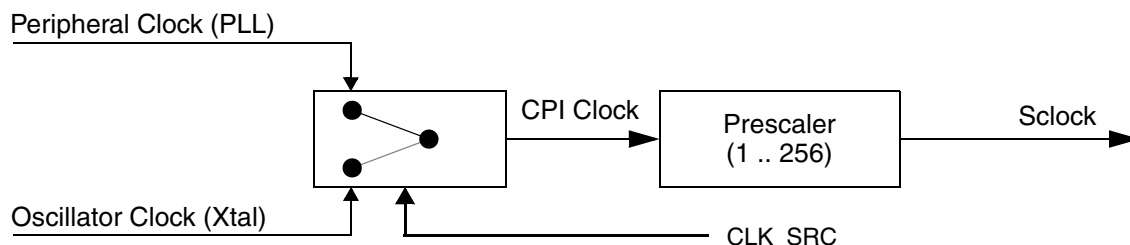
Figure 287. CAN Engine Clocking Scheme
