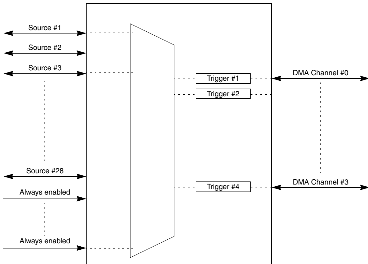
Figure 133. DMA_MUX channel 0-3 block diagram
