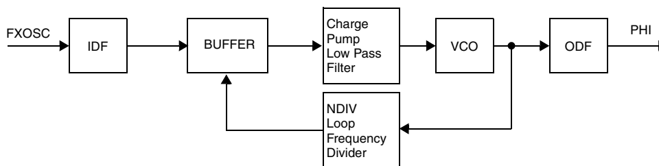
Figure 27. FMPLL block diagram
