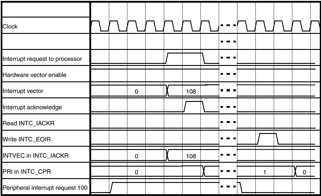
Figure 148. Hardware vector mode handshaking timing diagram
