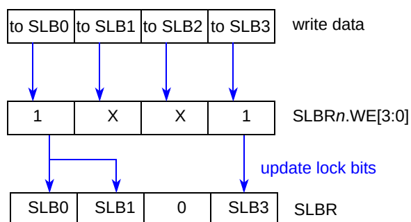
Figure 475. Change Lock Settings for Mixed Protection
