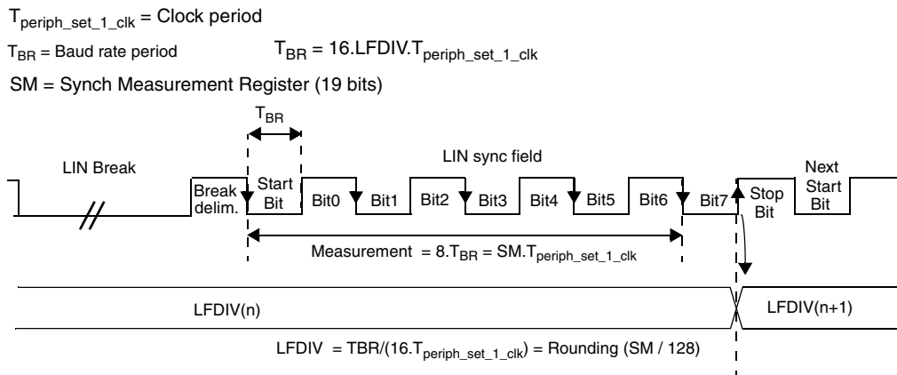
Figure 208. LIN sync field measurement
