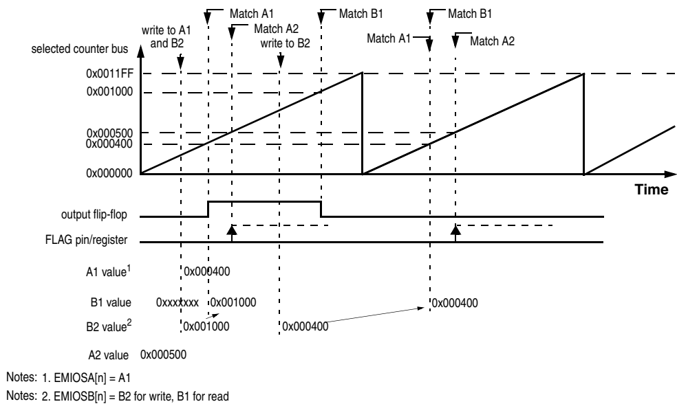
Figure 362. OPWMT with 0% Duty Cycle
