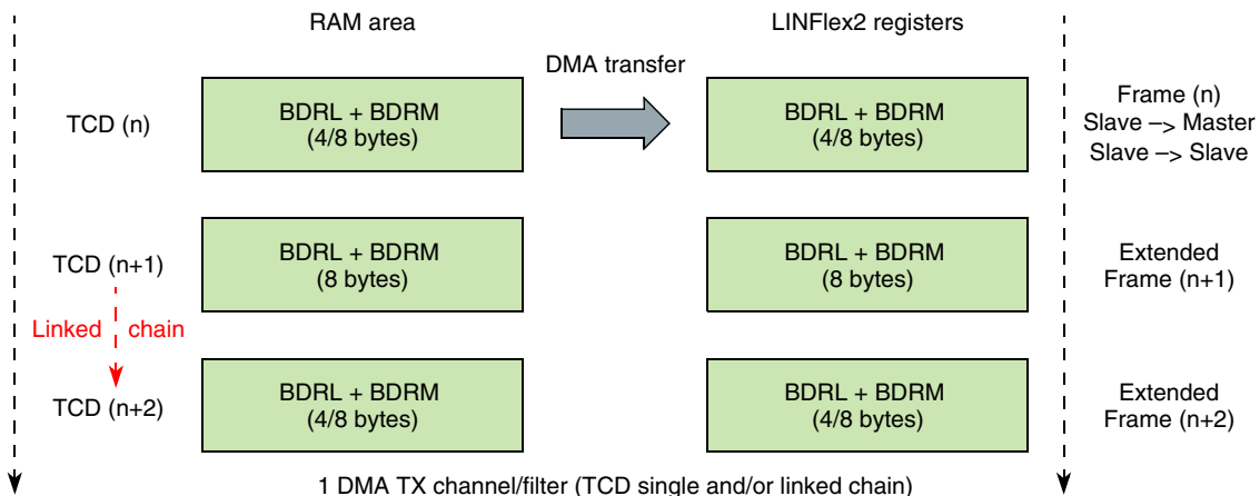
Figure 244. TCD chain memory map (slave node, TX mode)
