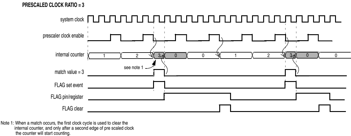
Figure 368. Time base generation with internal clock and clear on match start
