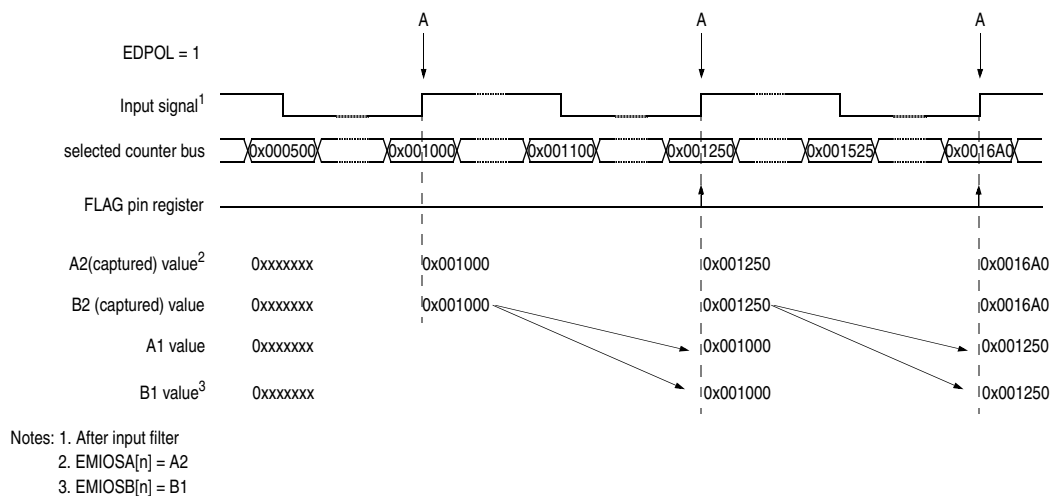
Figure 339. Input period measurement example
