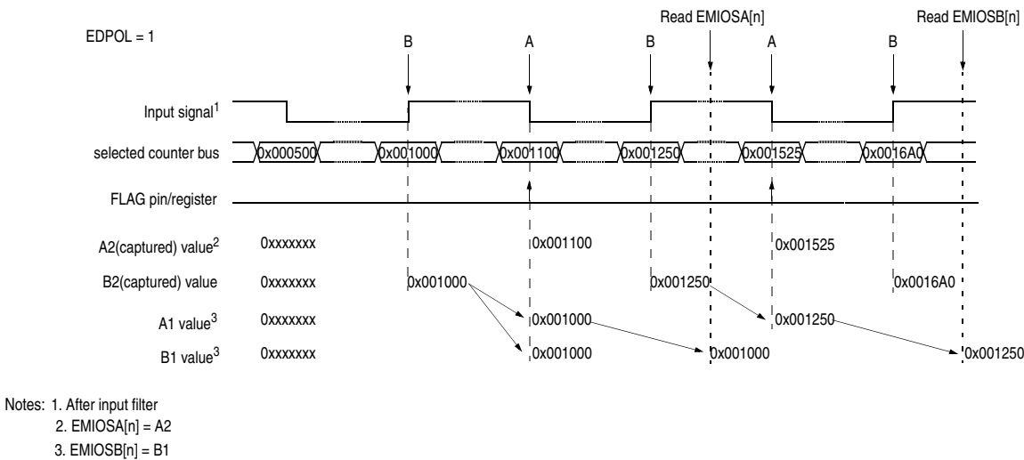
Figure 338. B1 and A1 updates at EMIOSA[n] and EMIOSB[n] reads
