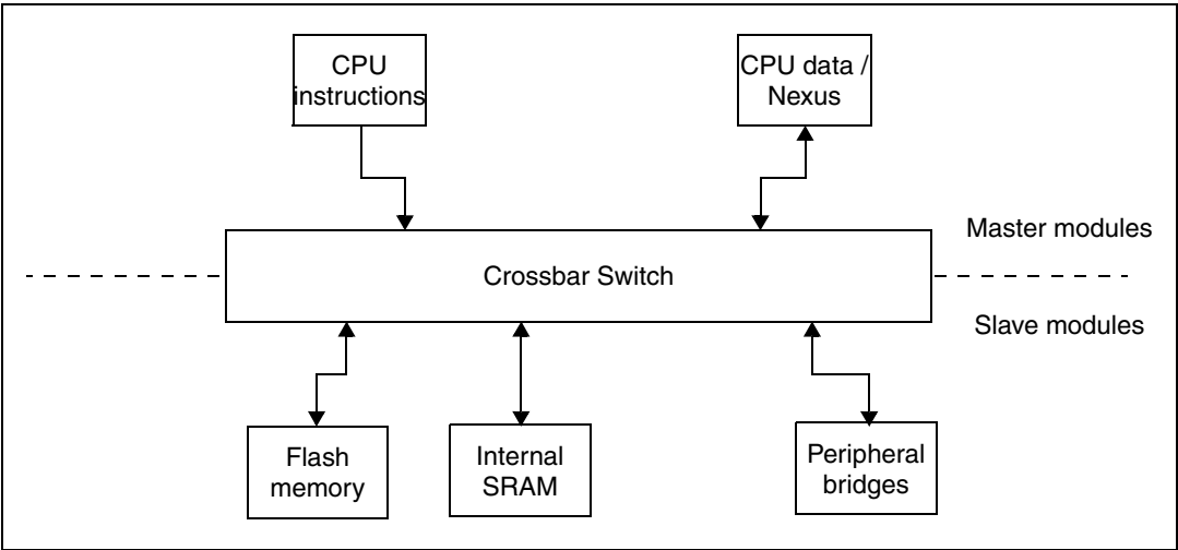
Figure 149. XBAR block diagram
