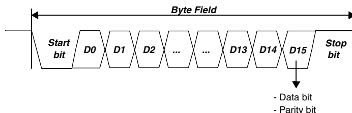
Figure 213. UART mode 16-bit data frame
