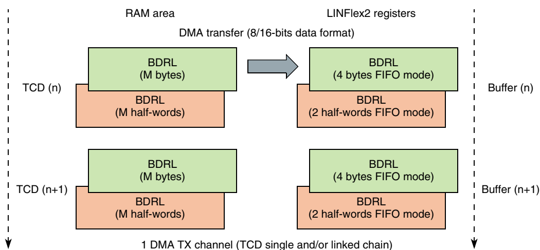
Figure 248. TCD chain memory map (UART node, TX mode)
