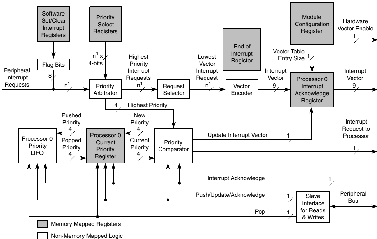
Figure 137. INTC block diagram
