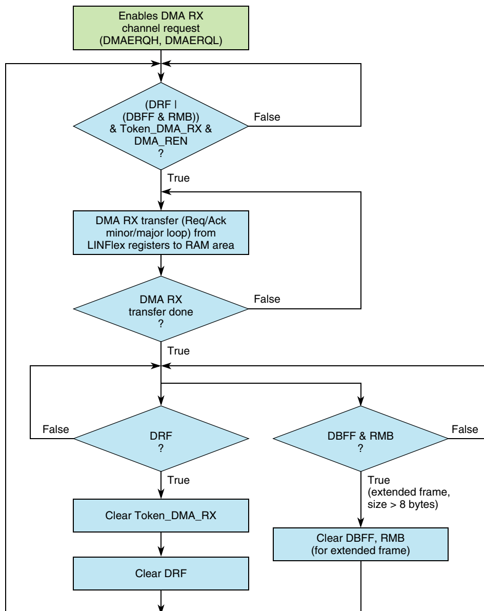
Figure 243. FSM to control the DMA RX interface (master node)
