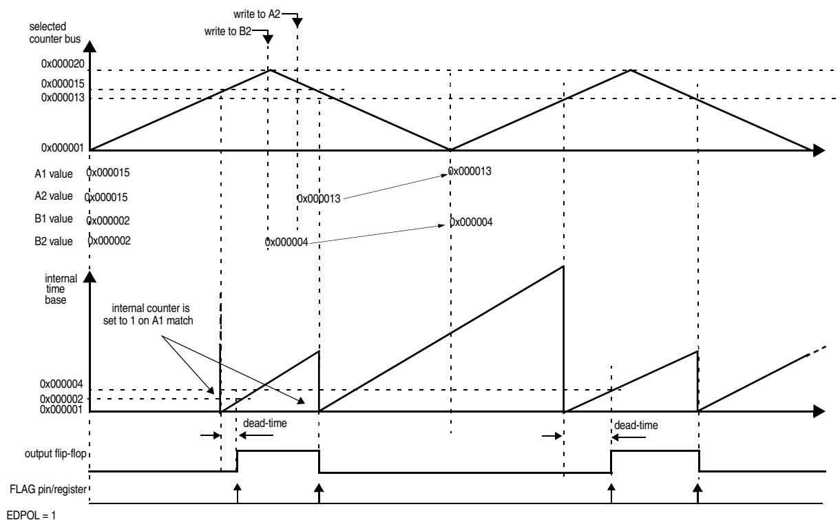
Figure 355. OPWMCB with lead dead time insertion
