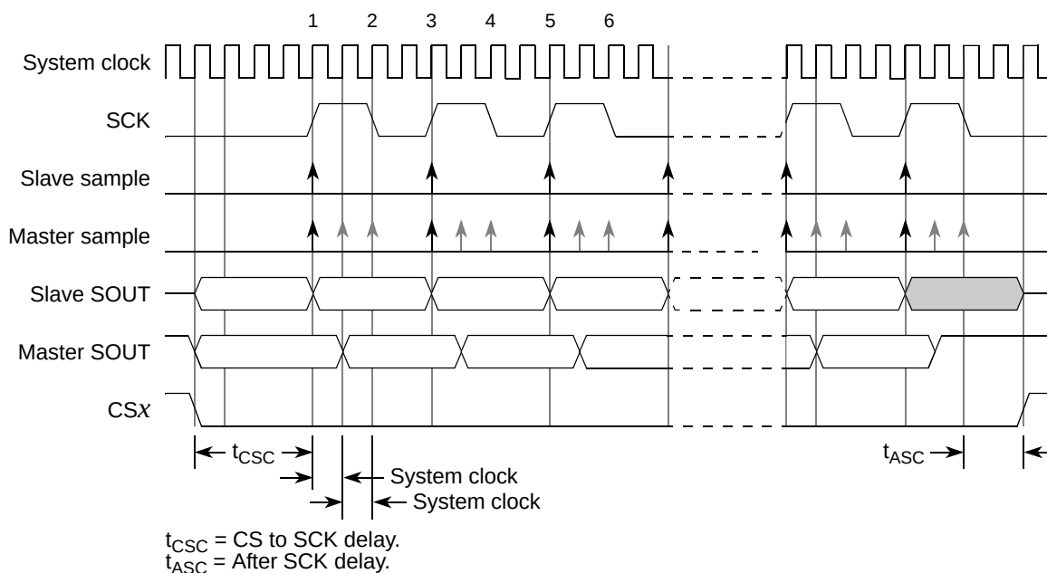
Figure 307. DSPI modified transfer format (MTFE = 1, CPHA = 0, f_{SCK} = f_{SYS} / 4 )
