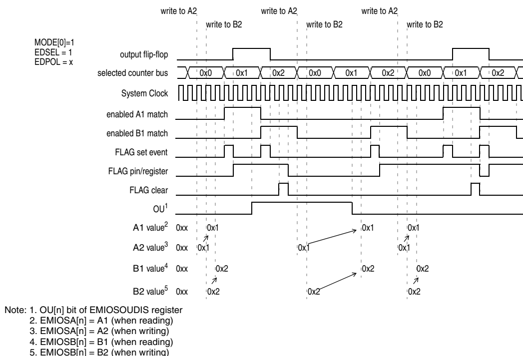
Figure 343. DAOC with transfer disabling example
