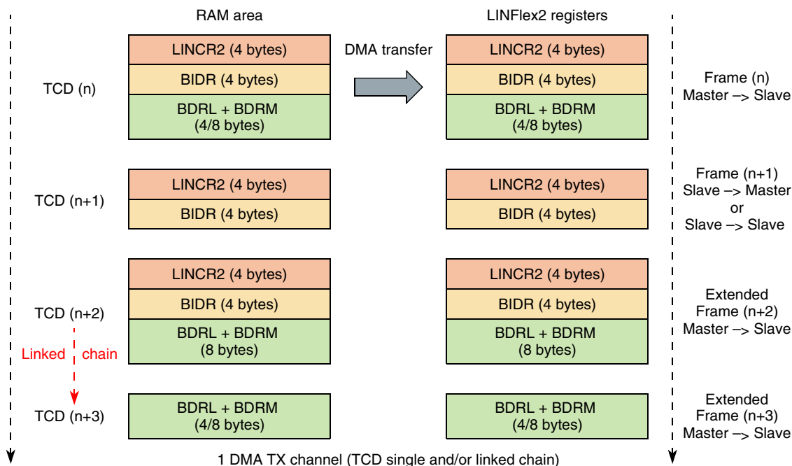
Figure 240. TCD chain memory map (master node, TX mode)
