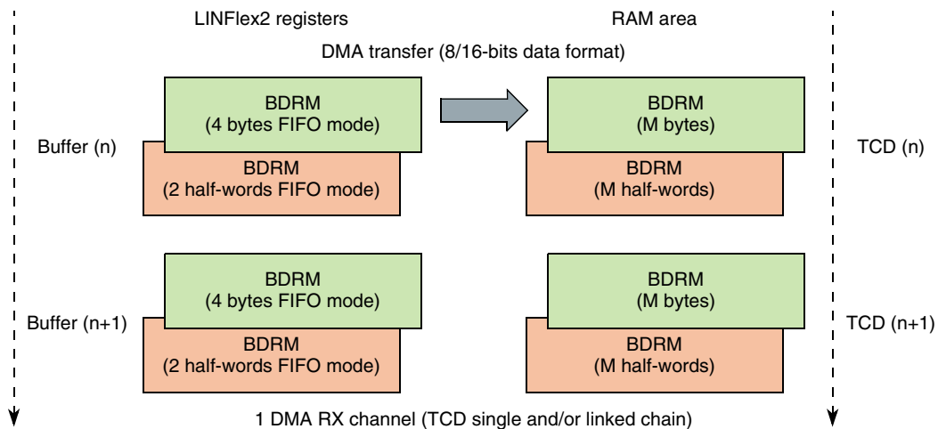
Figure 250. TCD chain memory map (UART node, RX mode)
