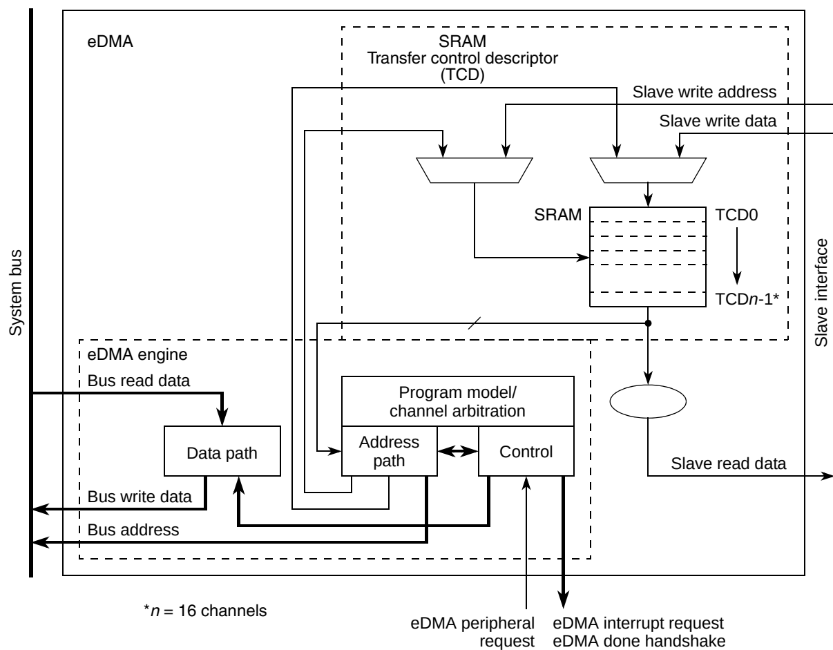
Figure 127. eDMA operation, part 2
