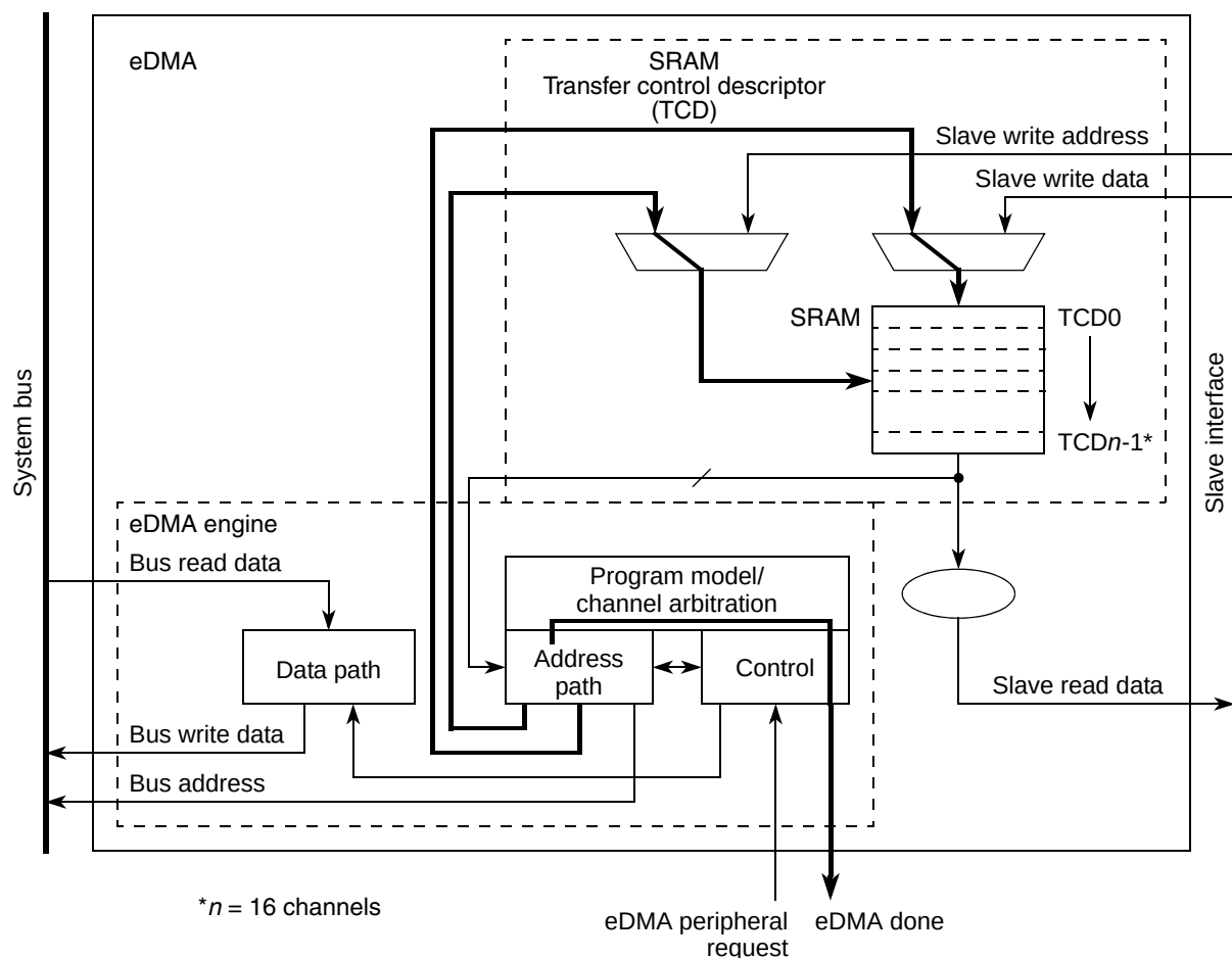
Figure 128. eDMA operation, part 3
