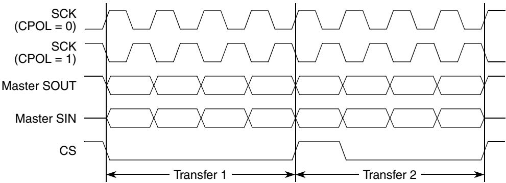
Figure 313. Continuous SCK timing diagram (CONT=1)
