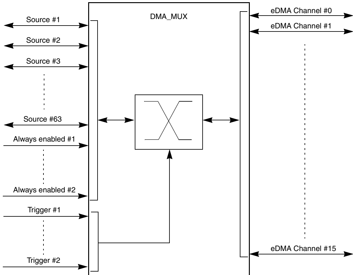
Figure 131. DMA_MUX block diagram
