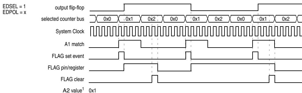
Figure 336. SAOC example with flag behavior
