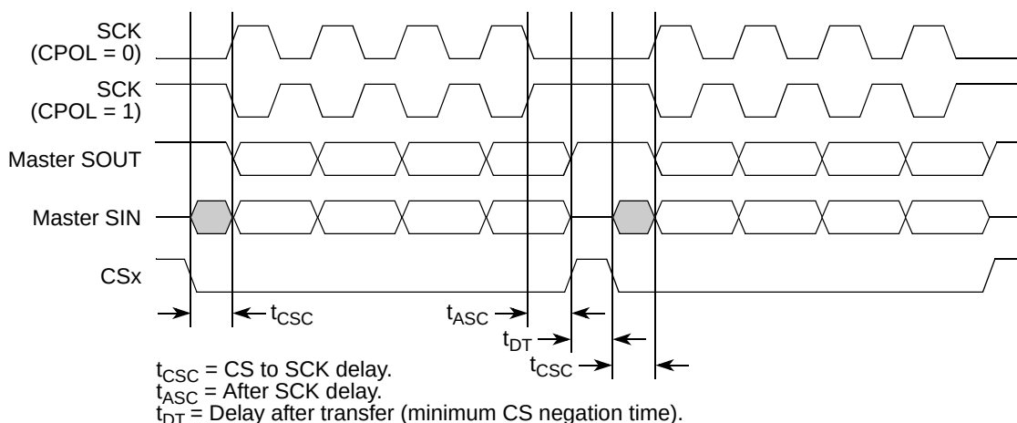
Figure 309. Example of non-continuous format ( CPHA = 1 , CONT = 0 )
