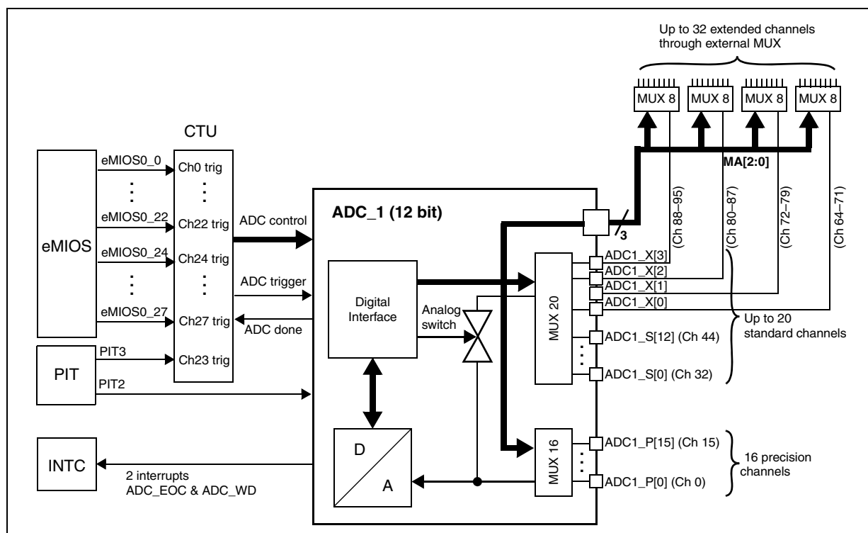
Figure 379. ADC implementation
