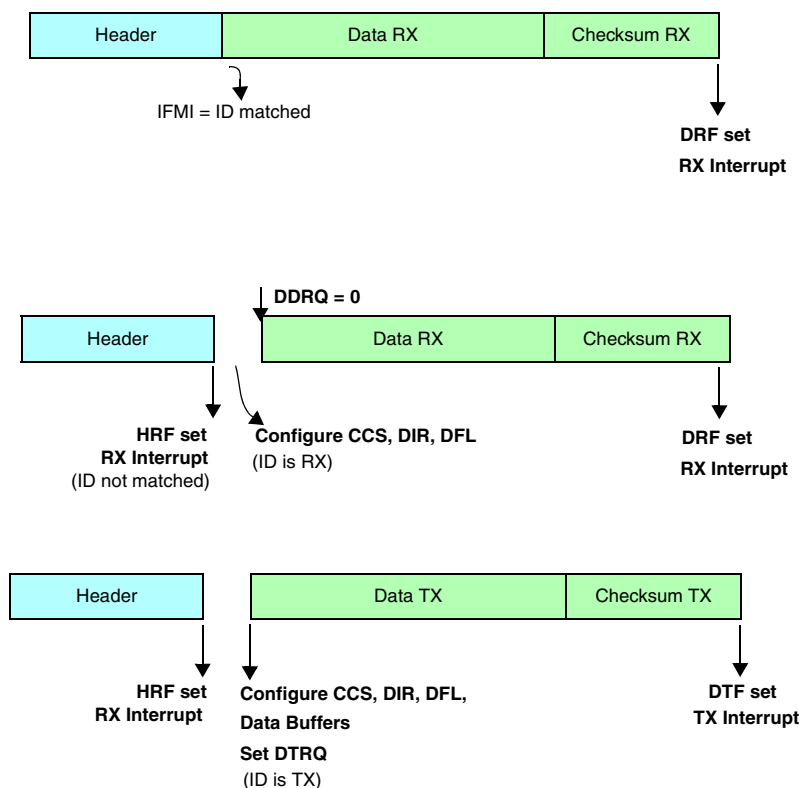
Figure 266. Programming consideration: slave node, RX filter, BF is set
