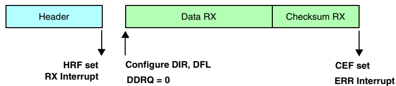
Figure 261. Programming consideration: slave node, receiver, no filters, checksum error
