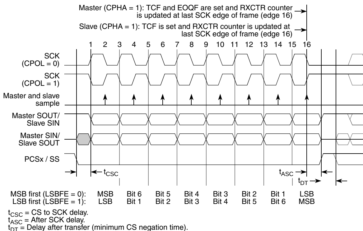
Figure 306. DSPI transfer timing diagram (MTFE = 0, CPHA = 1, FMSZ = 8)
