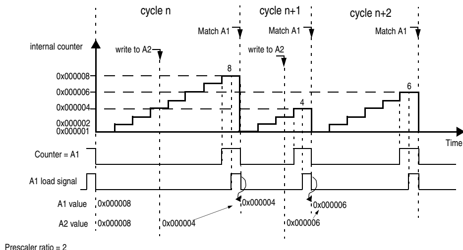
Figure 348. MCB Mode A1 Register Update in Up Counter mode
