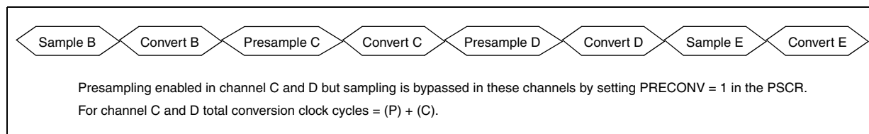
Figure 384. Presampling sequence with PRECONV = 1
