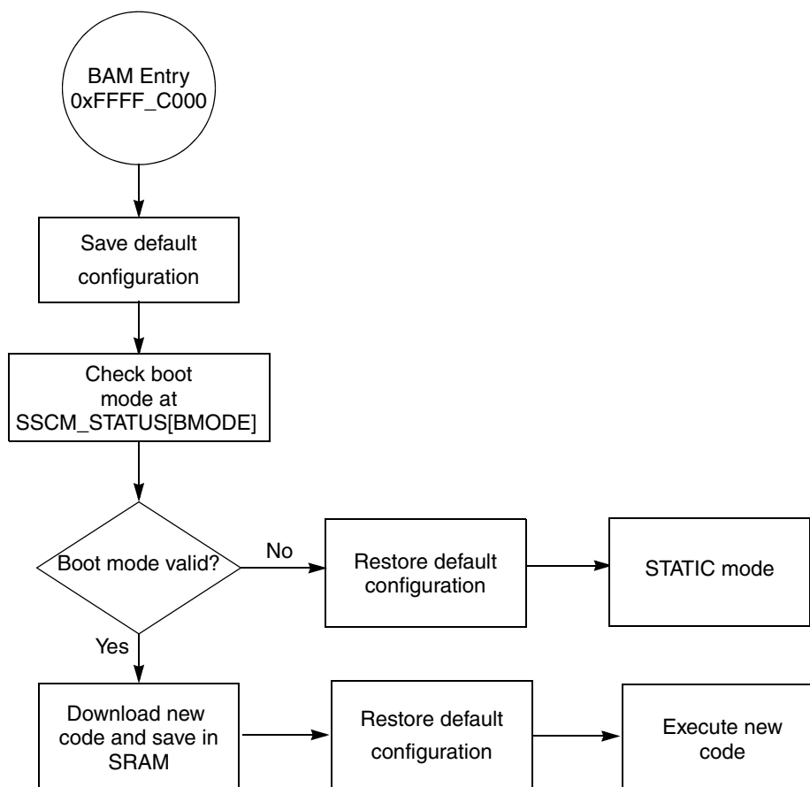
Figure 10. BAM logic flow
