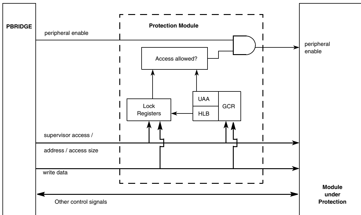
Figure 468. Register Protection block diagram
