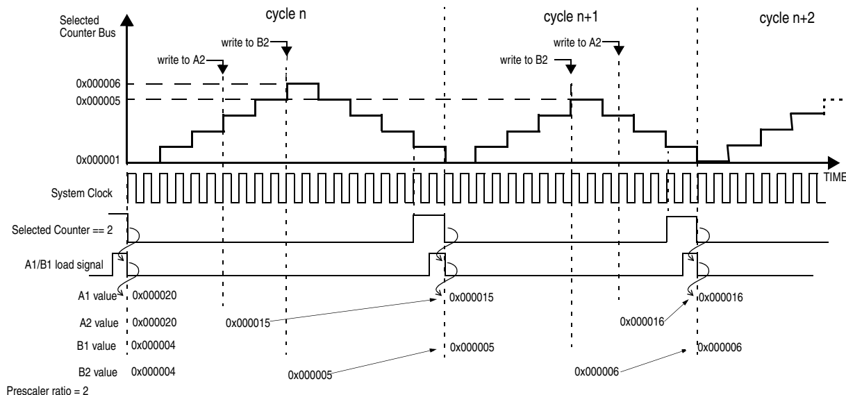
Figure 354. OPWMCB A1 and B1 registers load
