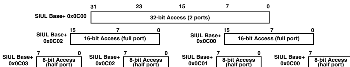
Figure 164. Data Port example arrangement showing configuration for different port width accesses
