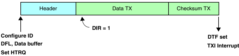
Figure 254. Programming consideration: master node, transmitter
