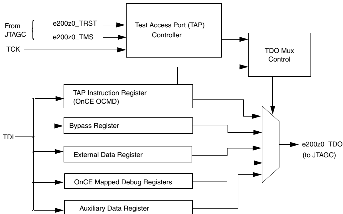
Figure 507. e200z0 OnCE Block Diagram
