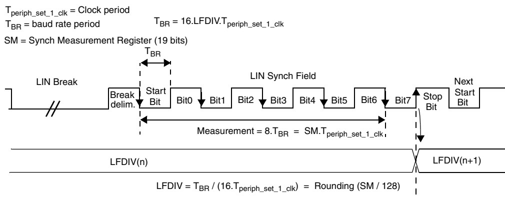
Figure 196. LIN synch field measurement
