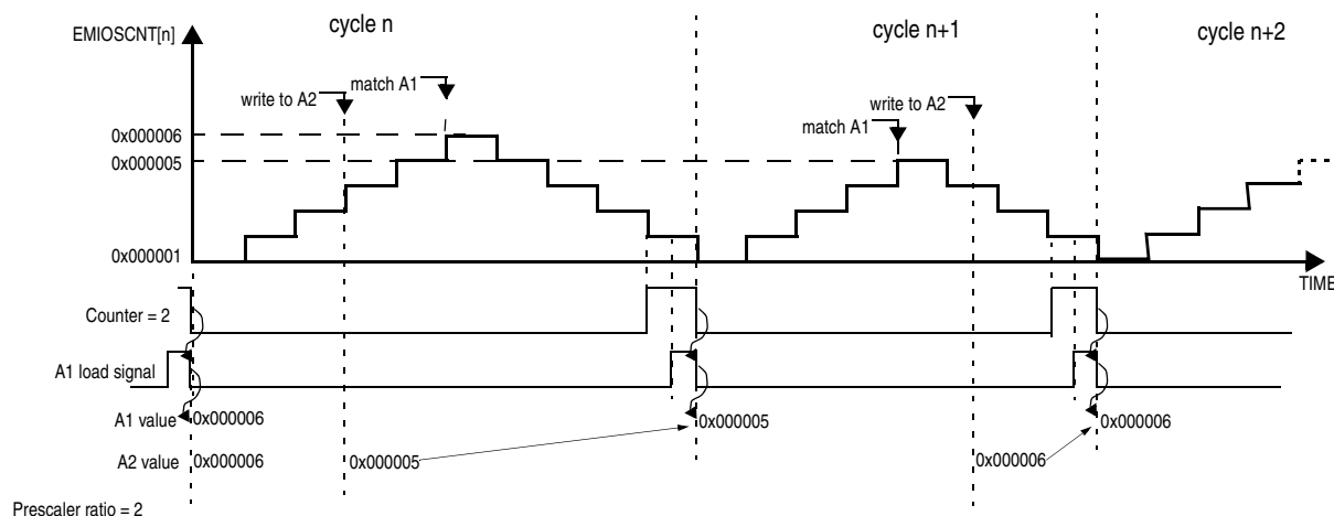
Figure 349. MCB Mode A1 Register Update in Up/Down Counter mode
