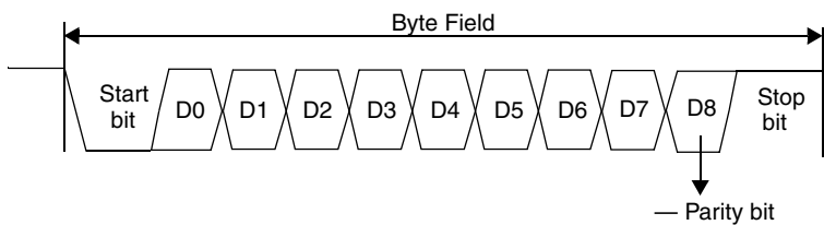
Figure 193. UART mode 9-bit data frame
