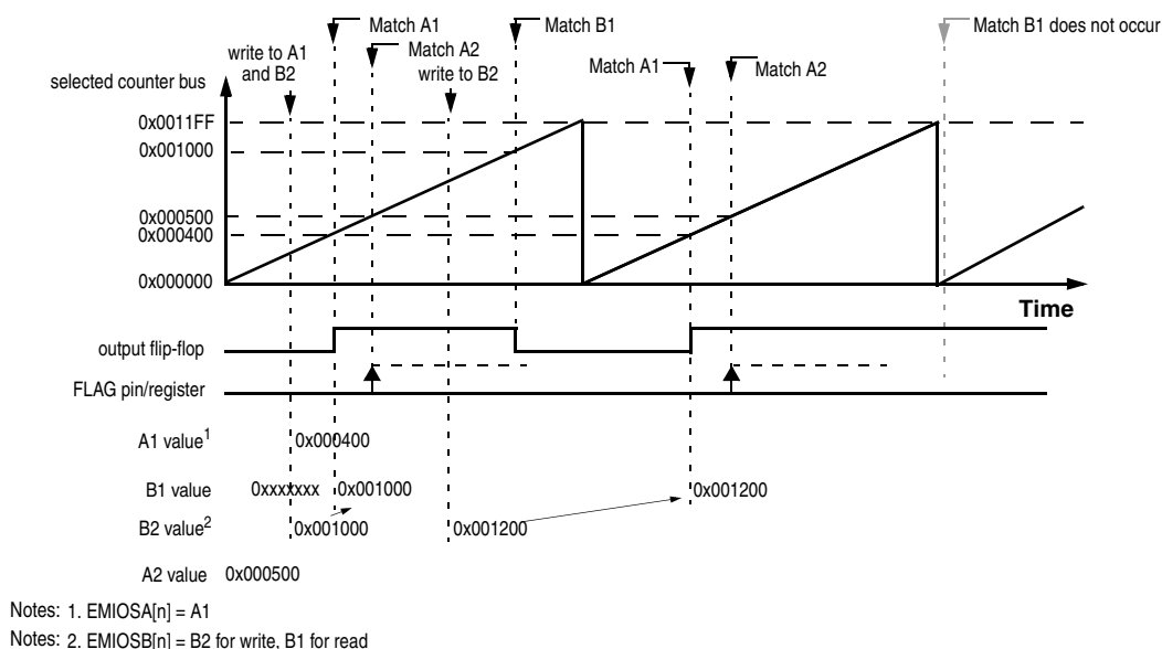
Figure 363. OPWMT with 100% duty cycle
