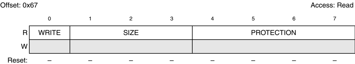
Figure 500. Platform RAM ECC Attributes Register (PREAT)
