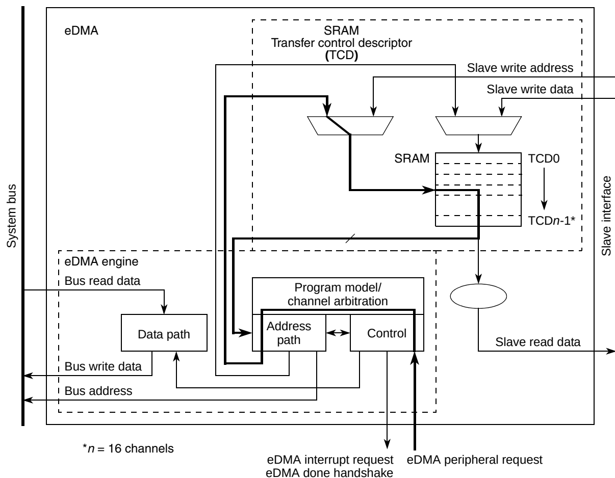
Figure 126. eDMA operation, part 1
