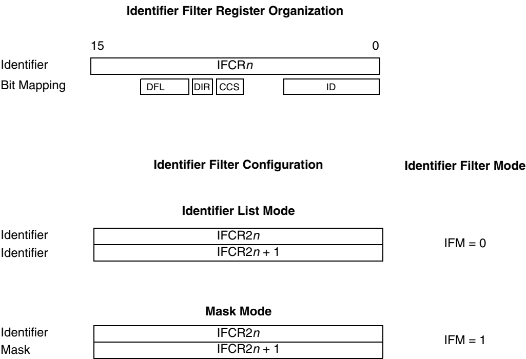
Figure 194. Filter configuration—register organization
