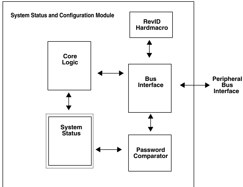
Figure 16. SSCM block diagram
