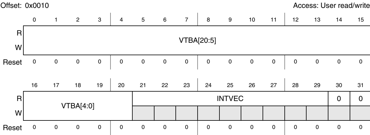
Figure 141. INTC Interrupt Acknowledge Register (INTC_IACKR) when INTC_MCR[VTES] = 1
