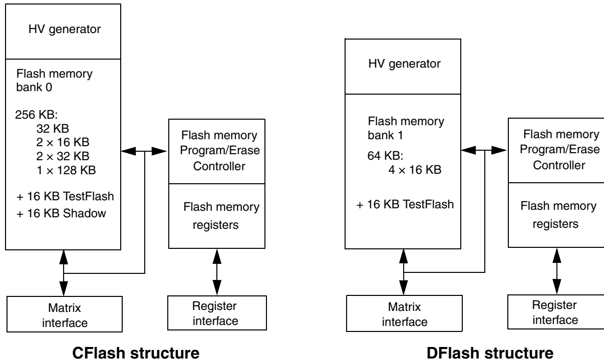
Figure 427. CFlash and DFlash module structures
