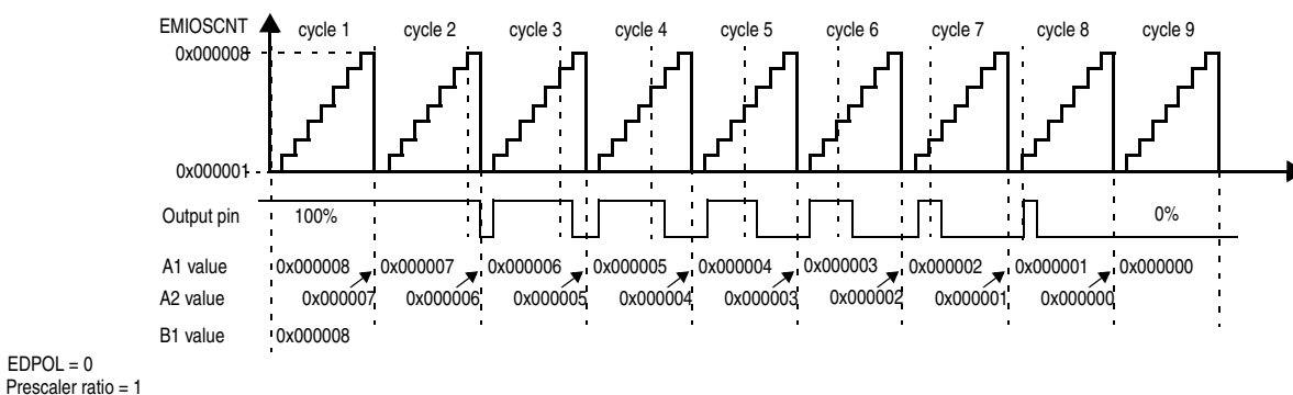
Figure 353. OPWFMB mode from 100% to 0% duty cycle
