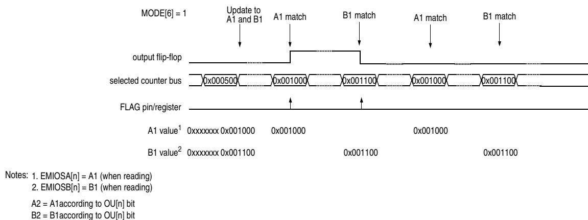
Figure 342. Double action output compare with FLAG set on both matches
