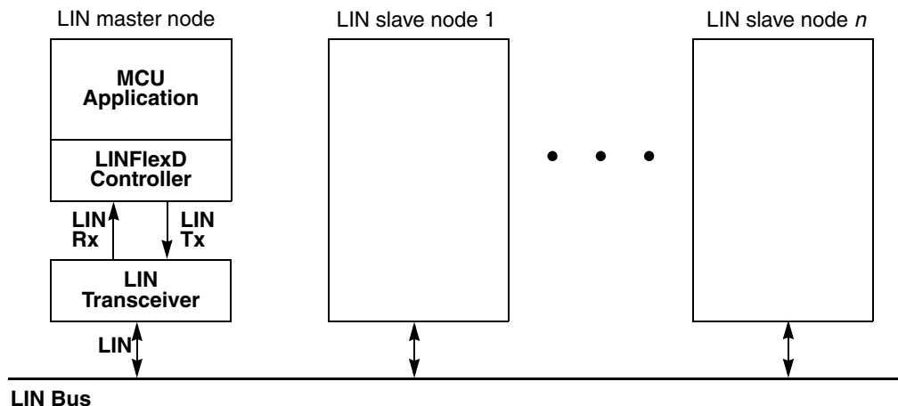
Figure 199. LIN network topology
