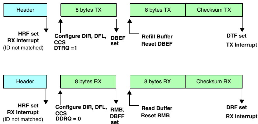
Figure 268. Programming consideration: extended frames
