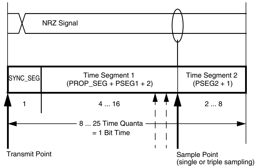
Figure 288. Segments within the Bit Time
