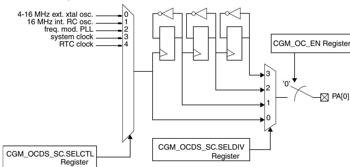
Figure 45. MC_CGM Output Clock Multiplexer and PA[0] Generation
