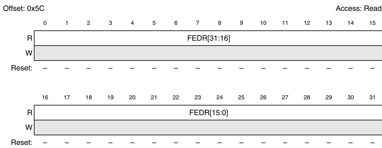
Figure 496. Platform Flash ECC Data Register (PFEDR)
