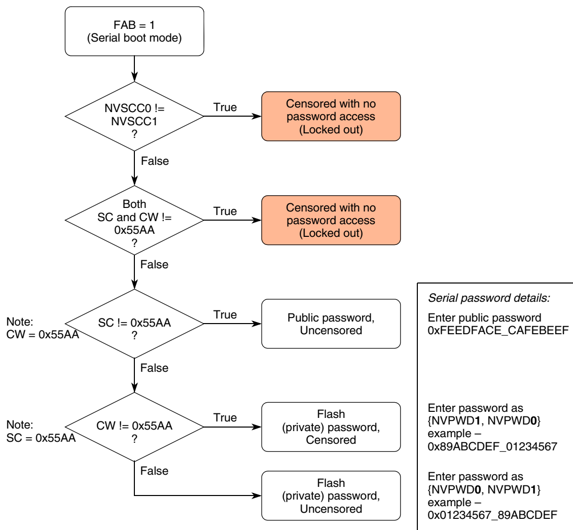
Figure 9. Censorship control in serial boot mode
