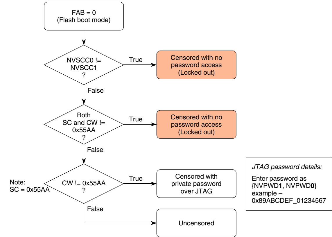
Figure 8. Censorship control in flash memory boot mode
