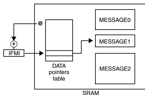
Figure 195. Identifier match index
