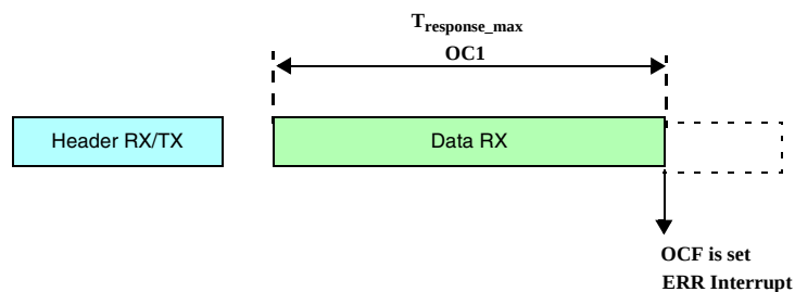
Figure 269. Programming consideration: response timeout
