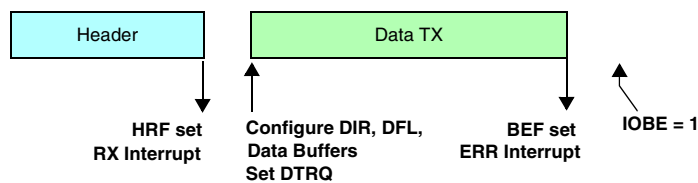
Figure 260. Programming consideration: slave node, transmitter, no filters, bit error
