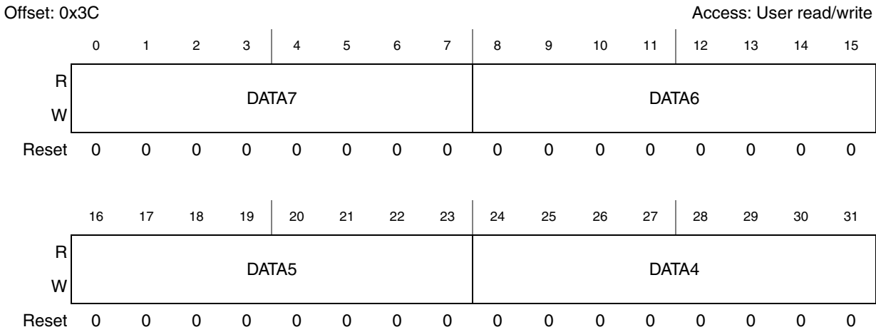
Figure 230. Buffer data register most significant (BDRM)
