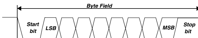
Figure 203. Structure of the data field
