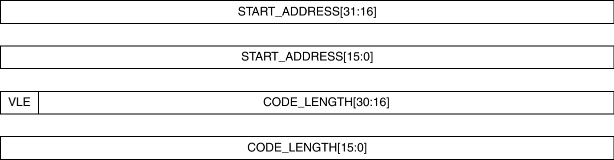
Figure 13. Start address, VLE bit and download size in bytes
