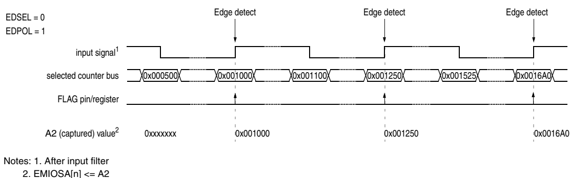
Figure 332. Single action input capture with rising edge triggering example
