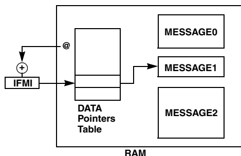
Figure 207. Identifier match index
