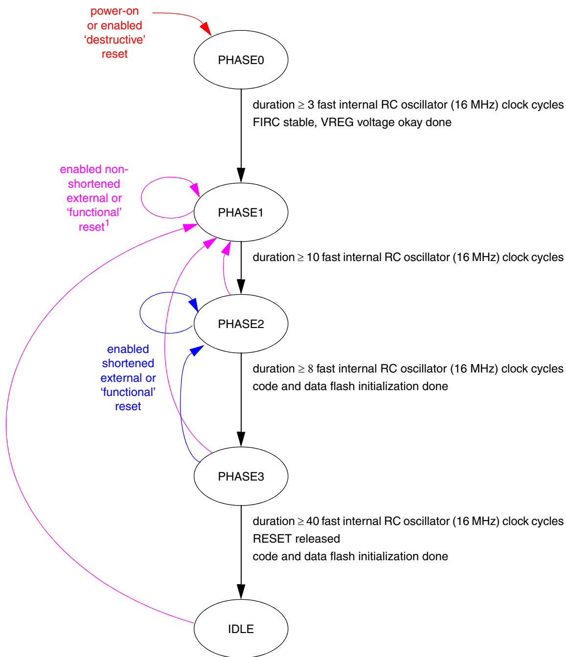
Figure 81. MC_RGM State Machine
