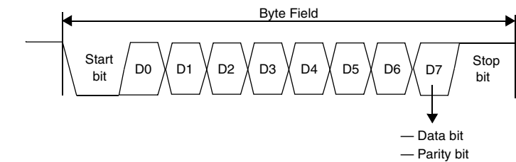
Figure 192. UART mode 8-bit data frame
