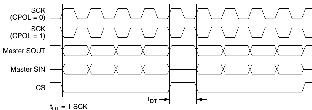
Figure 312. Continuous SCK timing diagram (CONT= 0)
