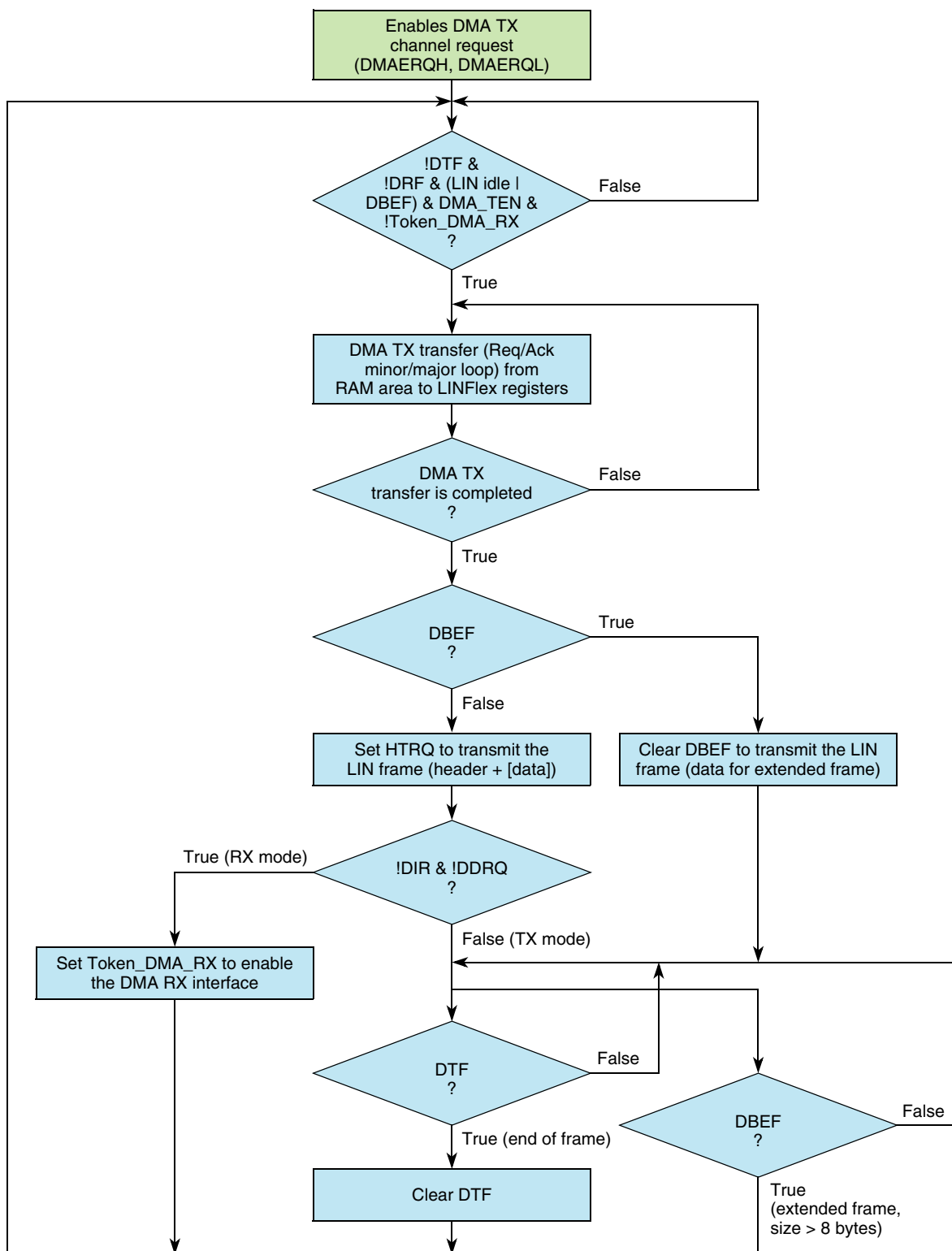
Figure 241. FSM to control the DMA TX interface (master node)
