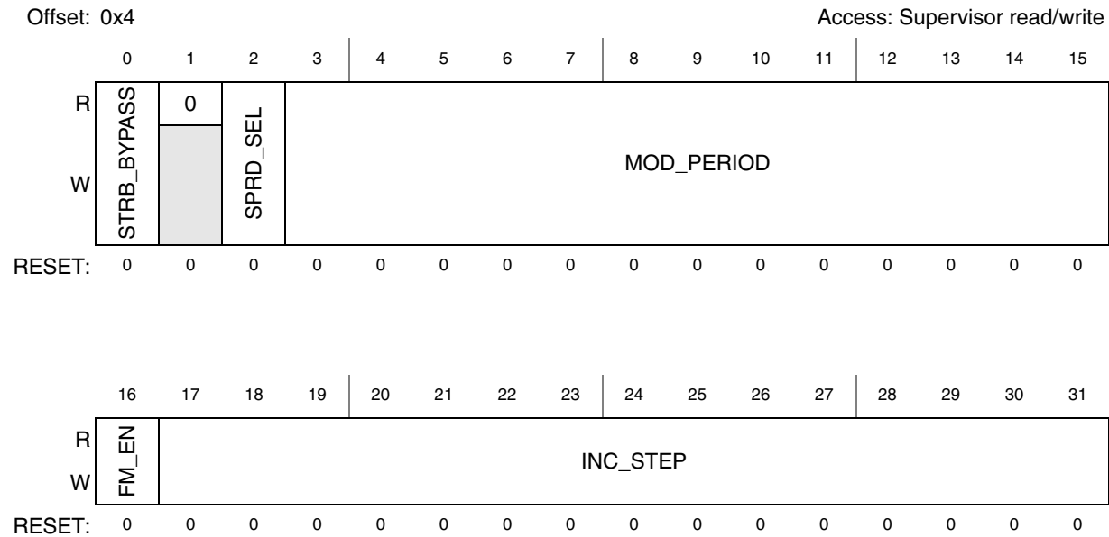
Figure 29. Modulation Register (MR)
