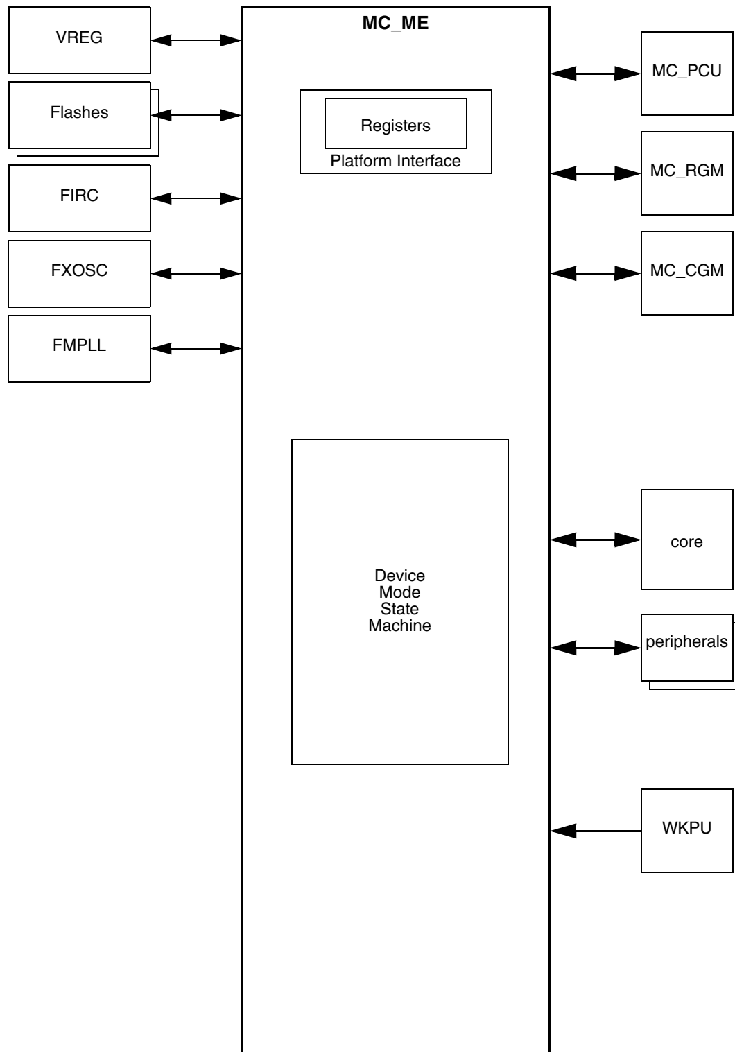
Figure 46. MC_ME Block Diagram
