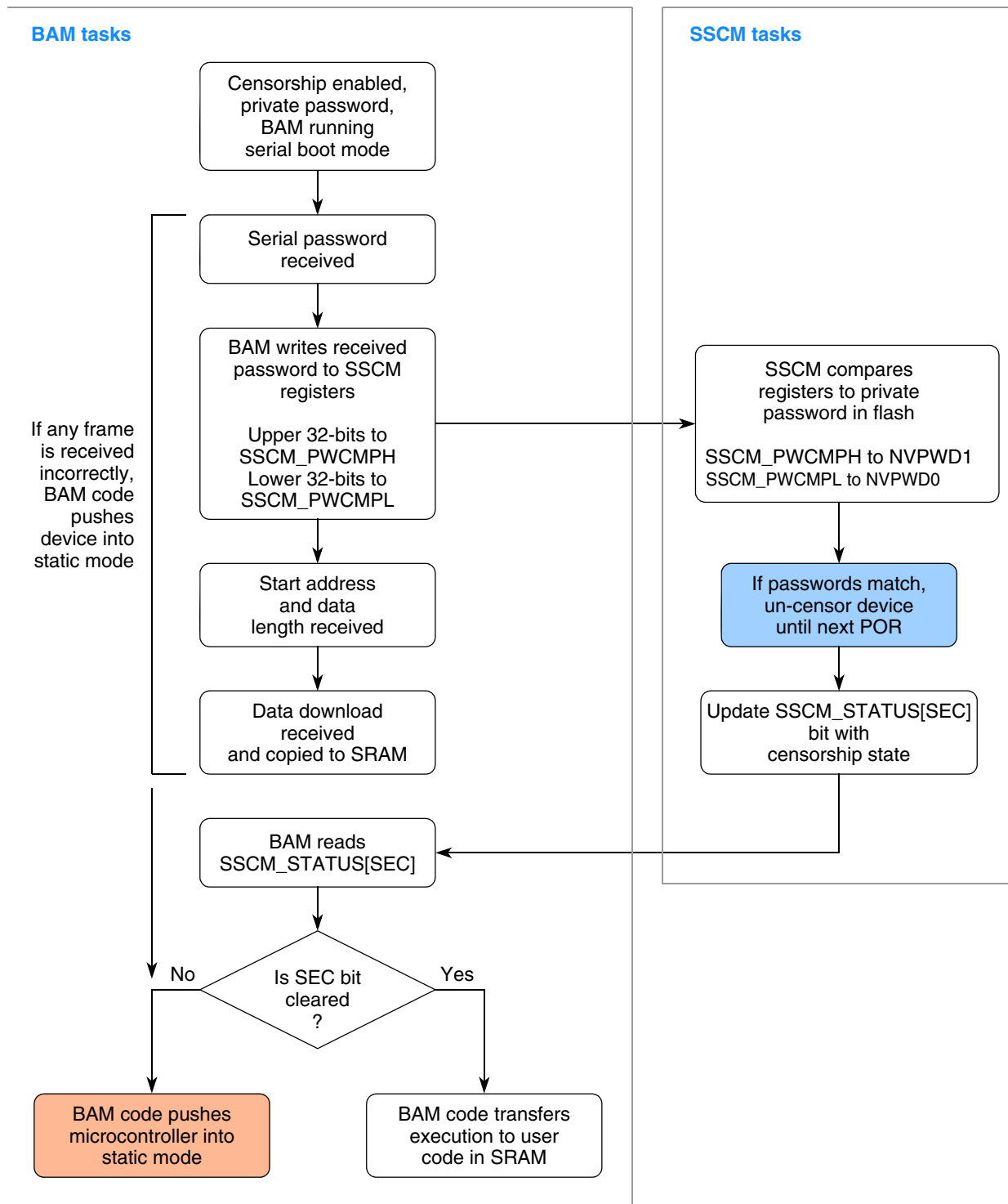
Figure 12. BAM serial boot mode flow for censorship enabled and private password
