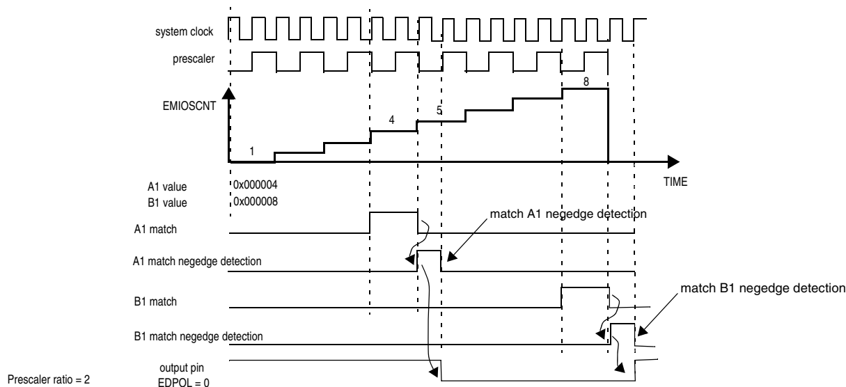
Figure 350. OPWFMB A1 and B1 match to Output Register Delay
