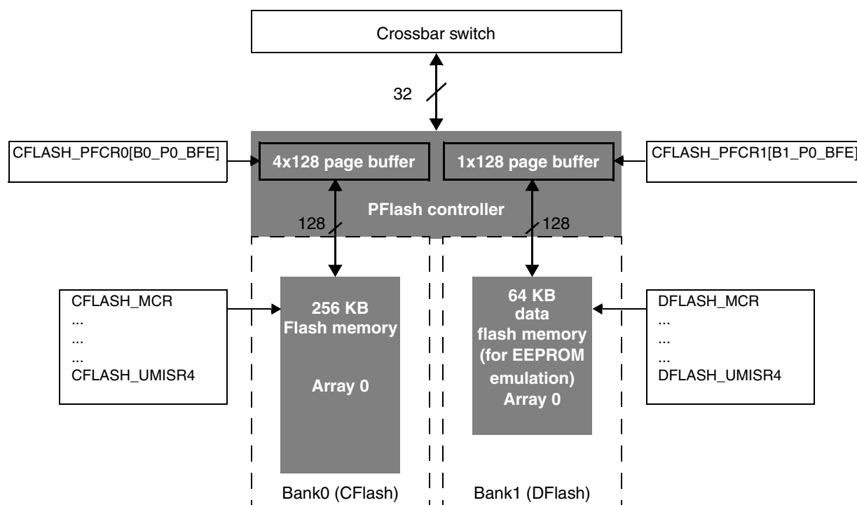
Figure 426. Flash memory architecture
