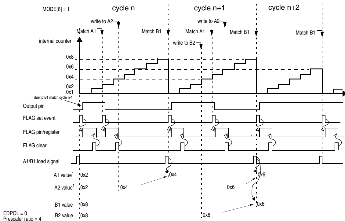
Figure 352. OPWFMB A1 and B1 registers update and flags
