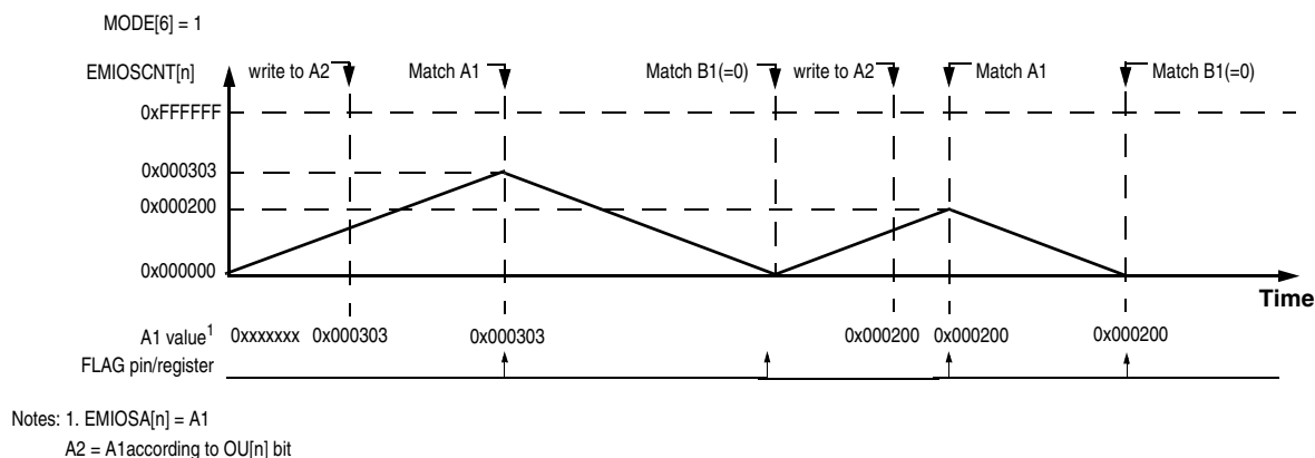
Figure 345. Modulus Counter Up/Down mode example
