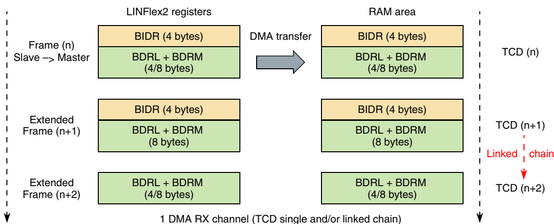
Figure 242. TCD chain memory map (master node, RX mode)
