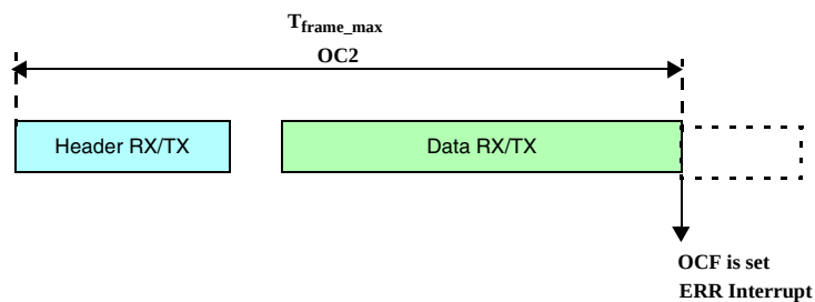
Figure 270. Programming consideration: frame timeout
