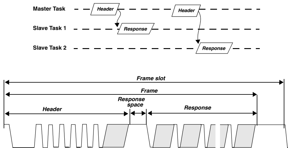
Figure 200. LIN frame structure
