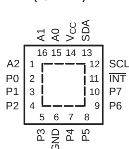
RGT PACKAGE (TOP VIEW)
