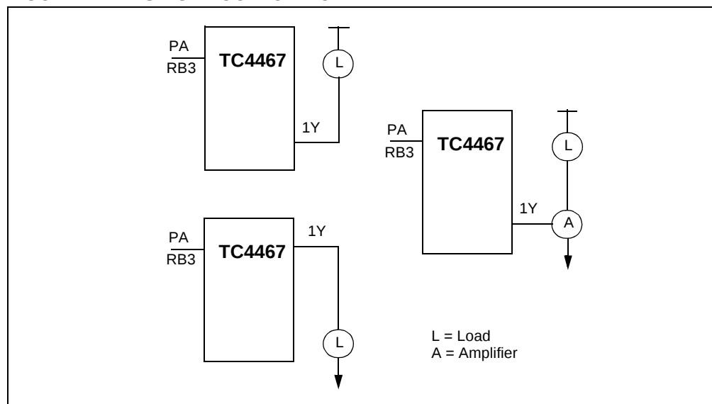
FIGURE A-2: SINGLE OUTPUT MODE PWM
