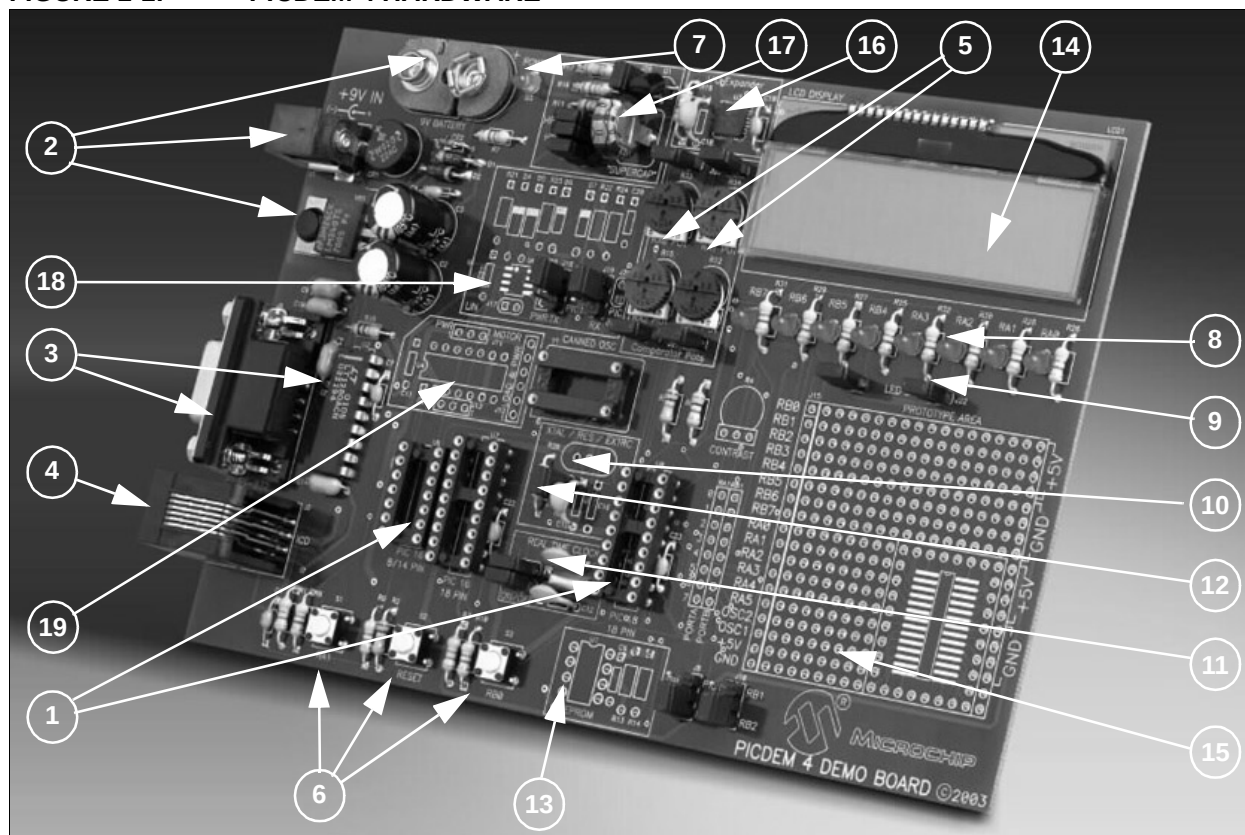
FIGURE 1-1: PICDEM 4 HARDWARE
