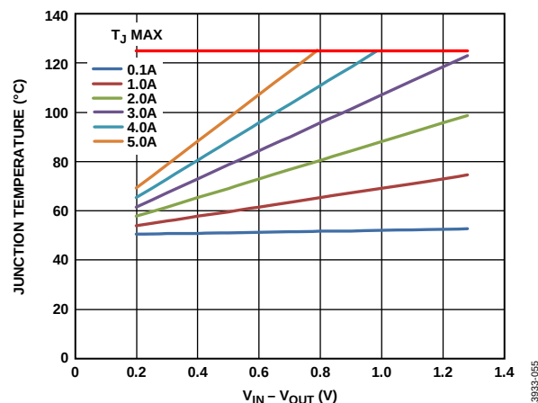
Figure 55. 100 \text{mm}^2 of PCB Copper, T_B = 50^{\circ}\text{C}
