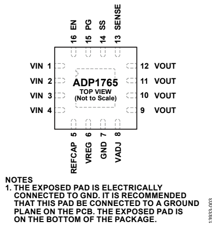
Figure 3. Pin Configuration
