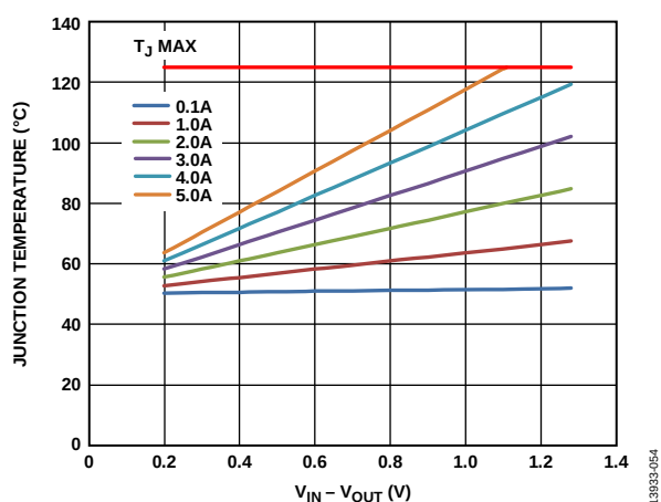
Figure 54. 500 \text{mm}^2 of PCB Copper, T_B = 50^{\circ}\text{C}
