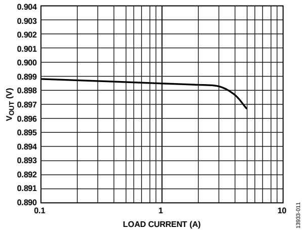
Figure 11. Output Voltage ( V_{OUT} ) vs. Load Current ( I_{LOAD} ), V_{OUT} = 0.9\text{ V}
