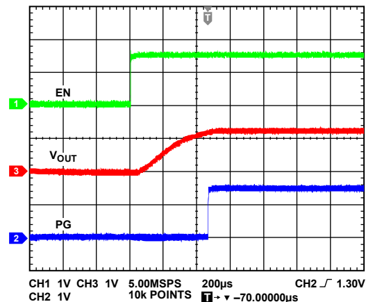
Figure 44. Typical PG Voltage Behavior vs. V_{OUT} , V_{IN} Rising ( V_{OUT} = 1.3 V)
