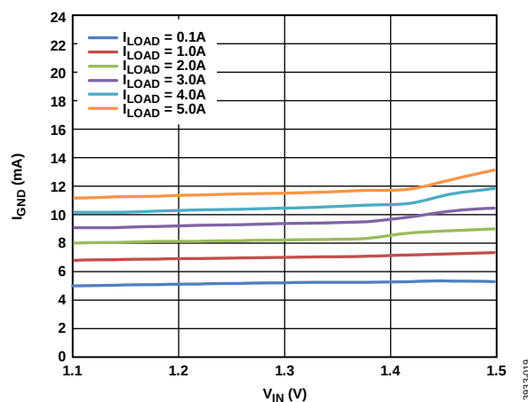
Figure 19. Ground Current ( I_{GND} ) vs. Input Voltage ( V_{IN} ) in Dropout, V_{OUT} = 1.3 V
