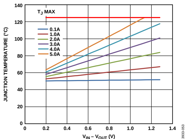
Figure 53. 1000 \text{mm}^2 of PCB Copper, T_B = 50^{\circ}\text{C}
