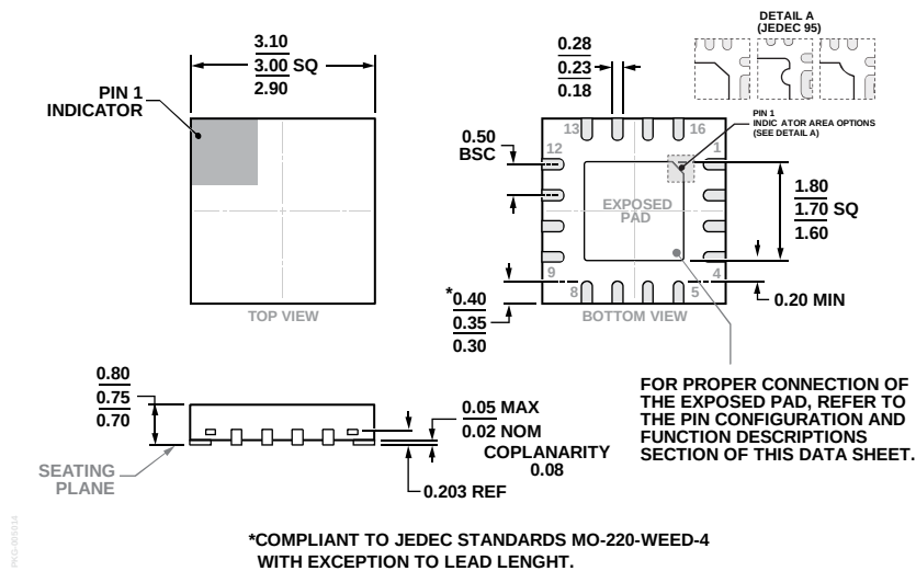
Figure 60. 16-Lead Lead Frame Chip Scale Package [LFCSP] 3 mm × 3 mm Body and 0.75 mm Package Height (CP-16-48) Dimensions shown in millimeters
