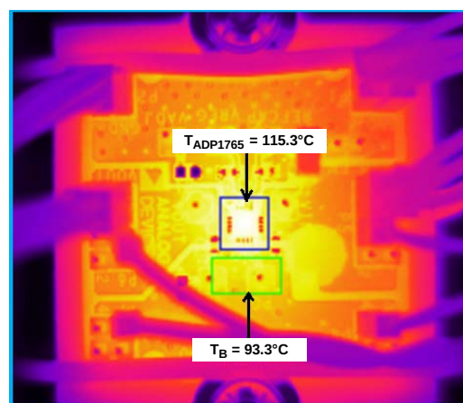
Figure 56. Thermal Image of the ADP1765 Evaluation Board at I_{\text{LOAD}} = 5 \text{ A} , V_{IN} = 1.5 \text{ V} , V_{OUT} = 1.3 \text{ V} , T_B = 93.3^{\circ}\text{C}
