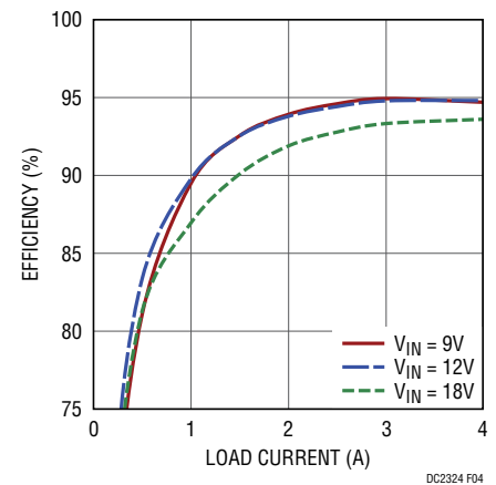
Figure 4. DC2324A-C Efficiency
