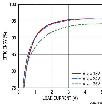
Figure 3. DC2324A-B Efficiency
