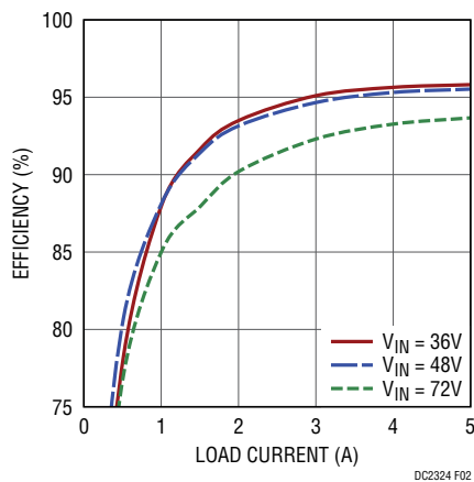
Figure 2. DC2324A-A Efficiency
