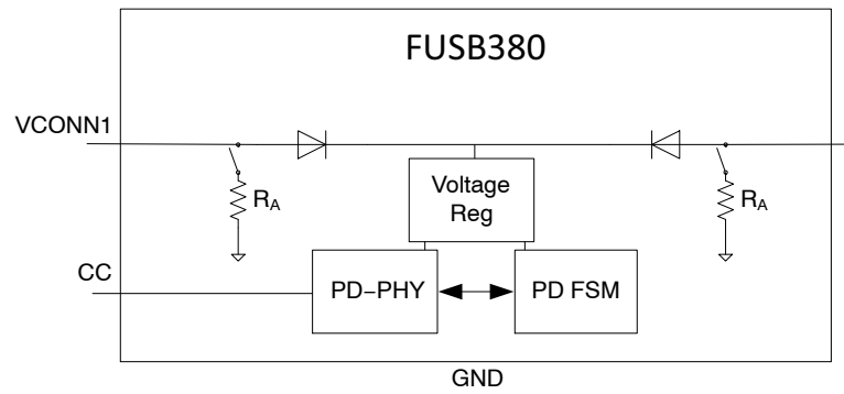
Figure 2. Block Diagram
